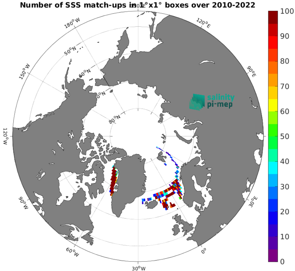
Figure 5: Number of SSS match-ups between TSG (LEGOS-DM) SSS and the CCI SSS L4 POLAR NH Merged-OI v4.41 - 30-day running (ESA) SSS product for the Arctic Ocean Pi-MEP region over 1^\circ \times 1^\circ boxes and for the full satellite product period.
