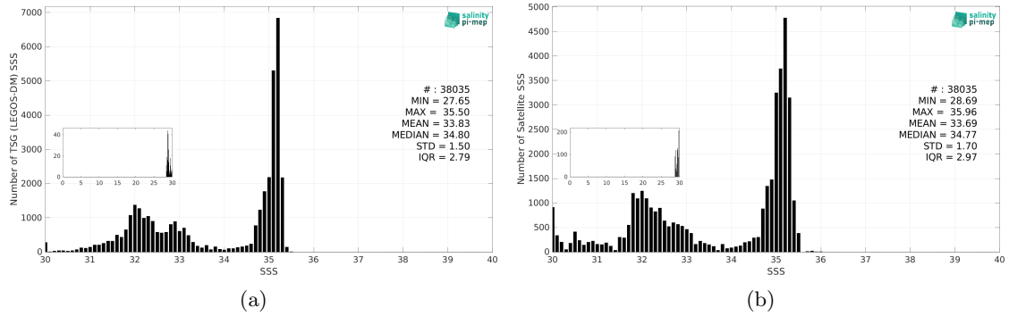
Figure 3: Histograms of SSS from TSG (LEGOS-DM) (a) and CCI SSS L4 POLAR NH Merged-OI v4.41 - 30-day running (ESA) (b) considering all match-up pairs per bins of 0.1 over the Arctic Ocean Pi-MEP region and for the full satellite product period.
