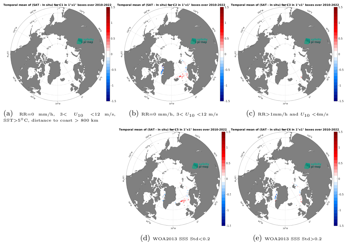
Figure 14: Temporal mean gridded over spatial boxes of size 1^\circ \times 1^\circ of \Delta SSS (CCI SSS L4 POLAR NH Merged-OI v4.41 - 30-day running (ESA) - TSG (LEGOS-DM)) for 5 different subdatasets corresponding to:RR=0 mm/h, 3 < U_{10} < 12 m/s, SST >5^\circ C, distance to coast > 800 km (a), RR=0 mm/h, 3 < U_{10} < 12 m/s (b), RR >1 mm/h and U_{10} < 4 m/s (c), WOA2013 SSS Std <0.2 (d), WOA2013 SSS Std >0.2 (e).
