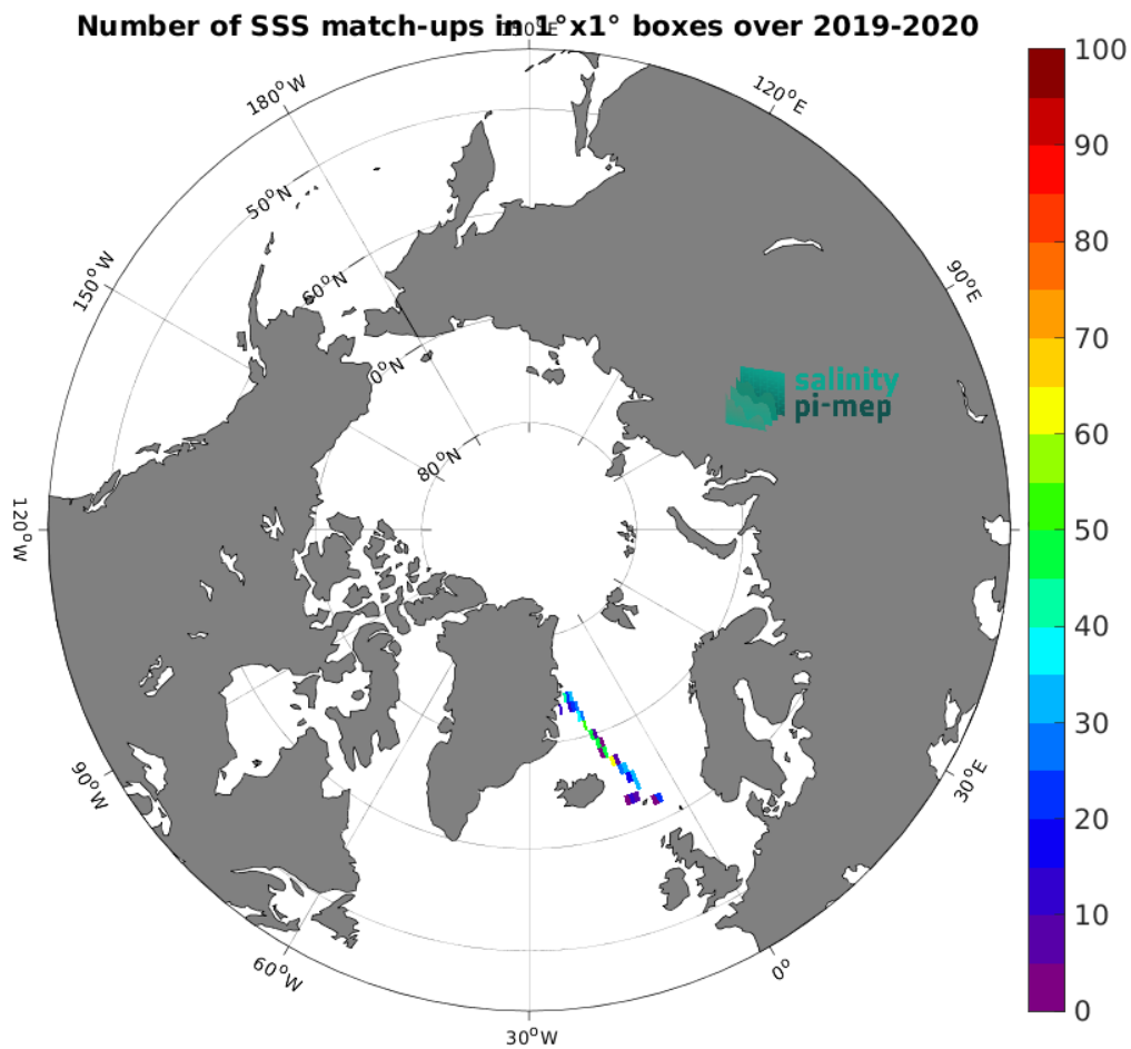
Figure 5: Number of SSS match-ups between TSG (Lauge-Koch) SSS and the CCI SSS L4 POLAR NH Merged-OI v4.41 - 30-day running (ESA) SSS product for the Arctic Ocean Pi-MEP region over 1^{\circ} \times 1^{\circ} boxes and for the full satellite product period.
