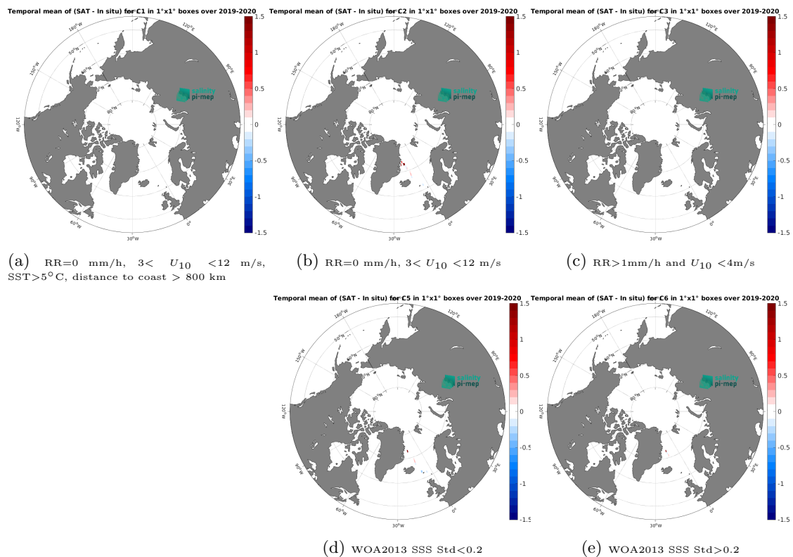
Figure 14: Temporal mean gridded over spatial boxes of size 1^\circ \times 1^\circ of \Delta\text{SSS} (CCI SSS L4 POLAR NH Merged-OI v4.41 - 30-day running (ESA) - TSG (Lauge-Koch)) for 5 different subdatasets corresponding to:RR=0 mm/h, 3 < U_{10} < 12 m/s, SST >5^\circ\text{C} , distance to coast > 800 km (a), RR=0 mm/h, 3 < U_{10} < 12 m/s (b), RR >1 mm/h and U_{10} < 4 m/s (c), WOA2013 SSS Std <0.2 (d), WOA2013 SSS Std >0.2 (e).
