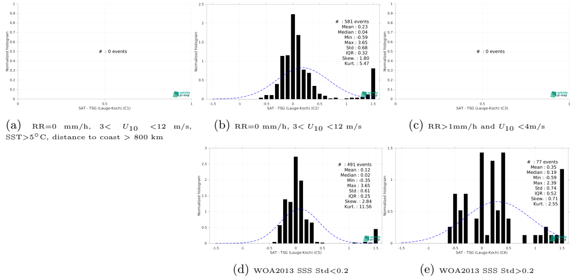
Figure 15: Normalized histogram of \Delta SSS (CCI SSS L4 POLAR NH Merged-OI v4.41 - 30-day running (ESA) - TSG (Lauge-Koch)) for 5 different subdatasets corresponding to: RR=0 mm/h, 3 < U_{10} < 12 m/s, SST > 5°C, distance to coast > 800 km (a), RR=0 mm/h, 3 < U_{10} < 12 m/s (b), RR > 1mm/h and U_{10} < 4 m/s (c), WOA2013 SSS Std < 0.2 (d), WOA2013 SSS Std > 0.2 (e).
