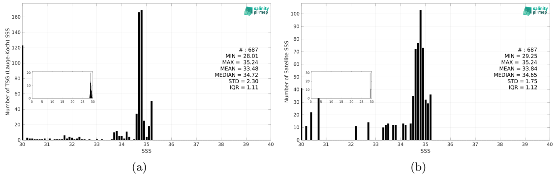
Figure 3: Histograms of SSS from TSG (Lauge-Koch) (a) and CCI SSS L4 POLAR NH Merged-OI v4.41 - 30-day running (ESA) (b) considering all match-up pairs per bins of 0.1 over the Arctic Ocean Pi-MEP region and for the full satellite product period.
