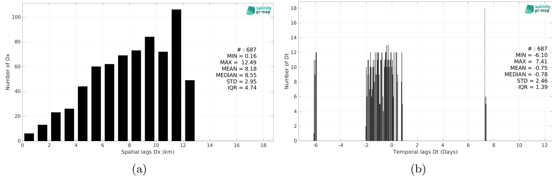
Figure 6: Histograms of the spatial (a) and temporal (b) lags between the location/time of the TSG (Lauge-Koch) measurement and the date of the corresponding CCI SSS L4 POLAR NH Merged-OI v4.41 - 30-day running (ESA) SSS pixel.
