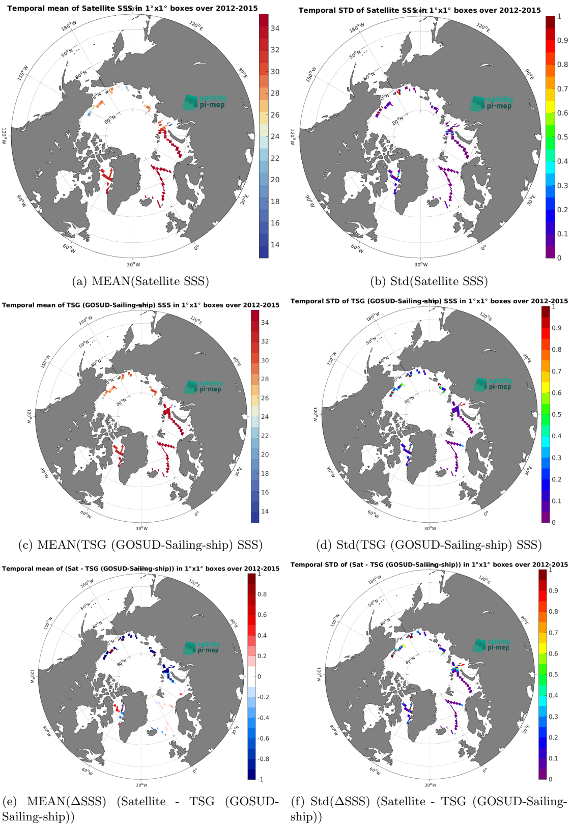
Figure 7: Temporal mean (left) and Std (right) of SSS from CCI SSS L4 POLAR NH Merged-OI v4.41 - 30-day running (ESA) (top), TSG (GOSUD-Sailing-ship) (middle), and of \Delta SSS (Satellite - TSG (GOSUD-Sailing-ship)). Only match-up pairs are used to generate these maps.
