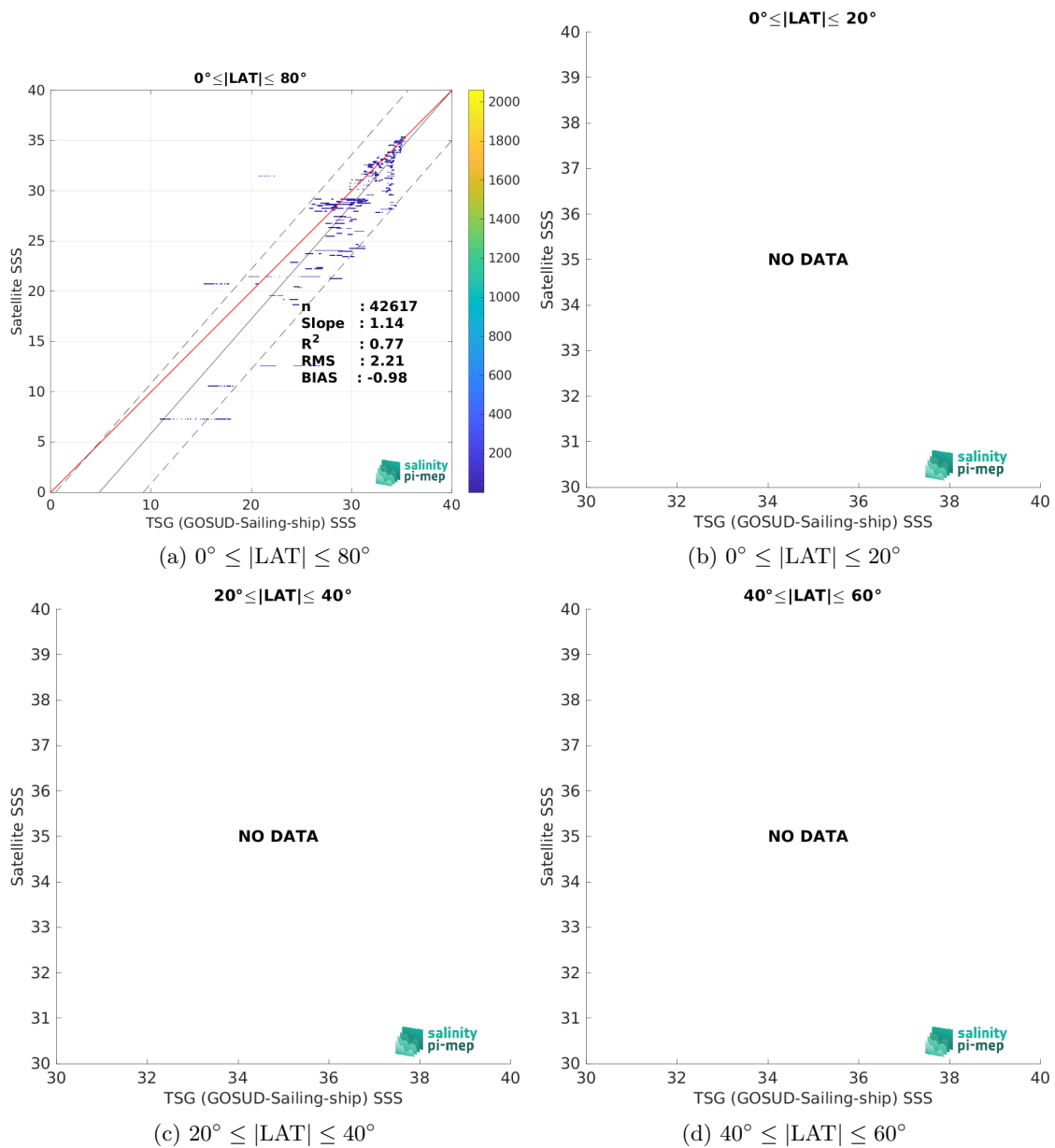
Figure 10: Contour maps of the concentration of CCI SSS L4 POLAR NH Merged-OI v4.41 - 30-day running (ESA) SSS (y-axis) versus TSG (GOSUD-Sailing-ship) SSS (x-axis) at match-up pairs for different latitude bands. For each plot, the red line shows x=y . The black thin and dashed lines indicate a linear fit through the data cloud and the \pm 95\% confidence levels, respectively. The number match-up pairs n , the slope and R^2 coefficient of the linear fit, the root mean square (RMS) and the mean bias between satellite and in situ data are indicated for each latitude band in each plots.
