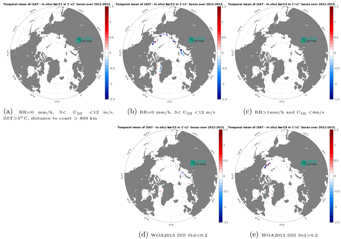
Figure 14: Temporal mean gridded over spatial boxes of size 1^\circ \times 1^\circ of \Delta SSS (CCI SSS L4 POLAR NH Merged-OI v4.41 - 30-day running (ESA) - TSG (GOSUD-Sailing-ship)) for 5 different subdatasets corresponding to:RR=0 mm/h, 3 < U_{10} < 12 m/s, SST >5^\circ\text{C} , distance to coast > 800 km (a), RR=0 mm/h, 3 < U_{10} < 12 m/s (b), RR >1 mm/h and U_{10} < 4 m/s (c), WOA2013 SSS Std <0.2 (d), WOA2013 SSS Std >0.2 (e).
