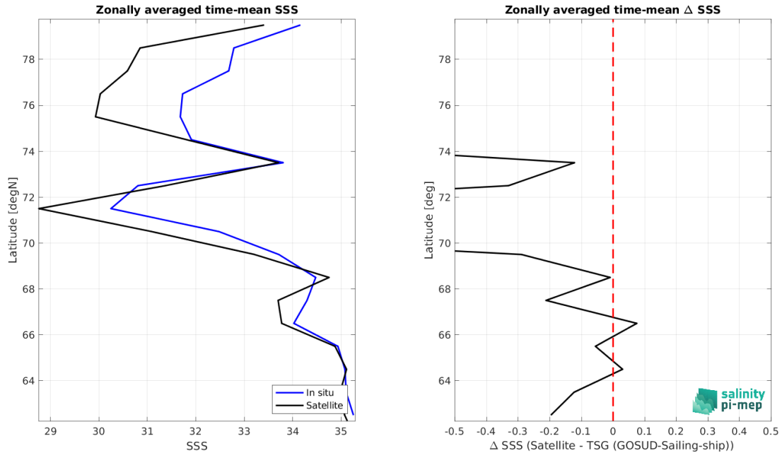
Figure 9: Left panel: Zonal mean SSS from CCI SSS L4 POLAR NH Merged-OI v4.41 - 30-day running (ESA) satellite product (black) and from TSG (GOSUD-Sailing-ship) (blue). Right panel: Zonal mean of \Delta SSS (Satellite - TSG (GOSUD-Sailing-ship)) for all the collected Pi-MEP match-up pairs estimated over the full satellite product period.
