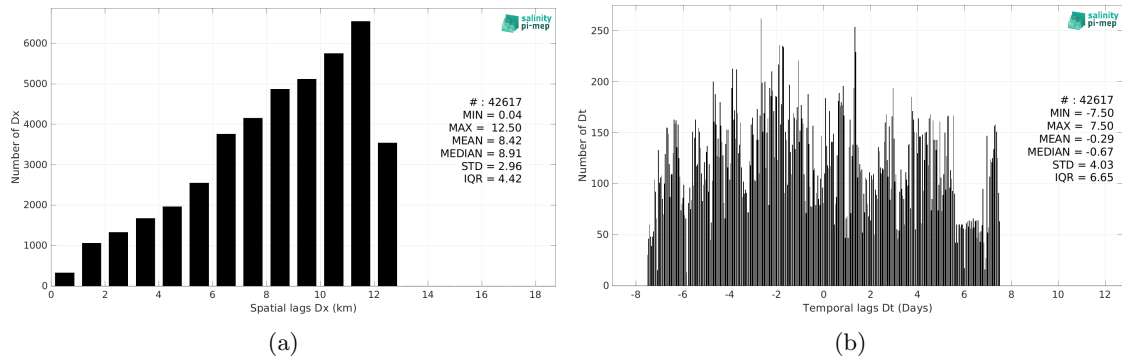
Figure 6: Histograms of the spatial (a) and temporal (b) lags between the location/time of the TSG (GOSUD-Sailing-ship) measurement and the date of the corresponding CCI SSS L4 POLAR NH Merged-OI v4.41 - 30-day running (ESA) SSS pixel.
