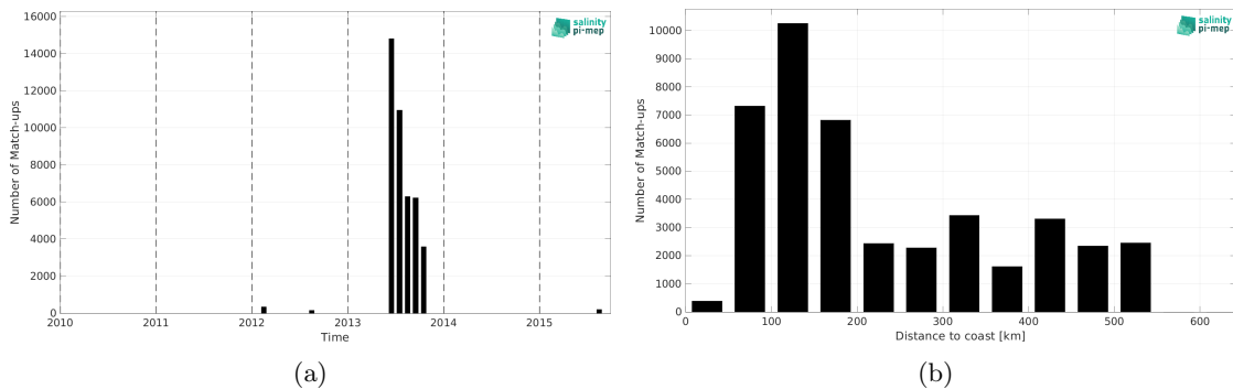
Figure 2: Number of match-ups between TSG (GOSUD-Sailing-ship) and CCI SSS L4 POLAR NH Merged-OI v4.41 - 30-day running (ESA) SSS as a function of time (a) and as function of the distance to coast (b) over the Arctic Ocean Pi-MEP region and for the full satellite product period.
