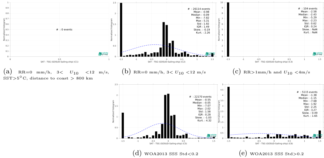
Figure 15: Normalized histogram of \Delta SSS (CCI SSS L4 POLAR NH Merged-OI v4.41 - 30-day running (ESA) - TSG (GOSUD-Sailing-ship)) for 5 different subdatasets corresponding to: RR=0 mm/h, 3 < U_{10} < 12 m/s, SST > 5°C, distance to coast > 800 km (a), RR=0 mm/h, 3 < U_{10} < 12 m/s (b), RR > 1mm/h and U_{10} < 4 m/s (c), WOA2013 SSS Std < 0.2 (d), WOA2013 SSS Std > 0.2 (e).
