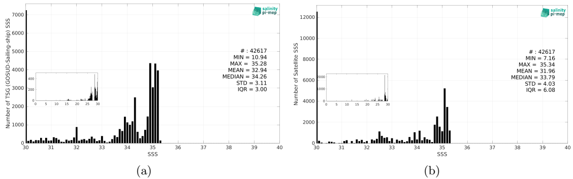
Figure 3: Histograms of SSS from TSG (GOSUD-Sailing-ship) (a) and CCI SSS L4 POLAR NH Merged-OI v4.41 - 30-day running (ESA) (b) considering all match-up pairs per bins of 0.1 over the Arctic Ocean Pi-MEP region and for the full satellite product period.
