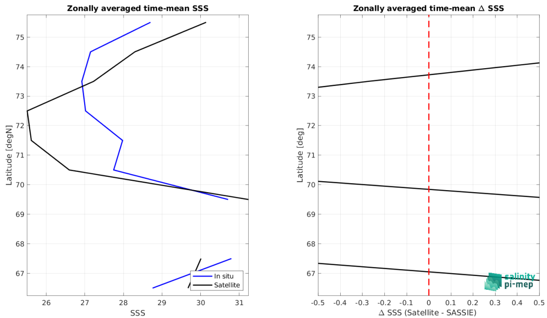
Figure 9: Left panel: Zonal mean SSS from CCI SSS L4 POLAR NH Merged-OI v4.41 - 30-day running (ESA) satellite product (black) and from SASSIE (blue). Right panel: Zonal mean of \Delta SSS (Satellite - SASSIE) for all the collected Pi-MEP match-up pairs estimated over the full satellite product period.
