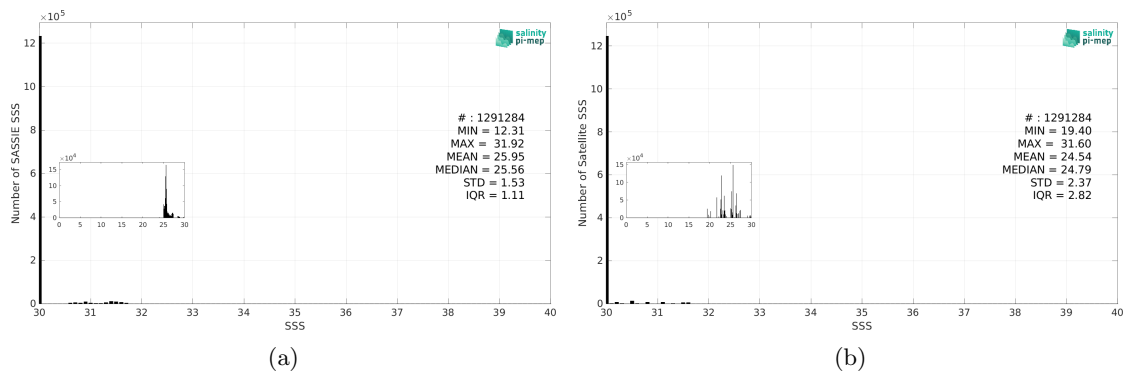
Figure 3: Histograms of SSS from SASSIE (a) and CCI SSS L4 POLAR NH Merged-OI v4.41 - 30-day running (ESA) (b) considering all match-up pairs per bins of 0.1 over the Arctic Ocean Pi-MEP region and for the full satellite product period.
