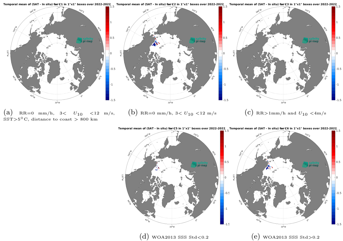
Figure 14: Temporal mean gridded over spatial boxes of size 1^\circ \times 1^\circ of \Delta SSS (CCI SSS L4 POLAR NH Merged-OI v4.41 - 30-day running (ESA) - SASSIE) for 5 different subdatasets corresponding to:RR=0 mm/h, 3 < U_{10} < 12 m/s, SST >5^\circ C, distance to coast > 800 km (a), RR=0 mm/h, 3 < U_{10} < 12 m/s (b), RR >1 mm/h and U_{10} < 4 m/s (c), WOA2013 SSS Std <0.2 (d), WOA2013 SSS Std >0.2 (e).
