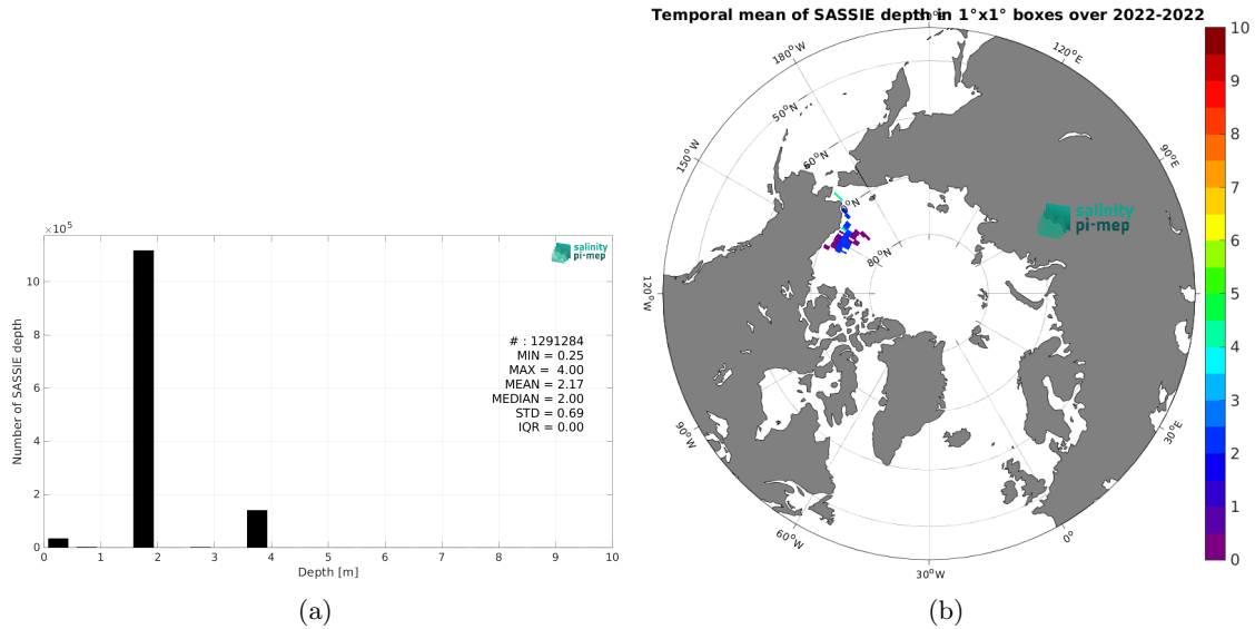
Figure 4: Histograms of the depth of the upper level SSS measurements from SASSIE in the Match-up DataBase for the Arctic Ocean Pi-MEP region (a) and temporal mean spatial distribution of pressure of the in situ SSS data over 1^\circ \times 1^\circ boxes and for the full satellite product period (b).
