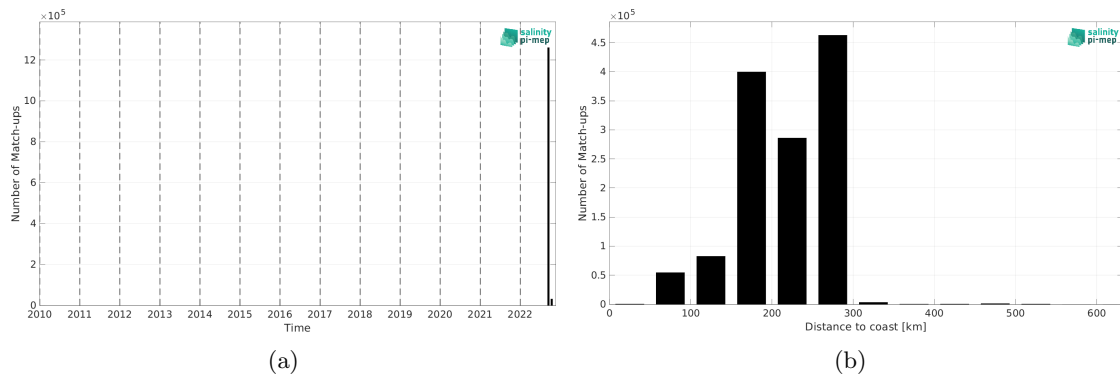
Figure 2: Number of match-ups between SASSIE and CCI SSS L4 POLAR NH Merged-OI v4.41 - 30-day running (ESA) SSS as a function of time (a) and as function of the distance to coast (b) over the Arctic Ocean Pi-MEP region and for the full satellite product period.
