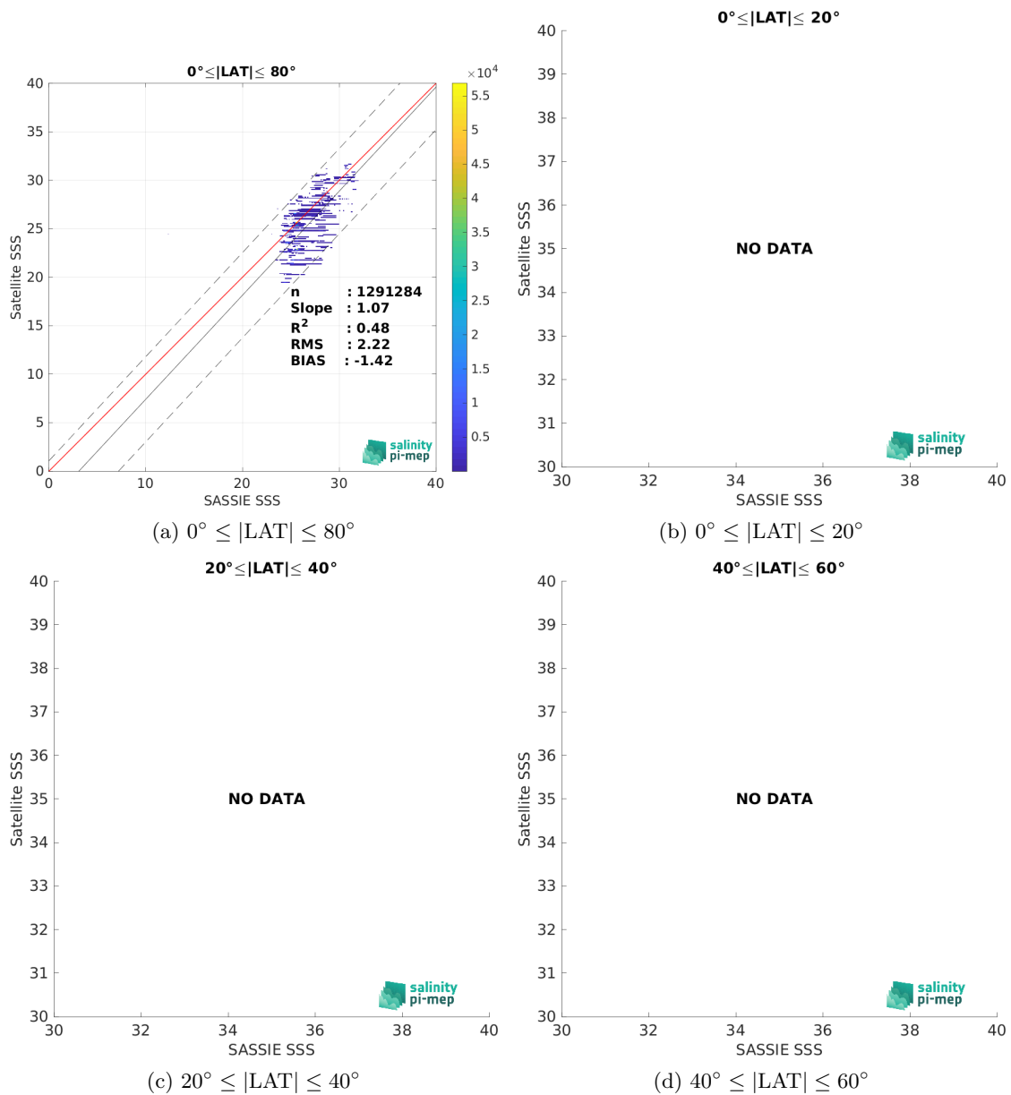
Figure 10: Contour maps of the concentration of CCI SSS L4 POLAR NH Merged-OI v4.41 - 30-day running (ESA) SSS (y-axis) versus SASSIE SSS (x-axis) at match-up pairs for different latitude bands. For each plot, the red line shows x=y . The black thin and dashed lines indicate a linear fit through the data cloud and the \pm 95\% confidence levels, respectively. The number match-up pairs n , the slope and R^2 coefficient of the linear fit, the root mean square (RMS) and the mean bias between satellite and in situ data are indicated for each latitude band in each plots.
