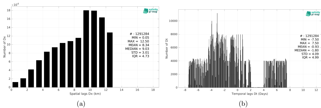
Figure 6: Histograms of the spatial (a) and temporal (b) lags between the location/time of the SASSIE measurement and the date of the corresponding CCI SSS L4 POLAR NH Merged-OI v4.41 - 30-day running (ESA) SSS pixel.
