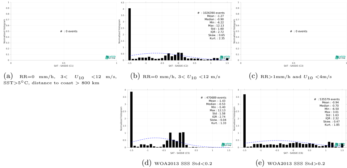
Figure 15: Normalized histogram of \Delta SSS (CCI SSS L4 POLAR NH Merged-OI v4.41 - 30-day running (ESA) - SASSIE) for 5 different subdatasets corresponding to: RR=0 mm/h, 3 < U_{10} < 12 m/s, SST > 5°C, distance to coast > 800 km (a), RR=0 mm/h, 3 < U_{10} < 12 m/s (b), RR > 1mm/h and U_{10} < 4 m/s (c), WOA2013 SSS Std < 0.2 (d), WOA2013 SSS Std > 0.2 (e).
