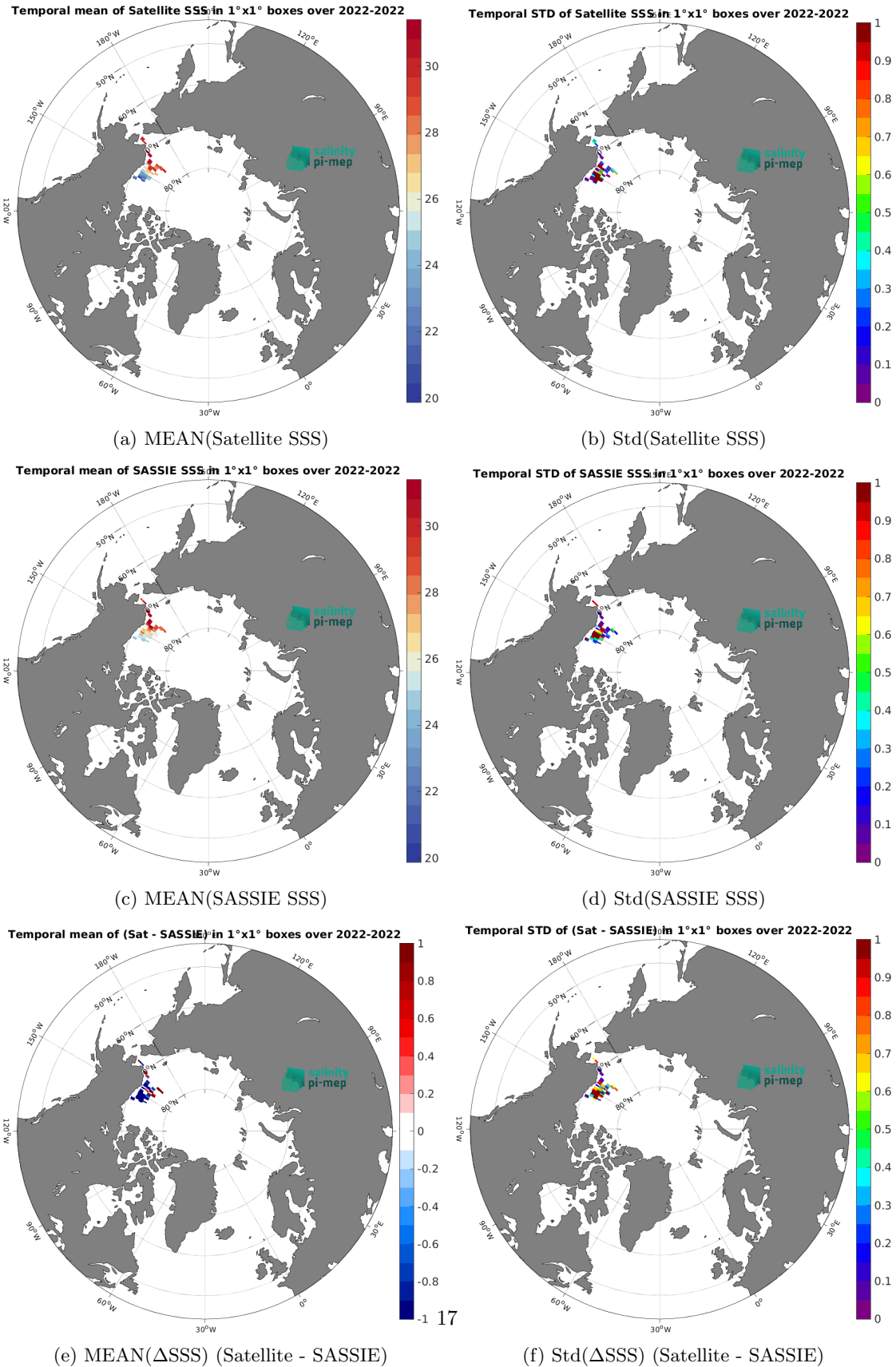
Figure 7: Temporal mean (left) and Std (right) of SSS from CCI SSS L4 POLAR NH Merged-OI v4.41 - 30-day running (ESA) (top), SASSIE (middle), and of \Delta SSS (Satellite - SASSIE). Only match-up pairs are used to generate these maps.
