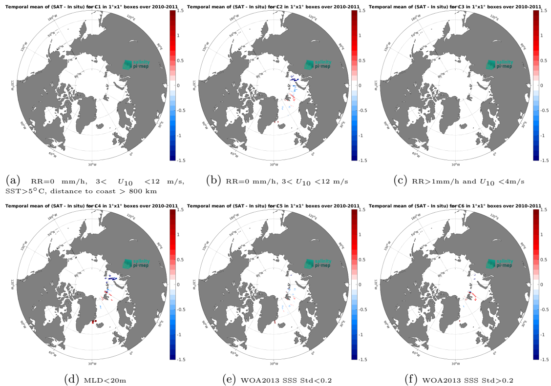
Figure 14: Temporal mean gridded over spatial boxes of size 1^\circ \times 1^\circ of \Delta\text{SSS} (CCI SSS L4 POLAR NH Merged-OI v4.41 - 30-day running (ESA) - Marine mammals) for 6 different subdatasets corresponding to:RR=0 mm/h, 3 < U_{10} < 12 m/s, SST>5°C, distance to coast > 800 km (a), RR=0 mm/h, 3 < U_{10} < 12 m/s (b), RR>1mm/h and U_{10} < 4 m/s (c),MLD<20m (d),WOA2013 SSS Std<0.2 (e),WOA2013 SSS Std>0.2 (f).
