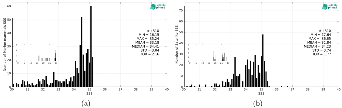
Figure 3: Histograms of SSS from Marine mammals (a) and CCI SSS L4 POLAR NH Merged-OI v4.41 - 30-day running (ESA) (b) considering all match-up pairs per bins of 0.1 over the Arctic Ocean Pi-MEP region and for the full satellite product period.
