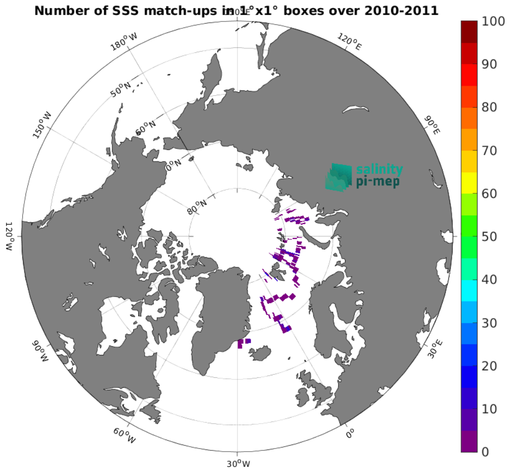
Figure 5: Number of SSS match-ups between Marine mammals SSS and the CCI SSS L4 POLAR NH Merged-OI v4.41 - 30-day running (ESA) SSS product for the Arctic Ocean Pi-MEP region over 1^{\circ} \times 1^{\circ} boxes and for the full satellite product period.
