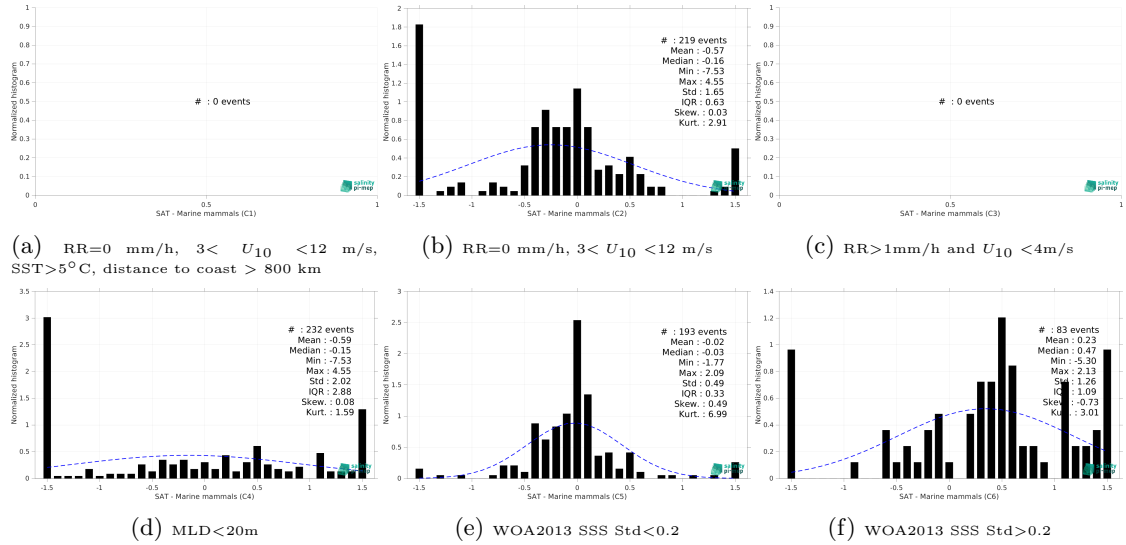
Figure 15: Normalized histogram of \Delta SSS (CCI SSS L4 POLAR NH Merged-OI v4.41 - 30-day running (ESA) - Marine mammals) for 6 different subdatasets corresponding to: RR=0 mm/h, 3 < U_{10} < 12 m/s, SST>5°C, distance to coast > 800 km (a), RR=0 mm/h, 3 < U_{10} < 12 m/s (b), RR>1mm/h and U_{10} < 4 m/s (c), MLD<20m (d), WOA2013 SSS Std<0.2 (e), WOA2013 SSS Std>0.2 (f).
