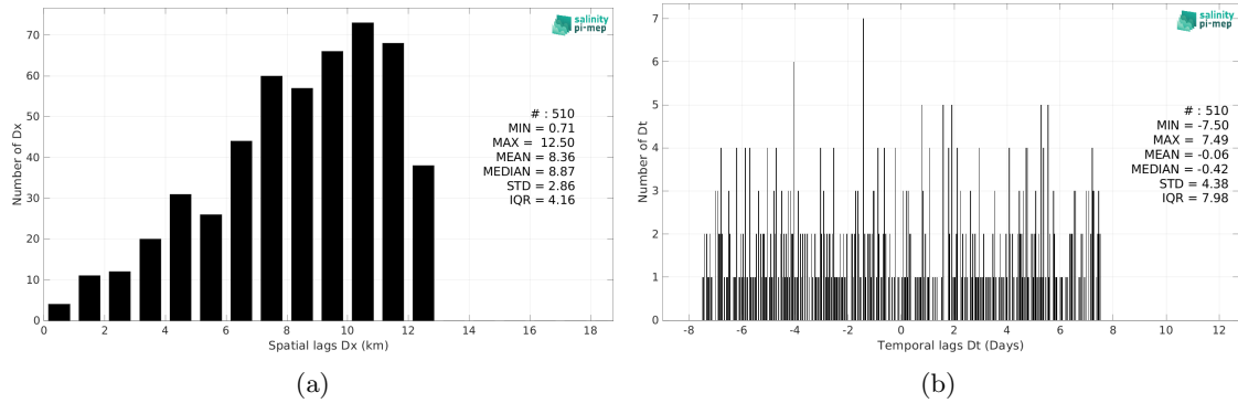
Figure 6: Histograms of the spatial (a) and temporal (b) lags between the location/time of the Marine mammals measurement and the date of the corresponding CCI SSS L4 POLAR NH Merged-OI v4.41 - 30-day running (ESA) SSS pixel.
