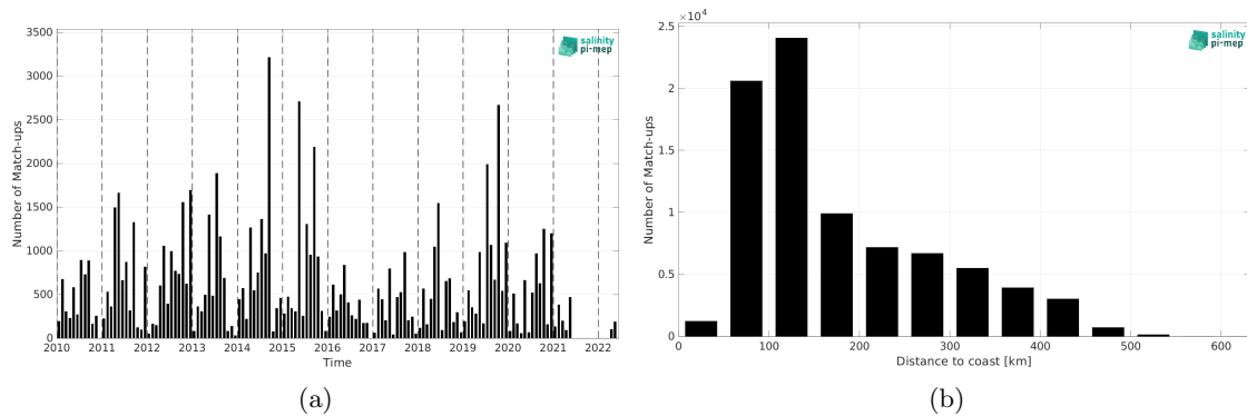
Figure 2: Number of match-ups between ICES and CCI SSS L4 POLAR NH Merged-OI v4.41 - 30-day running (ESA) SSS as a function of time (a) and as function of the distance to coast (b) over the Arctic Ocean Pi-MEP region and for the full satellite product period.
