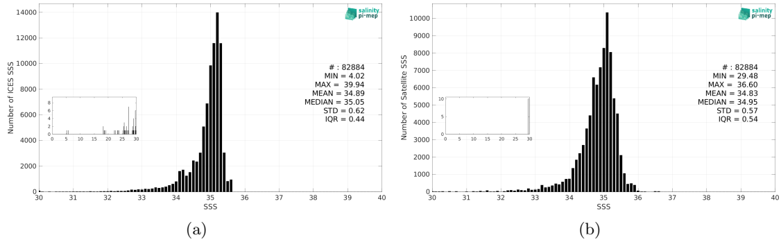
Figure 3: Histograms of SSS from ICES (a) and CCI SSS L4 POLAR NH Merged-OI v4.41 - 30-day running (ESA) (b) considering all match-up pairs per bins of 0.1 over the Arctic Ocean Pi-MEP region and for the full satellite product period.
