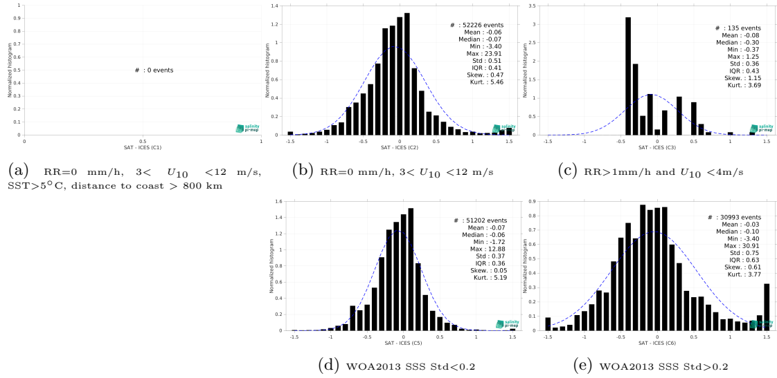
Figure 15: Normalized histogram of \Delta SSS (CCI SSS L4 POLAR NH Merged-OI v4.41 - 30-day running (ESA) - ICES) for 5 different subdatasets corresponding to: RR=0 mm/h, 3 < U_{10} < 12 m/s, SST>5°C, distance to coast > 800 km (a), RR=0 mm/h, 3 < U_{10} < 12 m/s (b), RR>1mm/h and U_{10} < 4 m/s (c), WOA2013 SSS Std<0.2 (d), WOA2013 SSS Std>0.2 (e).
