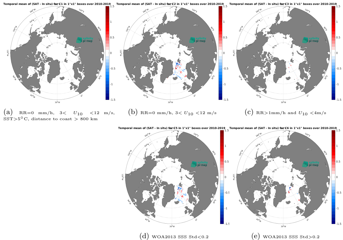
Figure 13: Temporal mean gridded over spatial boxes of size 1^\circ \times 1^\circ of \Delta SSS (CCI SSS L4 POLAR NH Merged-OI v4.41 - 30-day running (ESA) - Surface drifters) for 5 different subdatasets corresponding to:RR=0 mm/h, 3 < U_{10} < 12 m/s, SST >5^\circ C, distance to coast > 800 km (a), RR=0 mm/h, 3 < U_{10} < 12 m/s (b), RR >1 mm/h and U_{10} < 4 m/s (c), WOA2013 SSS Std <0.2 (d), WOA2013 SSS Std >0.2 (e).
