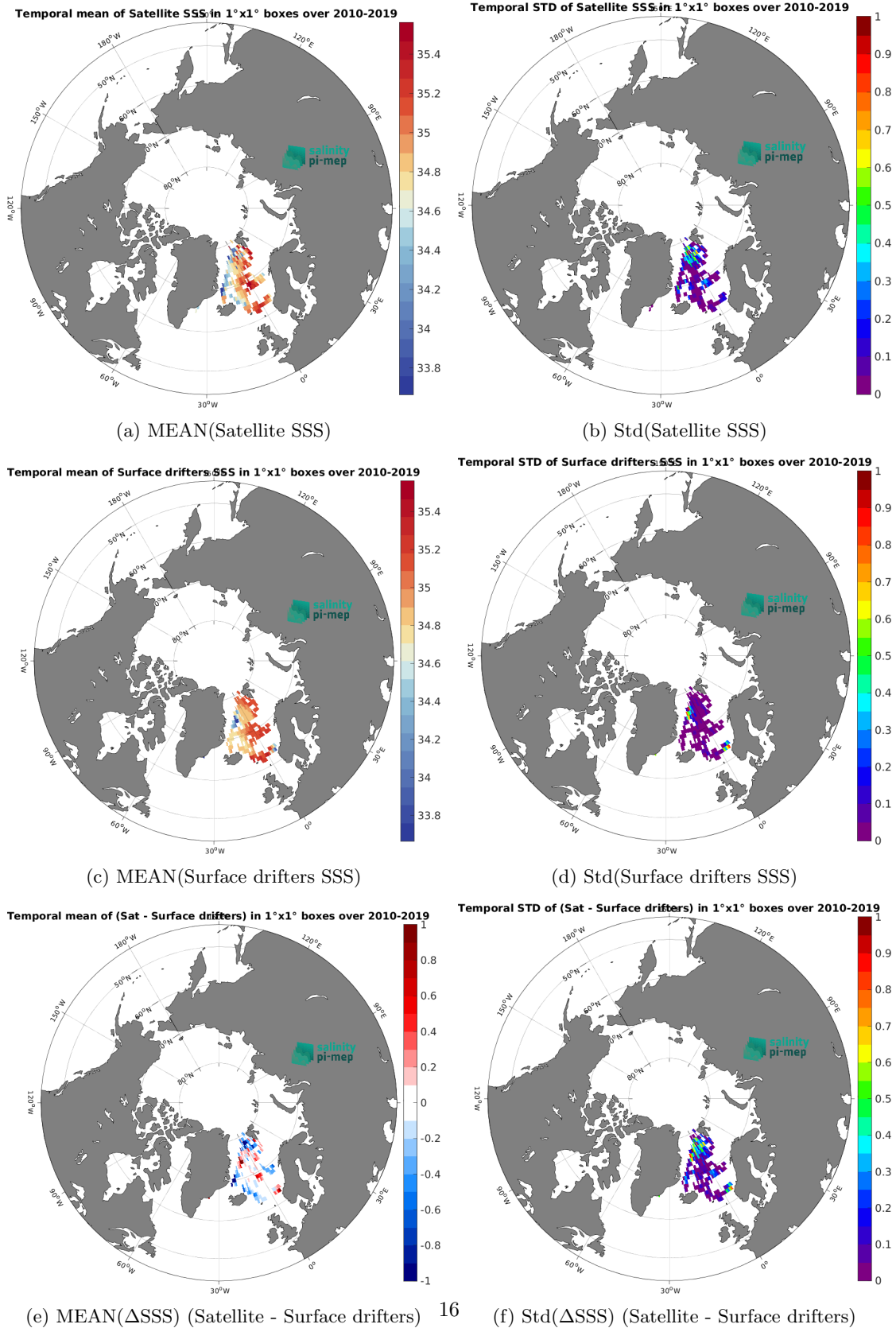
Figure 6: Temporal mean (left) and Std (right) of SSS from CCI SSS L4 POLAR NH Merged-OI v4.41 - 30-day running (ESA) (top), Surface drifters (middle), and of \Delta SSS (Satellite - Surface drifters). Only match-up pairs are used to generate these maps.
