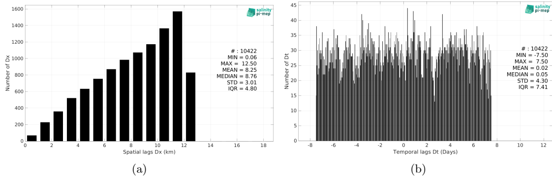
Figure 5: Histograms of the spatial (a) and temporal (b) lags between the location/time of the Surface drifters measurement and the date of the corresponding CCI SSS L4 POLAR NH Merged-OI v4.41 - 30-day running (ESA) SSS pixel.
