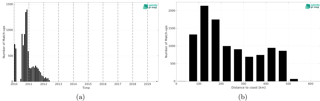
Figure 2: Number of match-ups between Surface drifters and CCI SSS L4 POLAR NH Merged-OI v4.41 - 30-day running (ESA) SSS as a function of time (a) and as function of the distance to coast (b) over the Arctic Ocean Pi-MEP region and for the full satellite product period.
