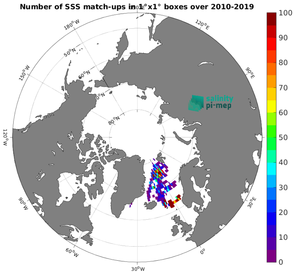
Figure 4: Number of SSS match-ups between Surface drifters SSS and the CCI SSS L4 POLAR NH Merged-OI v4.41 - 30-day running (ESA) SSS product for the Arctic Ocean Pi-MEP region over 1^{\circ} \times 1^{\circ} boxes and for the full satellite product period.
