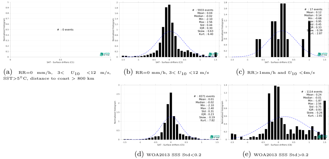
Figure 14: Normalized histogram of \Delta SSS (CCI SSS L4 POLAR NH Merged-OI v4.41 - 30-day running (ESA) - Surface drifters) for 5 different subdatasets corresponding to: RR=0 mm/h, 3 < U_{10} < 12 m/s, SST > 5°C, distance to coast > 800 km (a), RR=0 mm/h, 3 < U_{10} < 12 m/s (b), RR > 1mm/h and U_{10} < 4 m/s (c), WOA2013 SSS Std < 0.2 (d), WOA2013 SSS Std > 0.2 (e).
