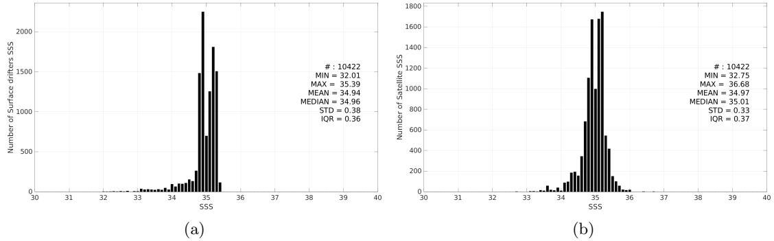
Figure 3: Histograms of SSS from Surface drifters (a) and CCI SSS L4 POLAR NH Merged-OI v4.41 - 30-day running (ESA) (b) considering all match-up pairs per bins of 0.1 over the Arctic Ocean Pi-MEP region and for the full satellite product period.
