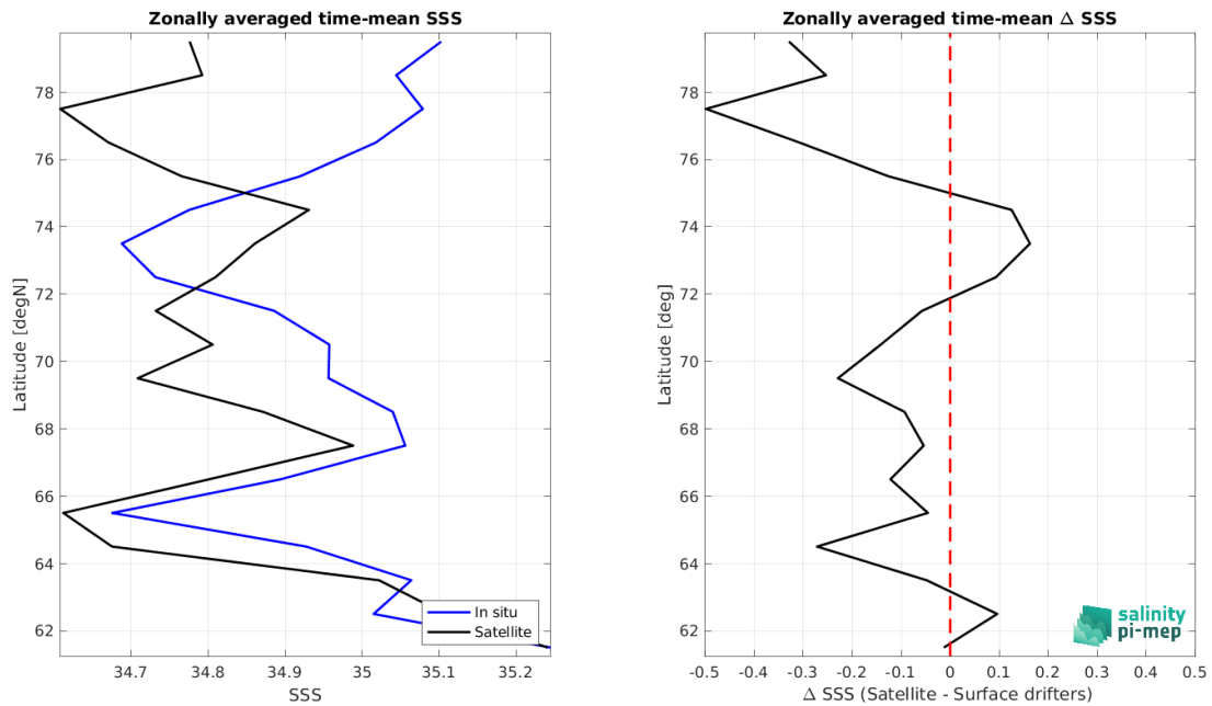
Figure 8: Left panel: Zonal mean SSS from CCI SSS L4 POLAR NH Merged-OI v4.41 - 30-day running (ESA) satellite product (black) and from Surface drifters (blue). Right panel: Zonal mean of \Delta SSS (Satellite - Surface drifters) for all the collected Pi-MEP match-up pairs estimated over the full satellite product period.
