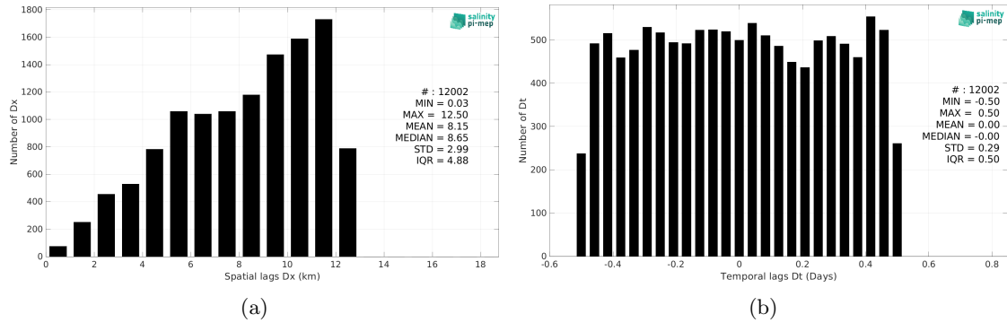
Figure 5: Histograms of the spatial (a) and temporal (b) lags between the location/time of the TSG (SAMOS) measurement and the date of the corresponding CCI SSS L4 POLAR NH Merged-OI v4.4 - 7-day running (ESA) SSS pixel.
