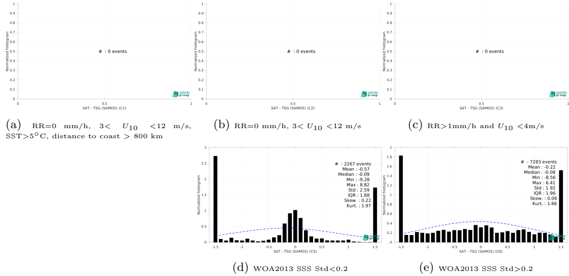
Figure 13: Normalized histogram of \Delta SSS (CCI SSS L4 POLAR NH Merged-OI v4.4 - 7-day running (ESA) - TSG (SAMOS)) for 5 different subdatasets corresponding to: RR=0 mm/h, 3 < U_{10} < 12 m/s, SST>5°C, distance to coast > 800 km (a), RR=0 mm/h, 3 < U_{10} < 12 m/s (b), RR>1mm/h and U_{10} < 4 m/s (c), WOA2013 SSS Std<0.2 (d), WOA2013 SSS Std>0.2 (e).
