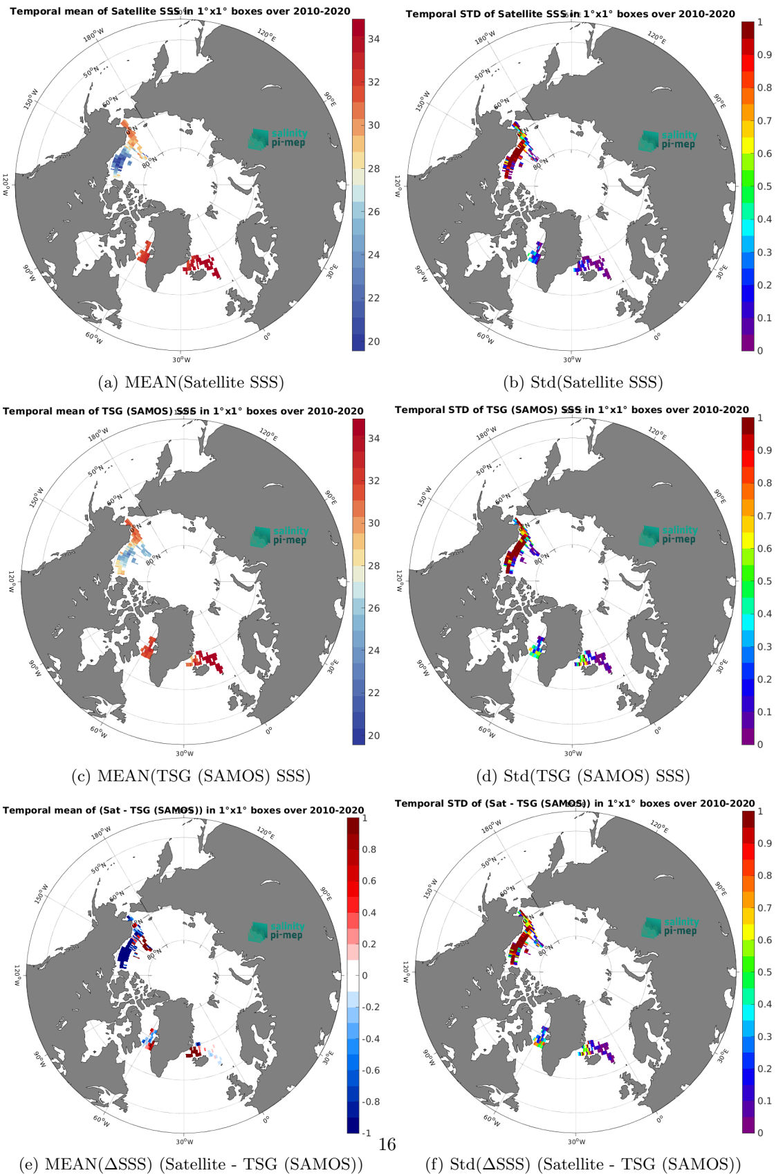
Figure 6: Temporal mean (left) and Std (right) of SSS from CCI SSS L4 POLAR NH Merged-OI v4.4 - 7-day running (ESA) (top), TSG (SAMOS) (middle), and of \Delta SSS (Satellite - TSG (SAMOS)). Only match-up pairs are used to generate these maps.
