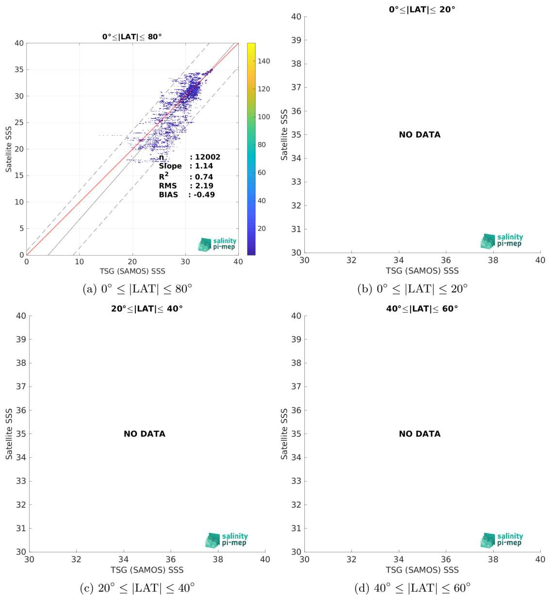
Figure 9: Contour maps of the concentration of CCI SSS L4 POLAR NH Merged-OI v4.4 - 7-day running (ESA) SSS (y-axis) versus TSG (SAMOS) SSS (x-axis) at match-up pairs for different latitude bands. For each plot, the red line shows x=y . The black thin and dashed lines indicate a linear fit through the data cloud and the \pm 95\% confidence levels, respectively. The number match-up pairs n , the slope and R^2 coefficient of the linear fit, the root mean square (RMS) and the mean bias between satellite and in situ data are indicated for each latitude band in each plots.
