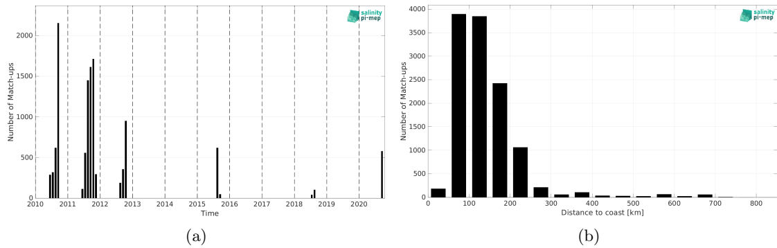
Figure 1: Number of match-ups between TSG (SAMOS) and CCI SSS L4 POLAR NH Merged-OI v4.4 - 7-day running (ESA) SSS as a function of time (a) and as function of the distance to coast (b) over the Arctic Ocean Pi-MEP region and for the full satellite product period.
