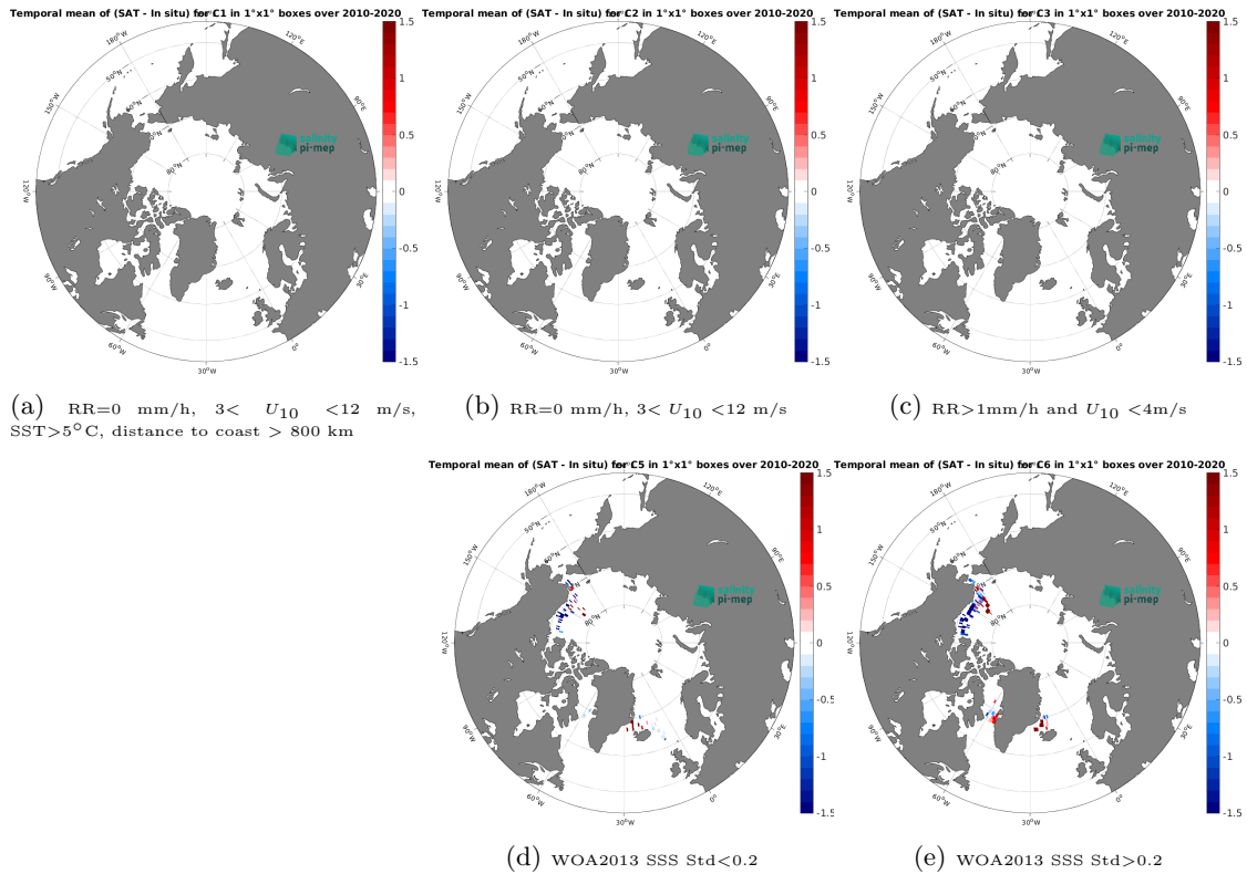
Figure 12: Temporal mean gridded over spatial boxes of size 1^{\circ}\times 1^{\circ} of \Delta\text{SSS} (CCI SSS L4 POLAR NH Merged-OI v4.4 - 7-day running (ESA) - TSG (SAMOS)) for 5 different subdatasets corresponding to:RR=0 mm/h, 3 < U_{10} < 12 m/s, SST >5^{\circ}\text{C} , distance to coast > 800 km (a), RR=0 mm/h, 3 < U_{10} < 12 m/s (b), RR >1 mm/h and U_{10} < 4 m/s (c), WOA2013 SSS Std <0.2 (d), WOA2013 SSS Std >0.2 (e).
