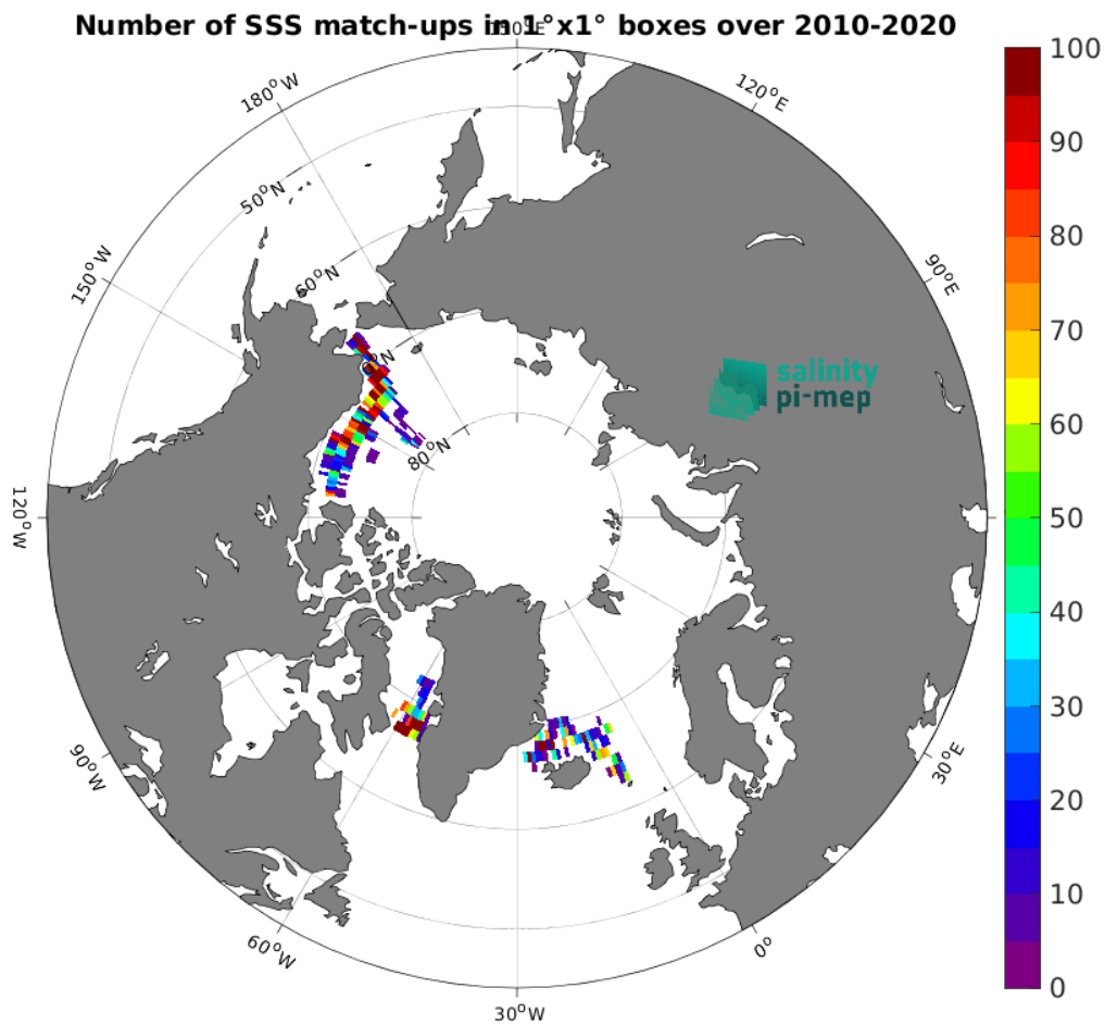
Figure 4: Number of SSS match-ups between TSG (SAMOS) SSS and the CCI SSS L4 POLAR NH Merged-OI v4.4 - 7-day running (ESA) SSS product for the Arctic Ocean Pi-MEP region over 1^{\circ} \times 1^{\circ} boxes and for the full satellite product period.
