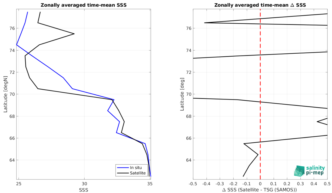
Figure 8: Left panel: Zonal mean SSS from CCI SSS L4 POLAR NH Merged-OI v4.4 - 7-day running (ESA) satellite product (black) and from TSG (SAMOS) (blue). Right panel: Zonal mean of \Delta SSS (Satellite - TSG (SAMOS)) for all the collected Pi-MEP match-up pairs estimated over the full satellite product period.
