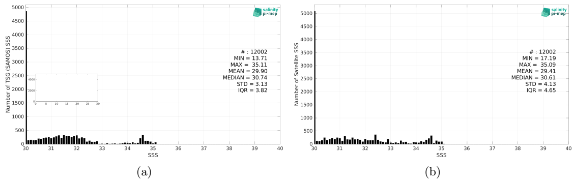
Figure 2: Histograms of SSS from TSG (SAMOS) (a) and CCI SSS L4 POLAR NH Merged-OI v4.4 - 7-day running (ESA) (b) considering all match-up pairs per bins of 0.1 over the Arctic Ocean Pi-MEP region and for the full satellite product period.
