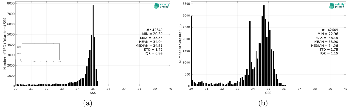
Figure 2: Histograms of SSS from TSG (Polarstern) (a) and CCI SSS L4 POLAR NH Merged-OI v4.4 - 7-day running (ESA) (b) considering all match-up pairs per bins of 0.1 over the Arctic Ocean Pi-MEP region and for the full satellite product period.
