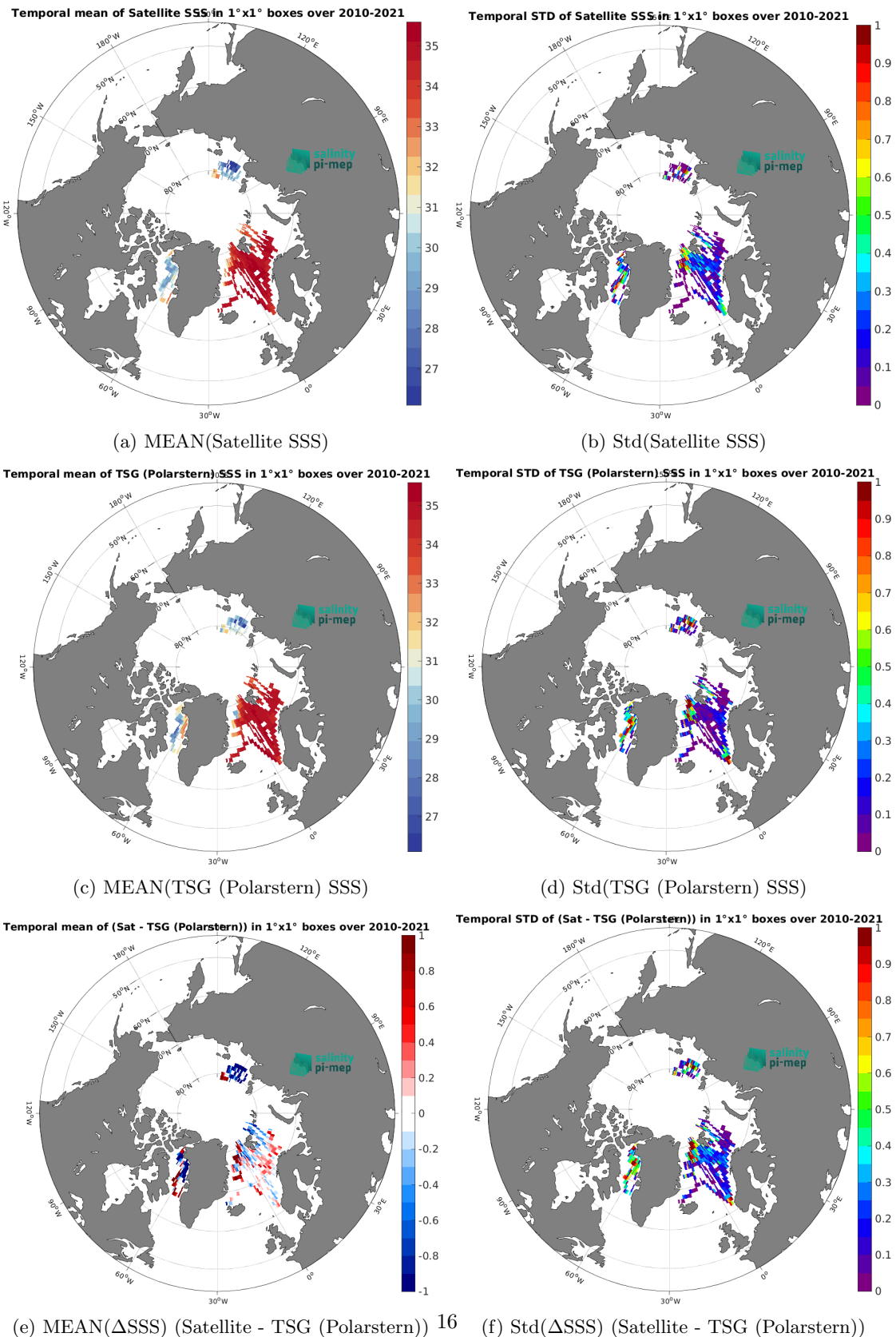
Figure 6: Temporal mean (left) and Std (right) of SSS from CCI SSS L4 POLAR NH Merged-OI v4.4 - 7-day running (ESA) (top), TSG (Polarstern) (middle), and of \Delta SSS (Satellite - TSG (Polarstern)). Only match-up pairs are used to generate these maps.
