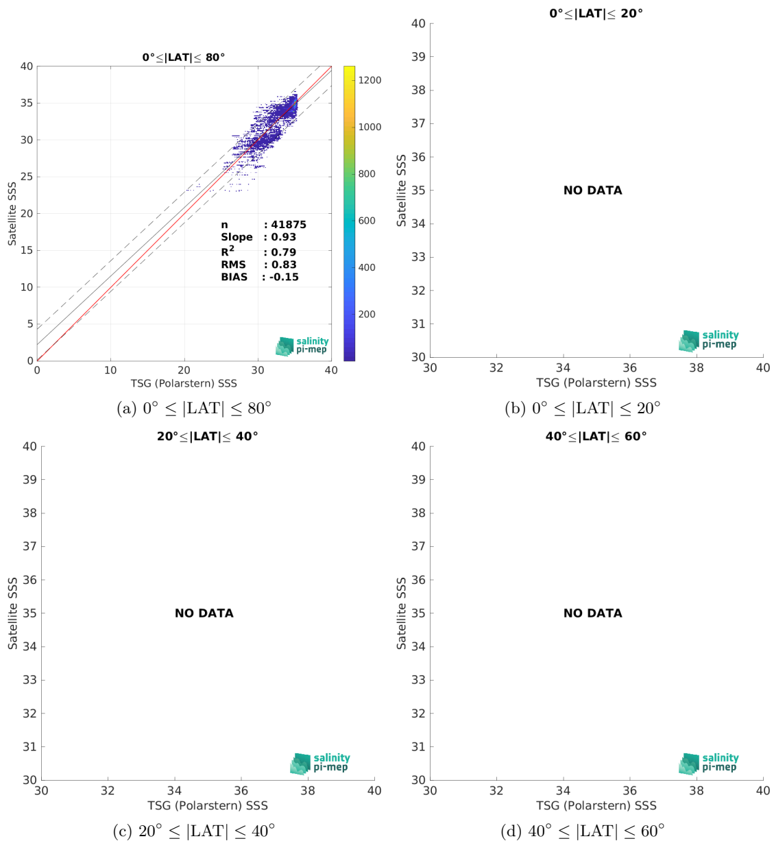
Figure 9: Contour maps of the concentration of CCI SSS L4 POLAR NH Merged-OI v4.4 - 7-day running (ESA) SSS (y-axis) versus TSG (Polarstern) SSS (x-axis) at match-up pairs for different latitude bands. For each plot, the red line shows x=y . The black thin and dashed lines indicate a linear fit through the data cloud and the \pm 95\% confidence levels, respectively. The number match-up pairs n , the slope and R^2 coefficient of the linear fit, the root mean square (RMS) and the mean bias between satellite and in situ data are indicated for each latitude band in each plots.
