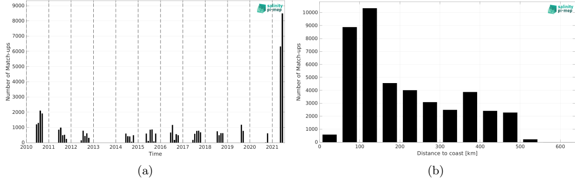
Figure 1: Number of match-ups between TSG (Polarstern) and CCI SSS L4 POLAR NH Merged-OI v4.4 - 7-day running (ESA) SSS as a function of time (a) and as function of the distance to coast (b) over the Arctic Ocean Pi-MEP region and for the full satellite product period.
