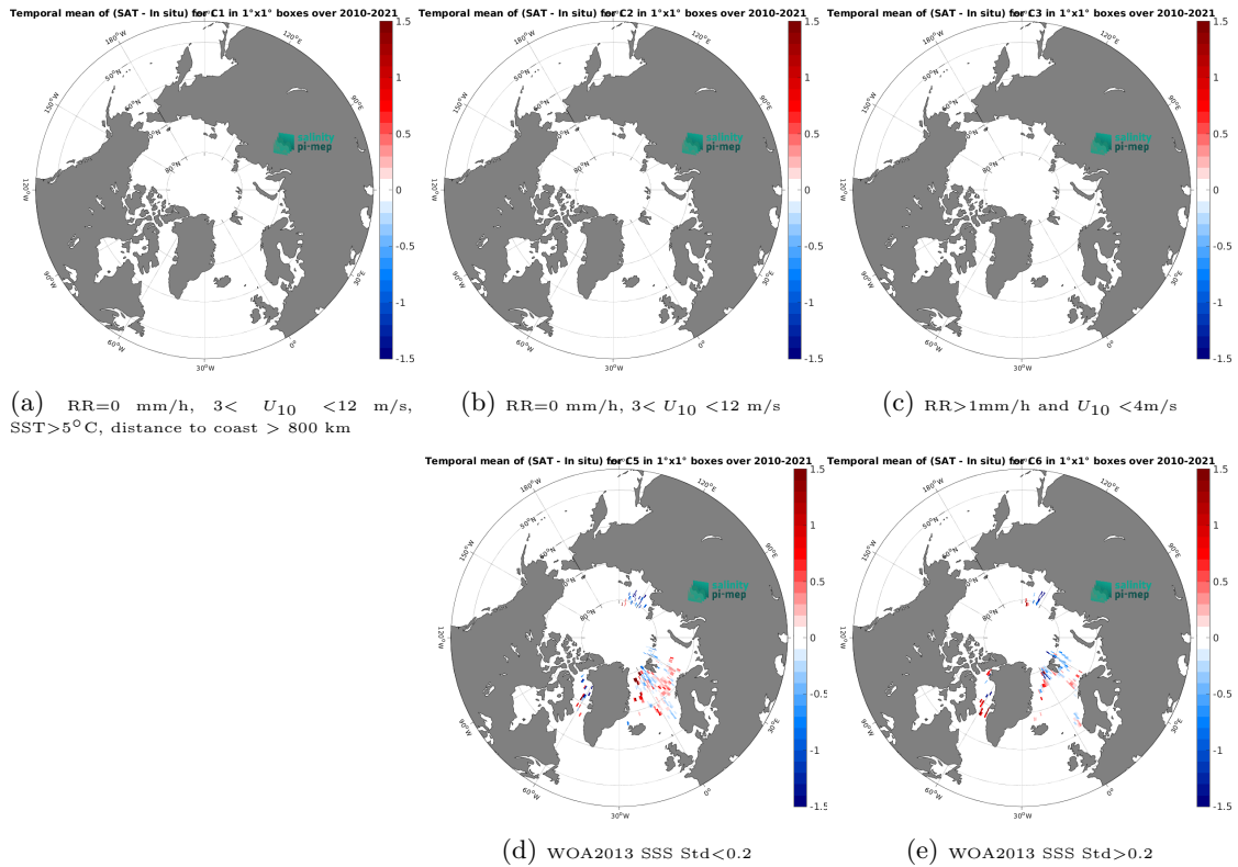
Figure 12: Temporal mean gridded over spatial boxes of size 1^{\circ}\times 1^{\circ} of \Delta\text{SSS} (CCI SSS L4 POLAR NH Merged-OI v4.4 - 7-day running (ESA) - TSG (Polarstern)) for 5 different subdatasets corresponding to:RR=0 mm/h, 3 < U_{10} < 12 m/s, SST >5^{\circ}\text{C} , distance to coast > 800 km (a), RR=0 mm/h, 3 < U_{10} < 12 m/s (b), RR >1 mm/h and U_{10} < 4 m/s (c), WOA2013 SSS Std <0.2 (d), WOA2013 SSS Std >0.2 (e).
