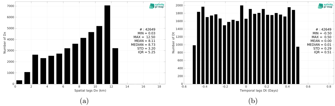
Figure 5: Histograms of the spatial (a) and temporal (b) lags between the location/time of the TSG (Polarstern) measurement and the date of the corresponding CCI SSS L4 POLAR NH Merged-OI v4.4 - 7-day running (ESA) SSS pixel.
