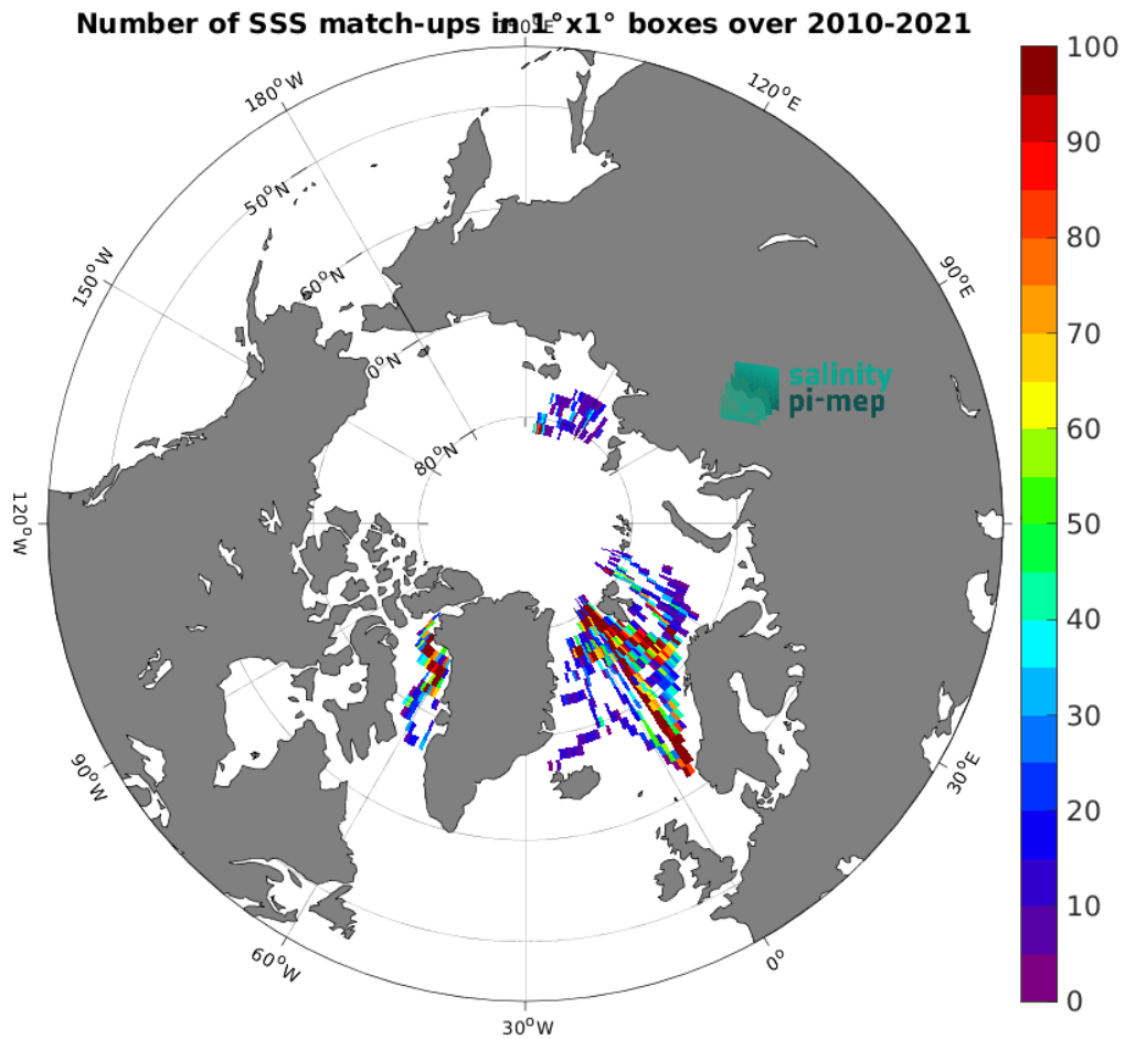
Figure 4: Number of SSS match-ups between TSG (Polarstern) SSS and the CCI SSS L4 POLAR NH Merged-OI v4.4 - 7-day running (ESA) SSS product for the Arctic Ocean Pi-MEP region over 1^{\circ} \times 1^{\circ} boxes and for the full satellite product period.
