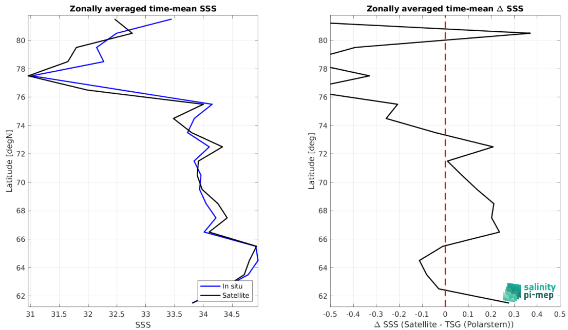
Figure 8: Left panel: Zonal mean SSS from CCI SSS L4 POLAR NH Merged-OI v4.4 - 7-day running (ESA) satellite product (black) and from TSG (Polarstern) (blue). Right panel: Zonal mean of \Delta SSS (Satellite - TSG (Polarstern)) for all the collected Pi-MEP match-up pairs estimated over the full satellite product period.
