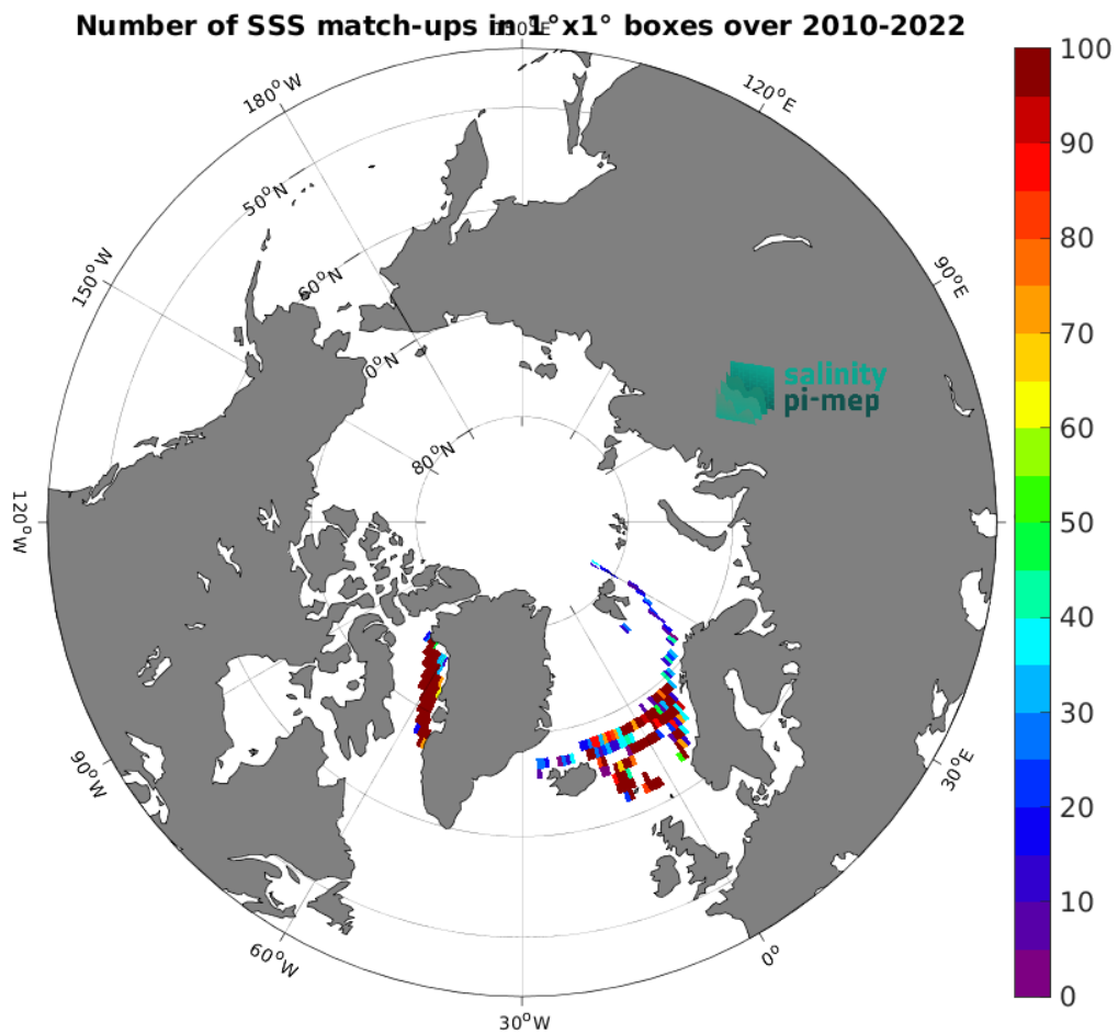
Figure 4: Number of SSS match-ups between TSG (LEGOS-DM) SSS and the CCI SSS L4 POLAR NH Merged-OI v4.4 - 7-day running (ESA) SSS product for the Arctic Ocean Pi-MEP region over 1^{\circ} \times 1^{\circ} boxes and for the full satellite product period.
