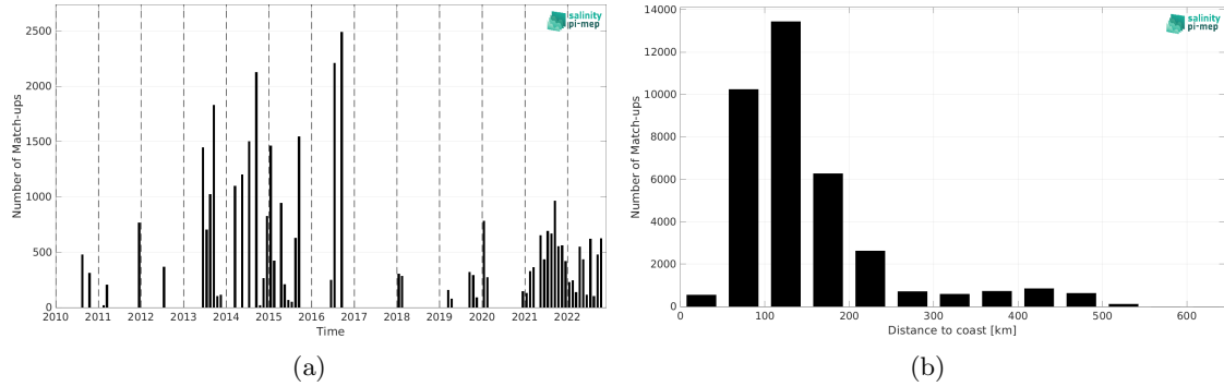
Figure 1: Number of match-ups between TSG (LEGOS-DM) and CCI SSS L4 POLAR NH Merged-OI v4.4 - 7-day running (ESA) SSS as a function of time (a) and as function of the distance to coast (b) over the Arctic Ocean Pi-MEP region and for the full satellite product period.
