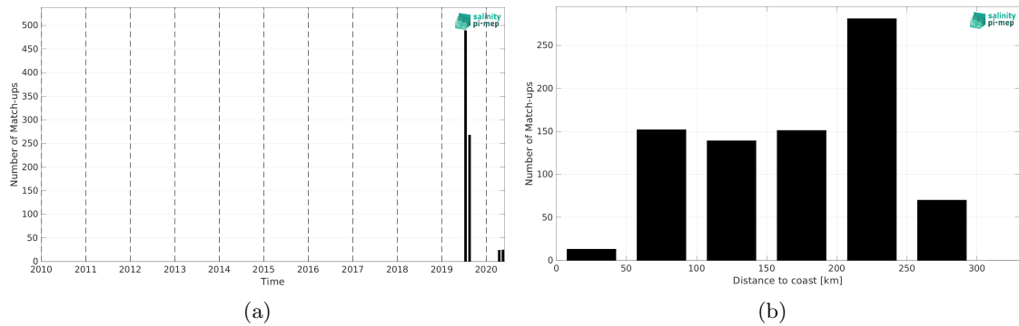
Figure 1: Number of match-ups between TSG (Lauge-Koch) and CCI SSS L4 POLAR NH Merged-OI v4.4 - 7-day running (ESA) SSS as a function of time (a) and as function of the distance to coast (b) over the Arctic Ocean Pi-MEP region and for the full satellite product period.
