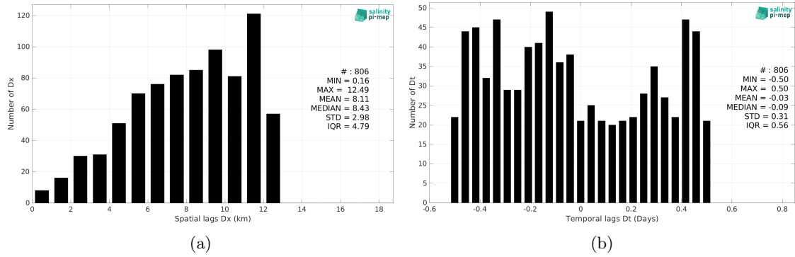
Figure 5: Histograms of the spatial (a) and temporal (b) lags between the location/time of the TSG (Lauge-Koch) measurement and the date of the corresponding CCI SSS L4 POLAR NH Merged-OI v4.4 - 7-day running (ESA) SSS pixel.
