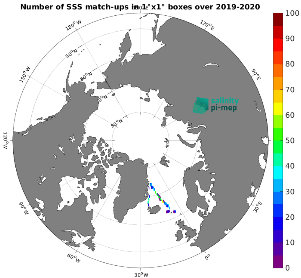
Figure 4: Number of SSS match-ups between TSG (Lauge-Koch) SSS and the CCI SSS L4 POLAR NH Merged-OI v4.4 - 7-day running (ESA) SSS product for the Arctic Ocean Pi-MEP region over 1^{\circ} \times 1^{\circ} boxes and for the full satellite product period.
