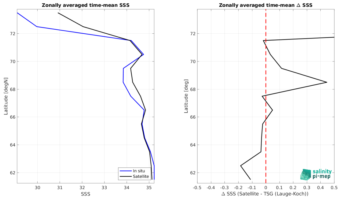
Figure 8: Left panel: Zonal mean SSS from CCI SSS L4 POLAR NH Merged-OI v4.4 - 7-day running (ESA) satellite product (black) and from TSG (Lauge-Koch) (blue). Right panel: Zonal mean of \Delta SSS (Satellite - TSG (Lauge-Koch)) for all the collected Pi-MEP match-up pairs estimated over the full satellite product period.
