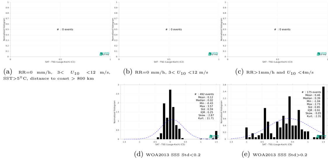
Figure 13: Normalized histogram of \Delta SSS (CCI SSS L4 POLAR NH Merged-OI v4.4 - 7-day running (ESA) - TSG (Lauge-Koch)) for 5 different subdatasets corresponding to: RR=0 mm/h, 3 < U_{10} < 12 m/s, SST>5°C, distance to coast > 800 km (a), RR=0 mm/h, 3 < U_{10} < 12 m/s (b), RR>1mm/h and U_{10} < 4 m/s (c), WOA2013 SSS Std<0.2 (d), WOA2013 SSS Std>0.2 (e).
