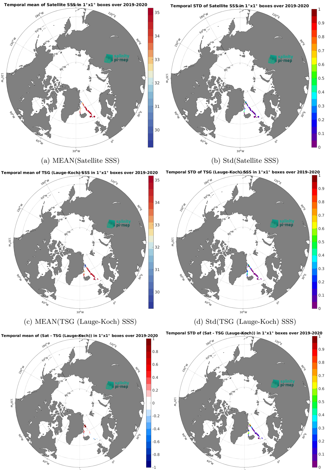
Figure 6: Temporal mean (left) and Std (right) of SSS from CCI SSS L4 POLAR NH Merged-OI v4.4 - 7-day running (ESA) (top), TSG (Lauge-Koch) (middle), and of \Delta SSS (Satellite - TSG (Lauge-Koch)). Only match-up pairs are used to generate these maps.
