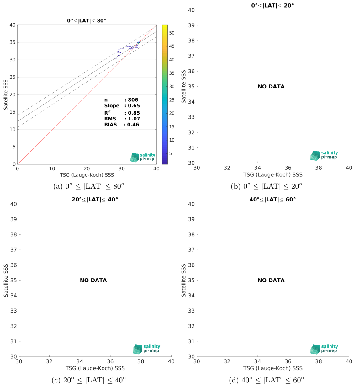
Figure 9: Contour maps of the concentration of CCI SSS L4 POLAR NH Merged-OI v4.4 - 7-day running (ESA) SSS (y-axis) versus TSG (Lauge-Koch) SSS (x-axis) at match-up pairs for different latitude bands. For each plot, the red line shows x=y . The black thin and dashed lines indicate a linear fit through the data cloud and the \pm 95\% confidence levels, respectively. The number match-up pairs n , the slope and R^2 coefficient of the linear fit, the root mean square (RMS) and the mean bias between satellite and in situ data are indicated for each latitude band in each plots.
