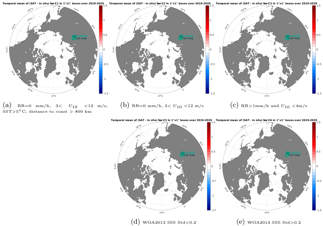
Figure 12: Temporal mean gridded over spatial boxes of size 1^{\circ}\times 1^{\circ} of \Delta\text{SSS} (CCI SSS L4 POLAR NH Merged-OI v4.4 - 7-day running (ESA) - TSG (Lauge-Koch)) for 5 different subdatasets corresponding to:RR=0 mm/h, 3 < U_{10} < 12 m/s, SST >5^{\circ}\text{C} , distance to coast > 800 km (a), RR=0 mm/h, 3 < U_{10} < 12 m/s (b), RR >1 mm/h and U_{10} < 4 m/s (c), WOA2013 SSS Std <0.2 (d), WOA2013 SSS Std >0.2 (e).
