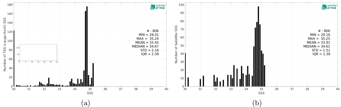
Figure 2: Histograms of SSS from TSG (Lauge-Koch) (a) and CCI SSS L4 POLAR NH Merged-OI v4.4 - 7-day running (ESA) (b) considering all match-up pairs per bins of 0.1 over the Arctic Ocean Pi-MEP region and for the full satellite product period.
