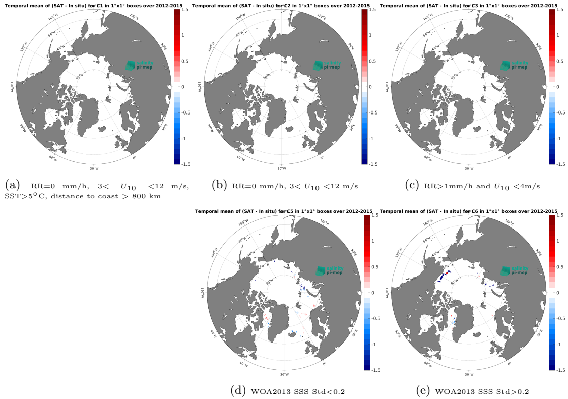
Figure 12: Temporal mean gridded over spatial boxes of size 1^\circ \times 1^\circ of \Delta SSS (CCI SSS L4 POLAR NH Merged-OI v4.4 - 7-day running (ESA) - TSG (GOSUD-Sailing-ship)) for 5 different subdatasets corresponding to: RR=0 mm/h, 3 < U_{10} < 12 m/s, SST>5°C, distance to coast > 800 km (a), RR=0 mm/h, 3 < U_{10} < 12 m/s (b), RR>1mm/h and U_{10} < 4 m/s (c), WOA2013 SSS Std<0.2 (d), WOA2013 SSS Std>0.2 (e).
