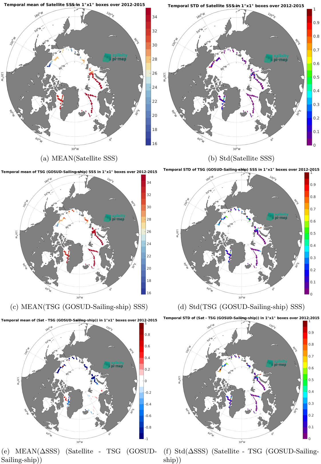
Figure 6: Temporal mean (left) and Std (right) of SSS from CCI SSS L4 POLAR NH Merged-OI v4.4 - 7-day running (ESA) (top), TSG (GOSUD-Sailing-ship) (middle), and of \Delta SSS (Satellite - TSG (GOSUD-Sailing-ship)). Only match-up pairs are used to generate these maps.
