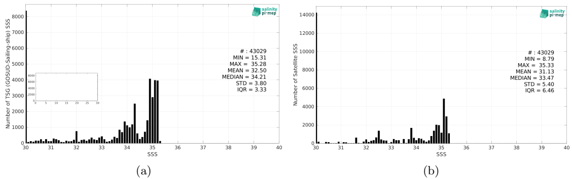
Figure 2: Histograms of SSS from TSG (GOSUD-Sailing-ship) (a) and CCI SSS L4 POLAR NH Merged-OI v4.4 - 7-day running (ESA) (b) considering all match-up pairs per bins of 0.1 over the Arctic Ocean Pi-MEP region and for the full satellite product period.
