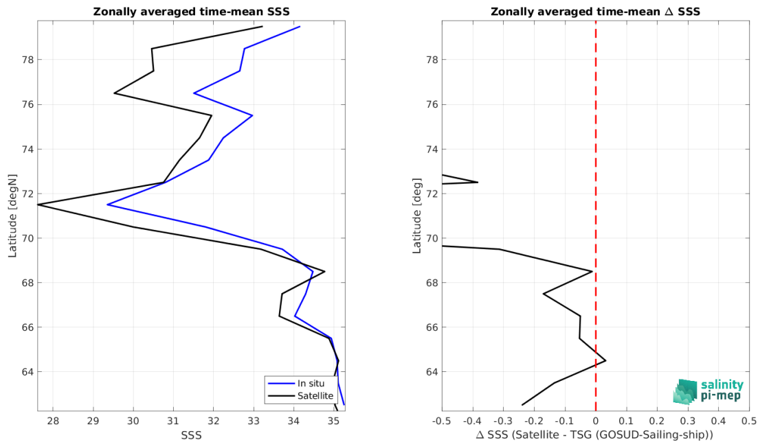
Figure 8: Left panel: Zonal mean SSS from CCI SSS L4 POLAR NH Merged-OI v4.4 - 7-day running (ESA) satellite product (black) and from TSG (GOSUD-Sailing-ship) (blue). Right panel: Zonal mean of \Delta SSS (Satellite - TSG (GOSUD-Sailing-ship)) for all the collected Pi-MEP match-up pairs estimated over the full satellite product period.
