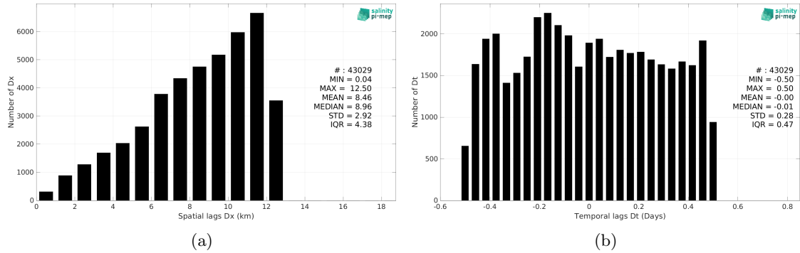
Figure 5: Histograms of the spatial (a) and temporal (b) lags between the location/time of the TSG (GOSUD-Sailing-ship) measurement and the date of the corresponding CCI SSS L4 POLAR NH Merged-OI v4.4 - 7-day running (ESA) SSS pixel.
