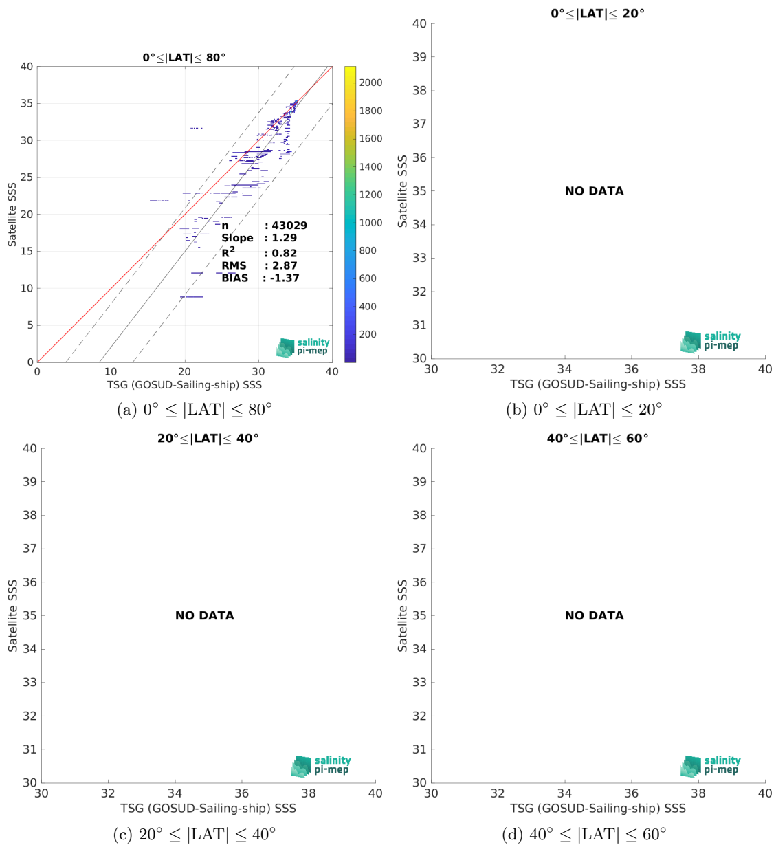
Figure 9: Contour maps of the concentration of CCI SSS L4 POLAR NH Merged-OI v4.4 - 7-day running (ESA) SSS (y-axis) versus TSG (GOSUD-Sailing-ship) SSS (x-axis) at match-up pairs for different latitude bands. For each plot, the red line shows x=y . The black thin and dashed lines indicate a linear fit through the data cloud and the \pm 95\% confidence levels, respectively. The number match-up pairs n , the slope and R^2 coefficient of the linear fit, the root mean square (RMS) and the mean bias between satellite and in situ data are indicated for each latitude band in each plots.
