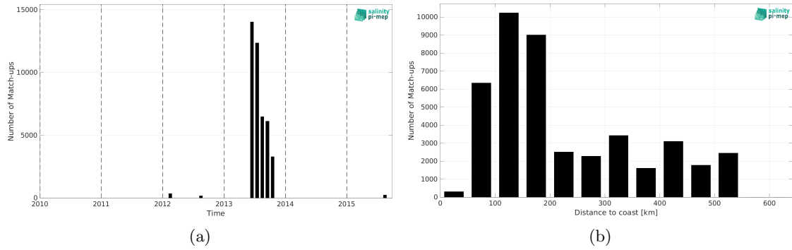
Figure 1: Number of match-ups between TSG (GOSUD-Sailing-ship) and CCI SSS L4 POLAR NH Merged-OI v4.4 - 7-day running (ESA) SSS as a function of time (a) and as function of the distance to coast (b) over the Arctic Ocean Pi-MEP region and for the full satellite product period.
