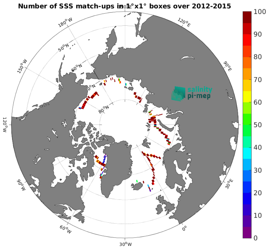
Figure 4: Number of SSS match-ups between TSG (GOSUD-Sailing-ship) SSS and the CCI SSS L4 POLAR NH Merged-OI v4.4 - 7-day running (ESA) SSS product for the Arctic Ocean Pi-MEP region over 1^{\circ} \times 1^{\circ} boxes and for the full satellite product period.
