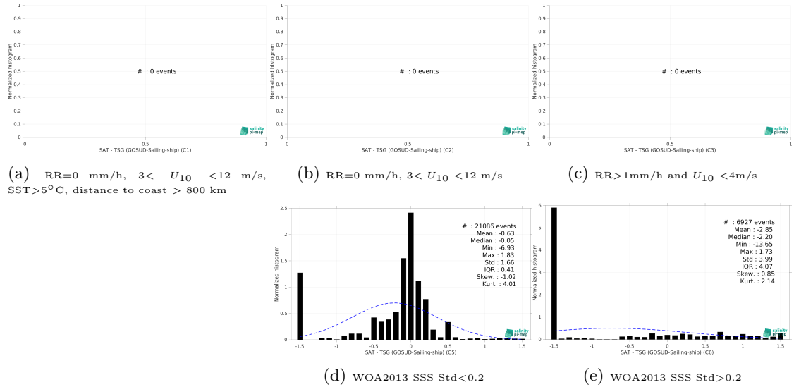
Figure 13: Normalized histogram of \Delta SSS (CCI SSS L4 POLAR NH Merged-OI v4.4 - 7-day running (ESA) - TSG (GOSUD-Sailing-ship)) for 5 different subdatasets corresponding to: RR=0 mm/h, 3 < U_{10} < 12 m/s, SST > 5°C, distance to coast > 800 km (a), RR=0 mm/h, 3 < U_{10} < 12 m/s (b), RR > 1mm/h and U_{10} < 4 m/s (c), WOA2013 SSS Std < 0.2 (d), WOA2013 SSS Std > 0.2 (e).
