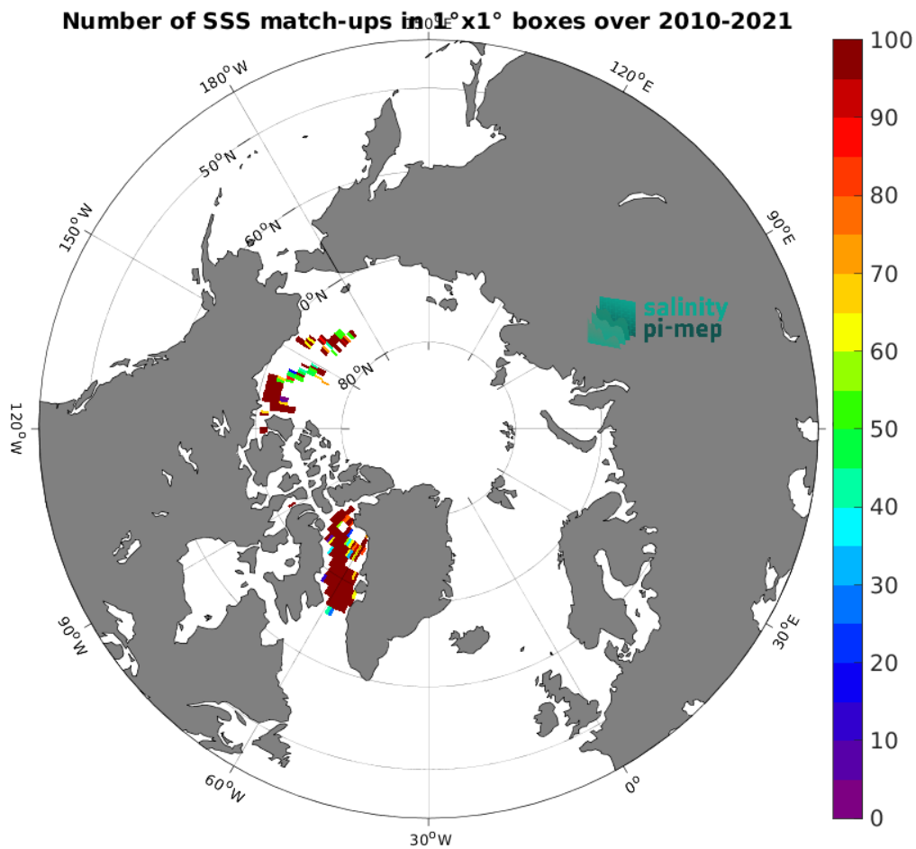
Figure 4: Number of SSS match-ups between TSG (Amundsen) SSS and the CCI SSS L4 POLAR NH Merged-OI v4.4 - 7-day running (ESA) SSS product for the Arctic Ocean Pi-MEP region over 1^{\circ} \times 1^{\circ} boxes and for the full satellite product period.
