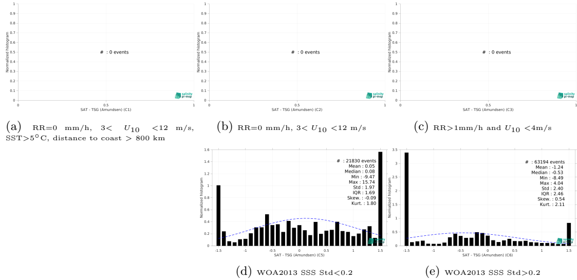
Figure 13: Normalized histogram of \Delta SSS (CCI SSS L4 POLAR NH Merged-OI v4.4 - 7-day running (ESA) - TSG (Amundsen)) for 5 different subdatasets corresponding to: RR=0 mm/h, 3 < U_{10} < 12 m/s, SST > 5°C, distance to coast > 800 km (a), RR=0 mm/h, 3 < U_{10} < 12 m/s (b), RR > 1mm/h and U_{10} < 4 m/s (c), WOA2013 SSS Std < 0.2 (d), WOA2013 SSS Std > 0.2 (e).
