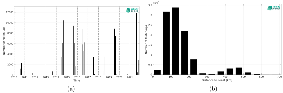
Figure 1: Number of match-ups between TSG (Amundsen) and CCI SSS L4 POLAR NH Merged-OI v4.4 - 7-day running (ESA) SSS as a function of time (a) and as function of the distance to coast (b) over the Arctic Ocean Pi-MEP region and for the full satellite product period.
