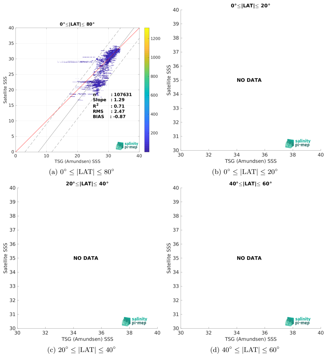
Figure 9: Contour maps of the concentration of CCI SSS L4 POLAR NH Merged-OI v4.4 - 7-day running (ESA) SSS (y-axis) versus TSG (Amundsen) SSS (x-axis) at match-up pairs for different latitude bands. For each plot, the red line shows x=y . The black thin and dashed lines indicate a linear fit through the data cloud and the \pm 95\% confidence levels, respectively. The number match-up pairs n , the slope and R^2 coefficient of the linear fit, the root mean square (RMS) and the mean bias between satellite and in situ data are indicated for each latitude band in each plots.
