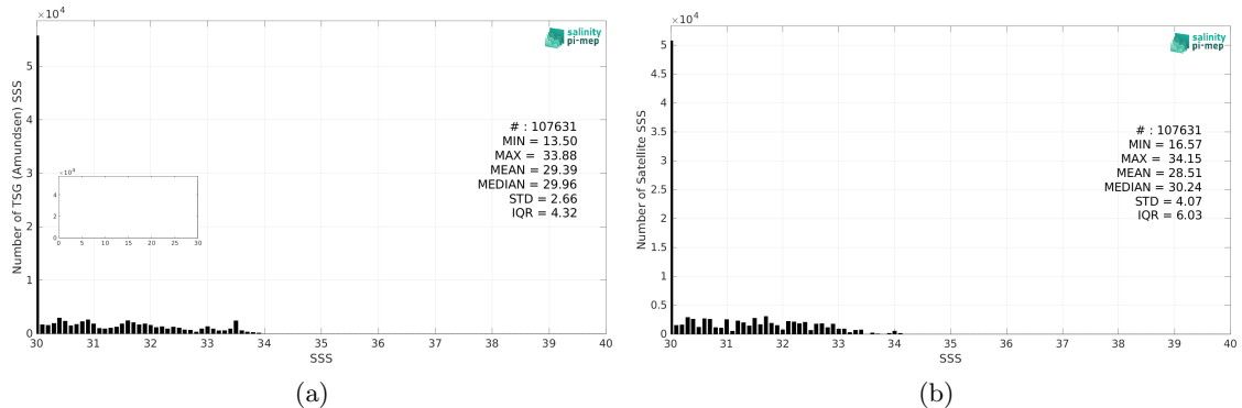
Figure 2: Histograms of SSS from TSG (Amundsen) (a) and CCI SSS L4 POLAR NH Merged-OI v4.4 - 7-day running (ESA) (b) considering all match-up pairs per bins of 0.1 over the Arctic Ocean Pi-MEP region and for the full satellite product period.
