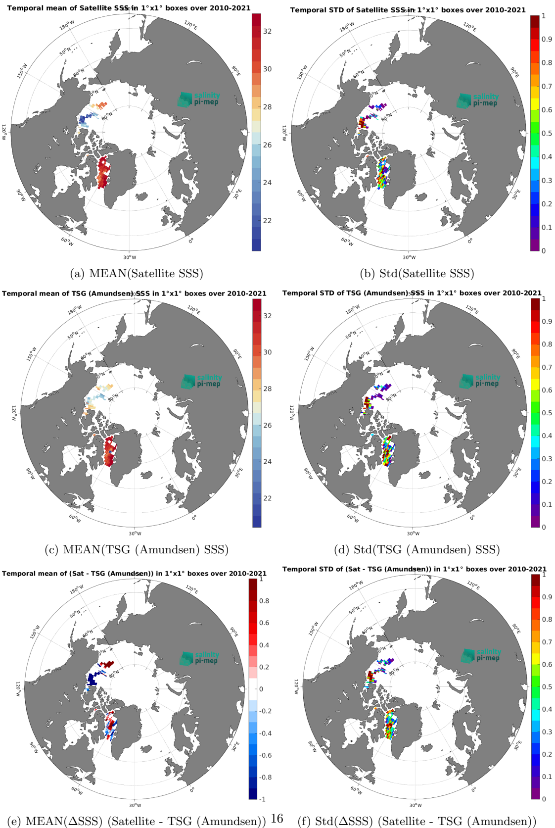
Figure 6: Temporal mean (left) and Std (right) of SSS from CCI SSS L4 POLAR NH Merged-OI v4.4 - 7-day running (ESA) (top), TSG (Amundsen) (middle), and of \Delta SSS (Satellite - TSG (Amundsen)). Only match-up pairs are used to generate these maps.
