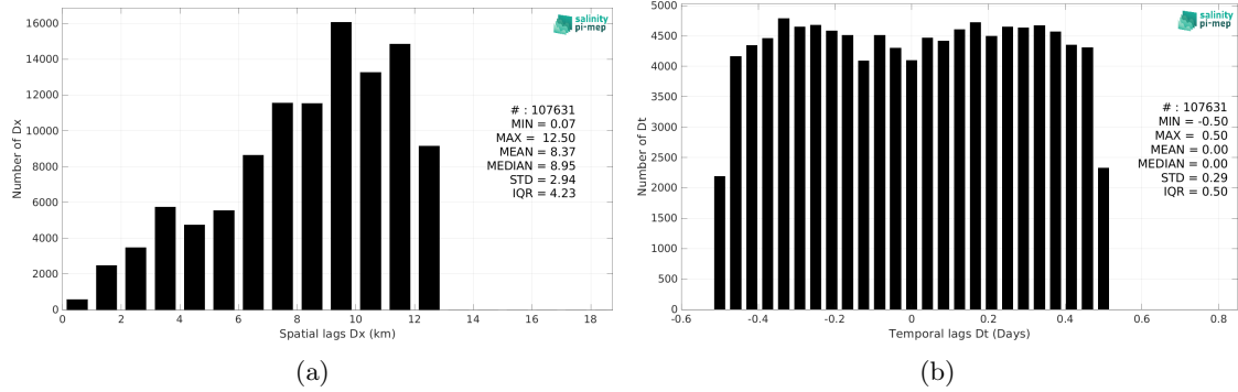
Figure 5: Histograms of the spatial (a) and temporal (b) lags between the location/time of the TSG (Amundsen) measurement and the date of the corresponding CCI SSS L4 POLAR NH Merged-OI v4.4 - 7-day running (ESA) SSS pixel.
