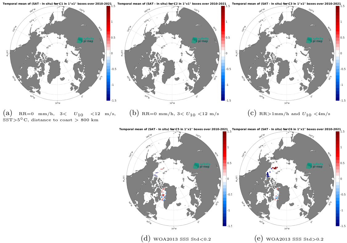
Figure 12: Temporal mean gridded over spatial boxes of size 1^{\circ}\times 1^{\circ} of \Delta\text{SSS} (CCI SSS L4 POLAR NH Merged-OI v4.4 - 7-day running (ESA) - TSG (Amundsen)) for 5 different subdatasets corresponding to:RR=0 mm/h, 3 < U_{10} < 12 m/s, SST >5^{\circ}\text{C} , distance to coast > 800 km (a), RR=0 mm/h, 3 < U_{10} < 12 m/s (b), RR >1 mm/h and U_{10} < 4 m/s (c), WOA2013 SSS Std <0.2 (d), WOA2013 SSS Std >0.2 (e).
