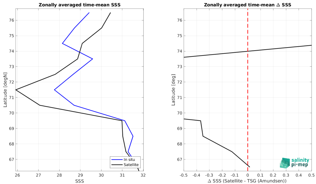
Figure 8: Left panel: Zonal mean SSS from CCI SSS L4 POLAR NH Merged-OI v4.4 - 7-day running (ESA) satellite product (black) and from TSG (Amundsen) (blue). Right panel: Zonal mean of \Delta SSS (Satellite - TSG (Amundsen)) for all the collected Pi-MEP match-up pairs estimated over the full satellite product period.
