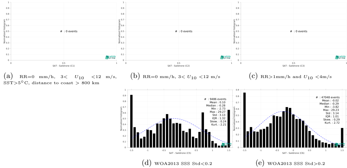
Figure 13: Normalized histogram of \Delta SSS (CCI SSS L4 POLAR NH Merged-OI v4.4 - 7-day running (ESA) - Saldrone) for 5 different subdatasets corresponding to: RR=0 mm/h, 3 < U_{10} < 12 m/s, SST >5^{\circ} C, distance to coast > 800 km (a), RR=0 mm/h, 3 < U_{10} < 12 m/s (b), RR >1 mm/h and U_{10} < 4 m/s (c), WOA2013 SSS Std <0.2 (d), WOA2013 SSS Std >0.2 (e).
