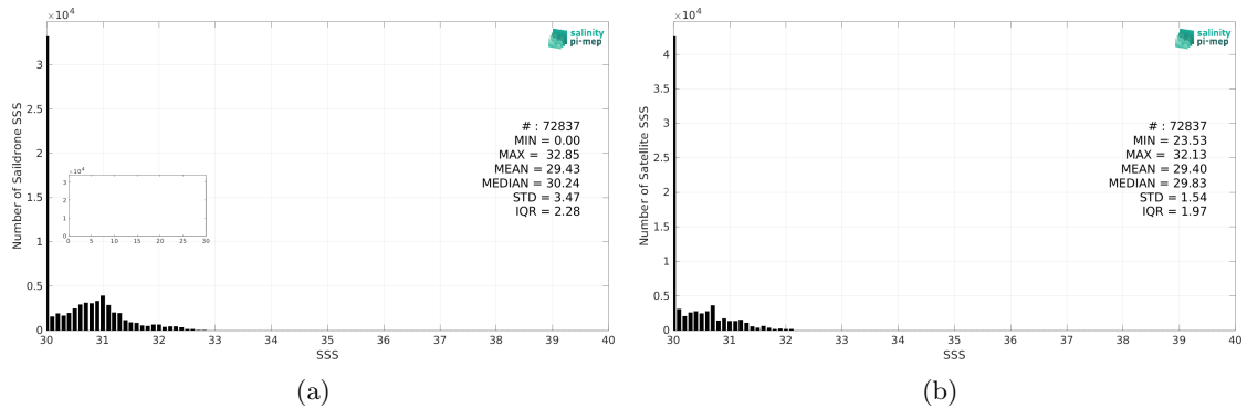
Figure 2: Histograms of SSS from Sailldrone (a) and CCI SSS L4 POLAR NH Merged-OI v4.4 - 7-day running (ESA) (b) considering all match-up pairs per bins of 0.1 over the Arctic Ocean Pi-MEP region and for the full satellite product period.
