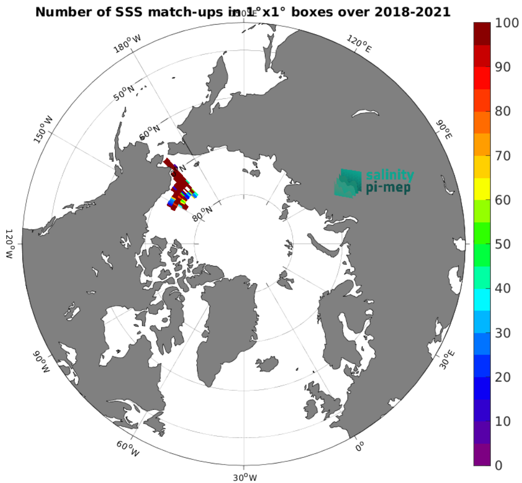
Figure 4: Number of SSS match-ups between Saildrone SSS and the CCI SSS L4 POLAR NH Merged-OI v4.4 - 7-day running (ESA) SSS product for the Arctic Ocean Pi-MEP region over 1^{\circ} \times 1^{\circ} boxes and for the full satellite product period.
