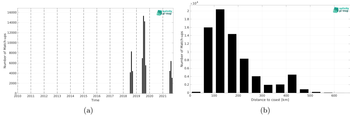
Figure 1: Number of match-ups between Sailldrone and CCI SSS L4 POLAR NH Merged-OI v4.4 - 7-day running (ESA) SSS as a function of time (a) and as function of the distance to coast (b) over the Arctic Ocean Pi-MEP region and for the full satellite product period.
