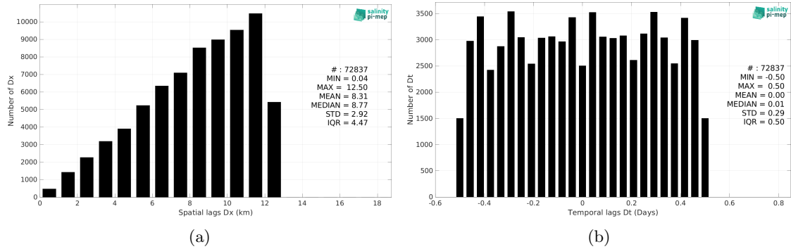
Figure 5: Histograms of the spatial (a) and temporal (b) lags between the location/time of the Saildrone measurement and the date of the corresponding CCI SSS L4 POLAR NH Merged-OI v4.4 - 7-day running (ESA) SSS pixel.
