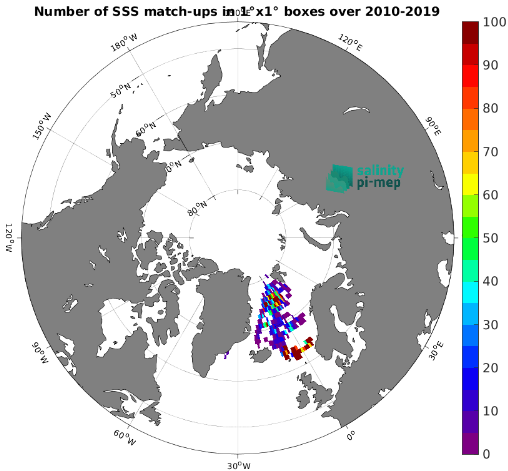
Figure 3: Number of SSS match-ups between Surface drifters SSS and the CCI SSS L4 POLAR NH Merged-OI v4.4 - 7-day running (ESA) SSS product for the Arctic Ocean Pi-MEP region over 1^{\circ} \times 1^{\circ} boxes and for the full satellite product period.
