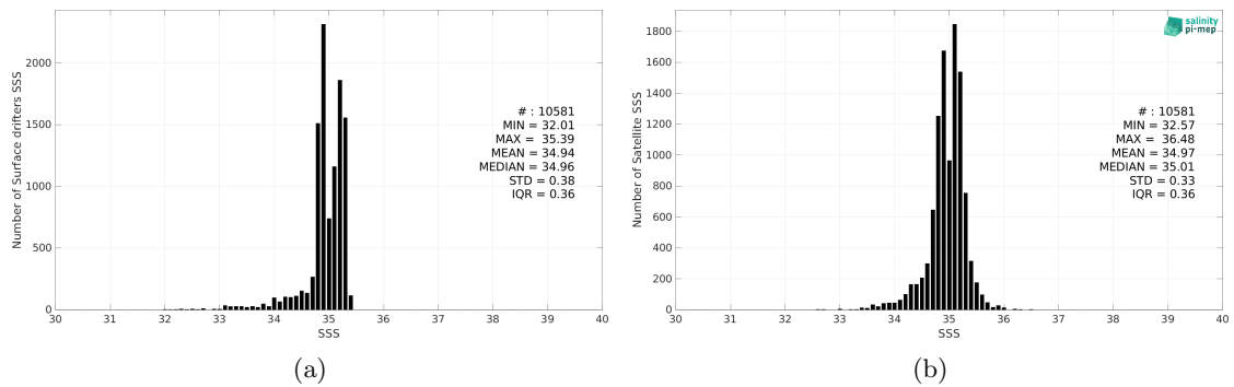
Figure 2: Histograms of SSS from Surface drifters (a) and CCI SSS L4 POLAR NH Merged-OI v4.4 - 7-day running (ESA) (b) considering all match-up pairs per bins of 0.1 over the Arctic Ocean Pi-MEP region and for the full satellite product period.
