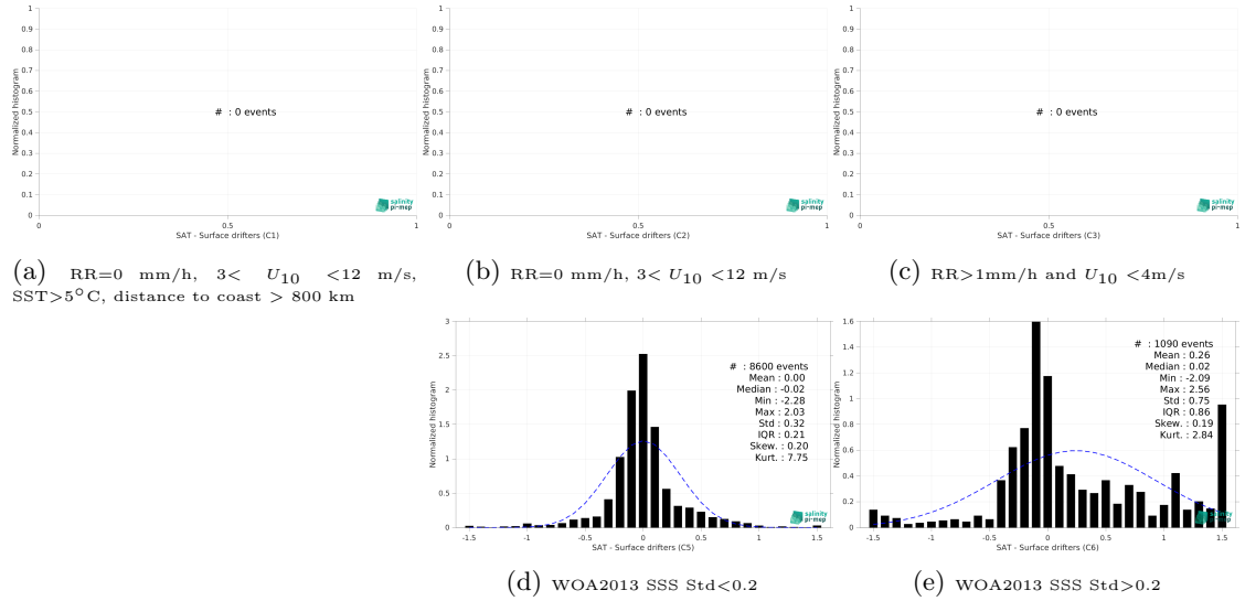
Figure 12: Normalized histogram of \Delta SSS (CCI SSS L4 POLAR NH Merged-OI v4.4 - 7-day running (ESA) - Surface drifters) for 5 different subdatasets corresponding to: RR=0 mm/h, 3 < U_{10} < 12 m/s, SST > 5°C, distance to coast > 800 km (a), RR=0 mm/h, 3 < U_{10} < 12 m/s (b), RR > 1mm/h and U_{10} < 4 m/s (c), WOA2013 SSS Std < 0.2 (d), WOA2013 SSS Std > 0.2 (e).
