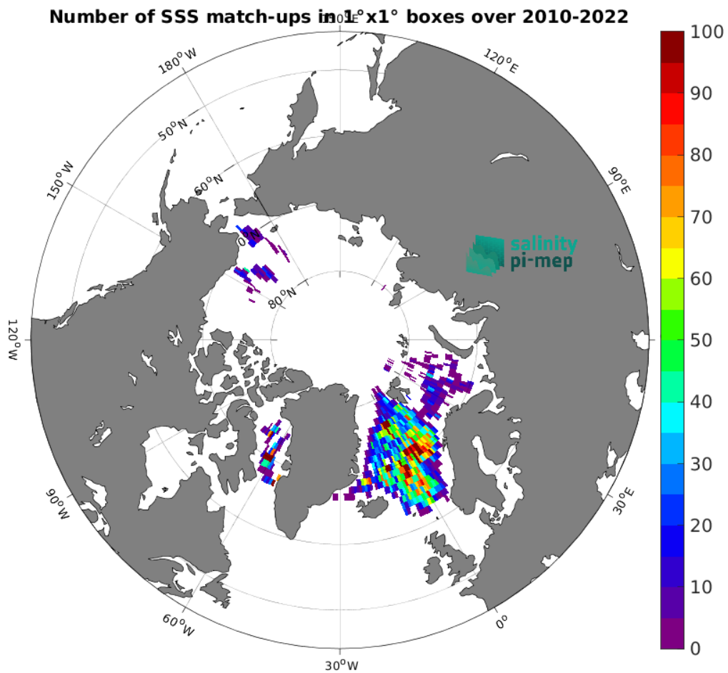
Figure 4: Number of SSS match-ups between Argo SSS and the CCI SSS L4 POLAR NH Merged-OI v4.4 - 7-day running (ESA) SSS product for the Arctic Ocean Pi-MEP region over 1^{\circ} \times 1^{\circ} boxes and for the full satellite product period.
