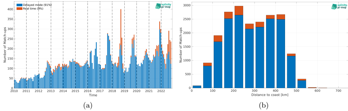
Figure 1: Number of match-ups between Argo and CCI SSS L4 POLAR NH Merged-OI v4.4 - 7-day running (ESA) SSS as a function of time (a) and as function of the distance to coast (b) over the Arctic Ocean Pi-MEP region and for the full satellite product period.
