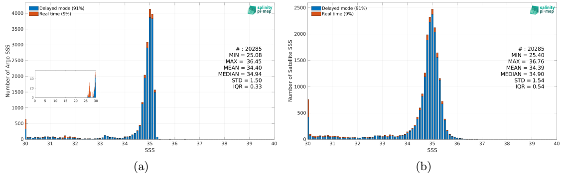
Figure 2: Histograms of SSS from Argo (a) and CCI SSS L4 POLAR NH Merged-OI v4.4 - 7-day running (ESA) (b) considering all match-up pairs per bins of 0.1 over the Arctic Ocean Pi-MEP region and for the full satellite product period.
