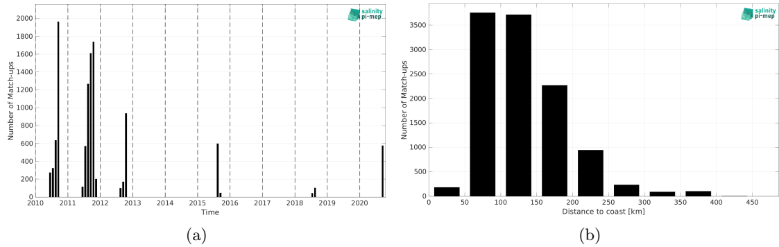
Figure 1: Number of match-ups between TSG (SAMOS) and CCI SSS L4 POLAR NH Merged-OI v4.4 - 30-day running (ESA) SSS as a function of time (a) and as function of the distance to coast (b) over the Arctic Ocean Pi-MEP region and for the full satellite product period.
