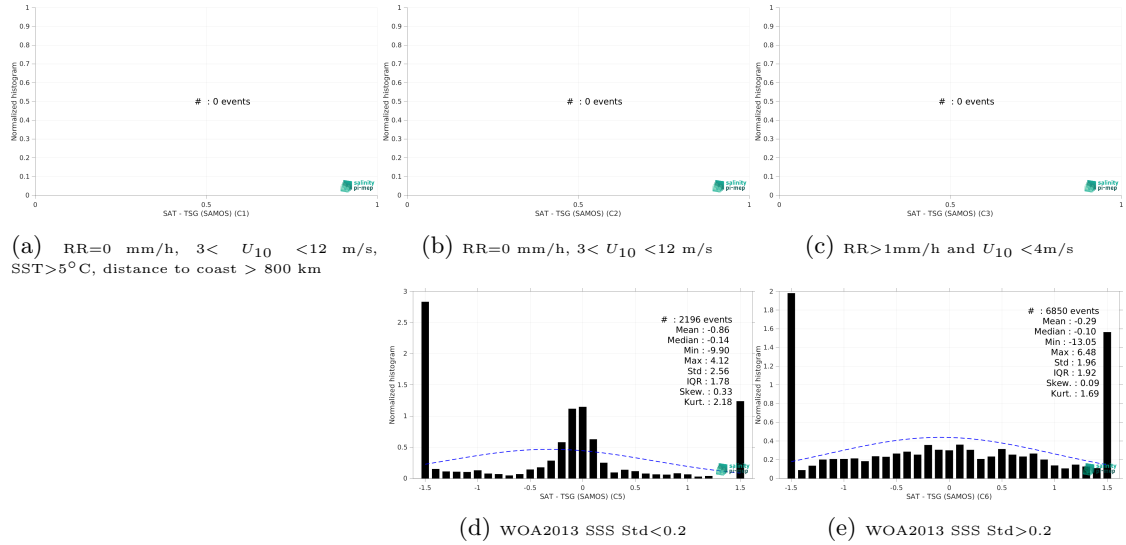
Figure 13: Normalized histogram of \Delta SSS (CCI SSS L4 POLAR NH Merged-OI v4.4 - 30-day running (ESA) - TSG (SAMOS)) for 5 different subdatasets corresponding to: RR=0 mm/h, 3 < U_{10} < 12 m/s, SST>5°C, distance to coast > 800 km (a), RR=0 mm/h, 3 < U_{10} < 12 m/s (b), RR>1mm/h and U_{10} < 4 m/s (c), WOA2013 SSS Std<0.2 (d), WOA2013 SSS Std>0.2 (e).
