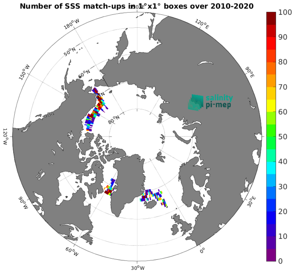
Figure 4: Number of SSS match-ups between TSG (SAMOS) SSS and the CCI SSS L4 POLAR NH Merged-OI v4.4 - 30-day running (ESA) SSS product for the Arctic Ocean Pi-MEP region over 1^{\circ} \times 1^{\circ} boxes and for the full satellite product period.
