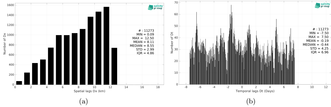
Figure 5: Histograms of the spatial (a) and temporal (b) lags between the location/time of the TSG (SAMOS) measurement and the date of the corresponding CCI SSS L4 POLAR NH Merged-OI v4.4 - 30-day running (ESA) SSS pixel.
