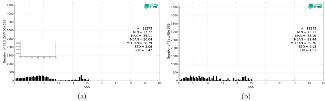
Figure 2: Histograms of SSS from TSG (SAMOS) (a) and CCI SSS L4 POLAR NH Merged-OI v4.4 - 30-day running (ESA) (b) considering all match-up pairs per bins of 0.1 over the Arctic Ocean Pi-MEP region and for the full satellite product period.
