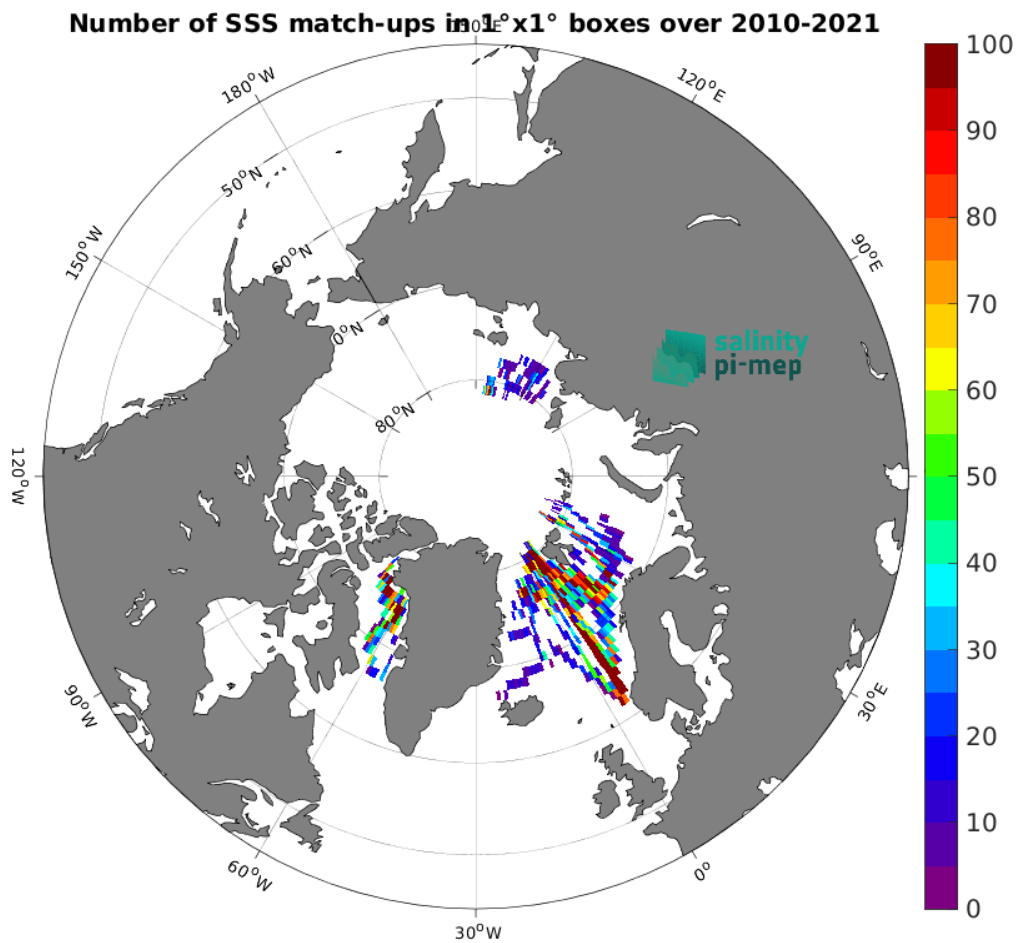
Figure 4: Number of SSS match-ups between TSG (Polarstern) SSS and the CCI SSS L4 POLAR NH Merged-OI v4.4 - 30-day running (ESA) SSS product for the Arctic Ocean Pi-MEP region over 1^{\circ} \times 1^{\circ} boxes and for the full satellite product period.
