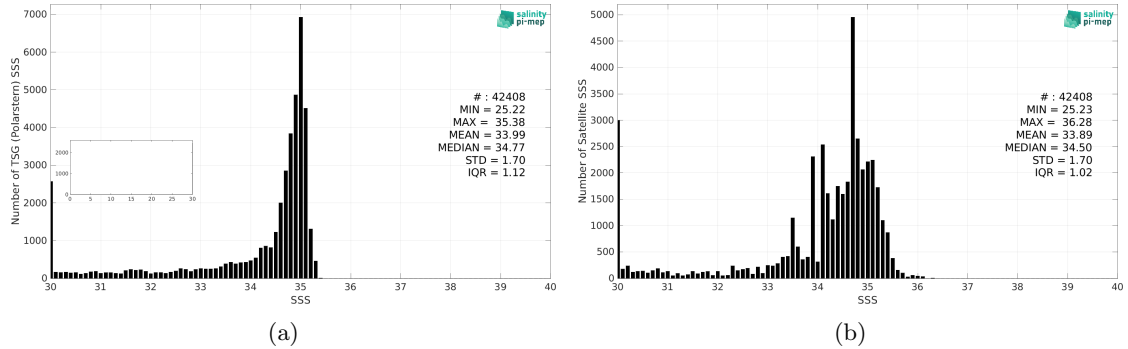
Figure 2: Histograms of SSS from TSG (Polarstern) (a) and CCI SSS L4 POLAR NH Merged-OI v4.4 - 30-day running (ESA) (b) considering all match-up pairs per bins of 0.1 over the Arctic Ocean Pi-MEP region and for the full satellite product period.
