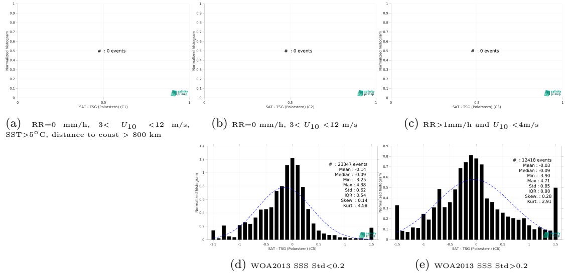
Figure 13: Normalized histogram of \Delta SSS (CCI SSS L4 POLAR NH Merged-OI v4.4 - 30-day running (ESA) - TSG (Polarstern)) for 5 different subdatasets corresponding to: RR=0 mm/h, 3 < U_{10} < 12 m/s, SST>5°C, distance to coast > 800 km (a), RR=0 mm/h, 3 < U_{10} < 12 m/s (b), RR>1mm/h and U_{10} < 4 m/s (c), WOA2013 SSS Std<0.2 (d), WOA2013 SSS Std>0.2 (e).
