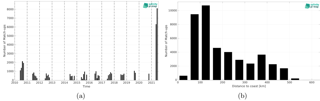
Figure 1: Number of match-ups between TSG (Polarstern) and CCI SSS L4 POLAR NH Merged-OI v4.4 - 30-day running (ESA) SSS as a function of time (a) and as function of the distance to coast (b) over the Arctic Ocean Pi-MEP region and for the full satellite product period.
