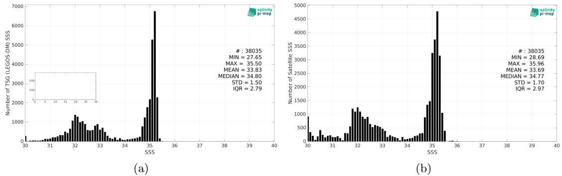
Figure 2: Histograms of SSS from TSG (LEGOS-DM) (a) and CCI SSS L4 POLAR NH Merged-OI v4.4 - 30-day running (ESA) (b) considering all match-up pairs per bins of 0.1 over the Arctic Ocean Pi-MEP region and for the full satellite product period.
