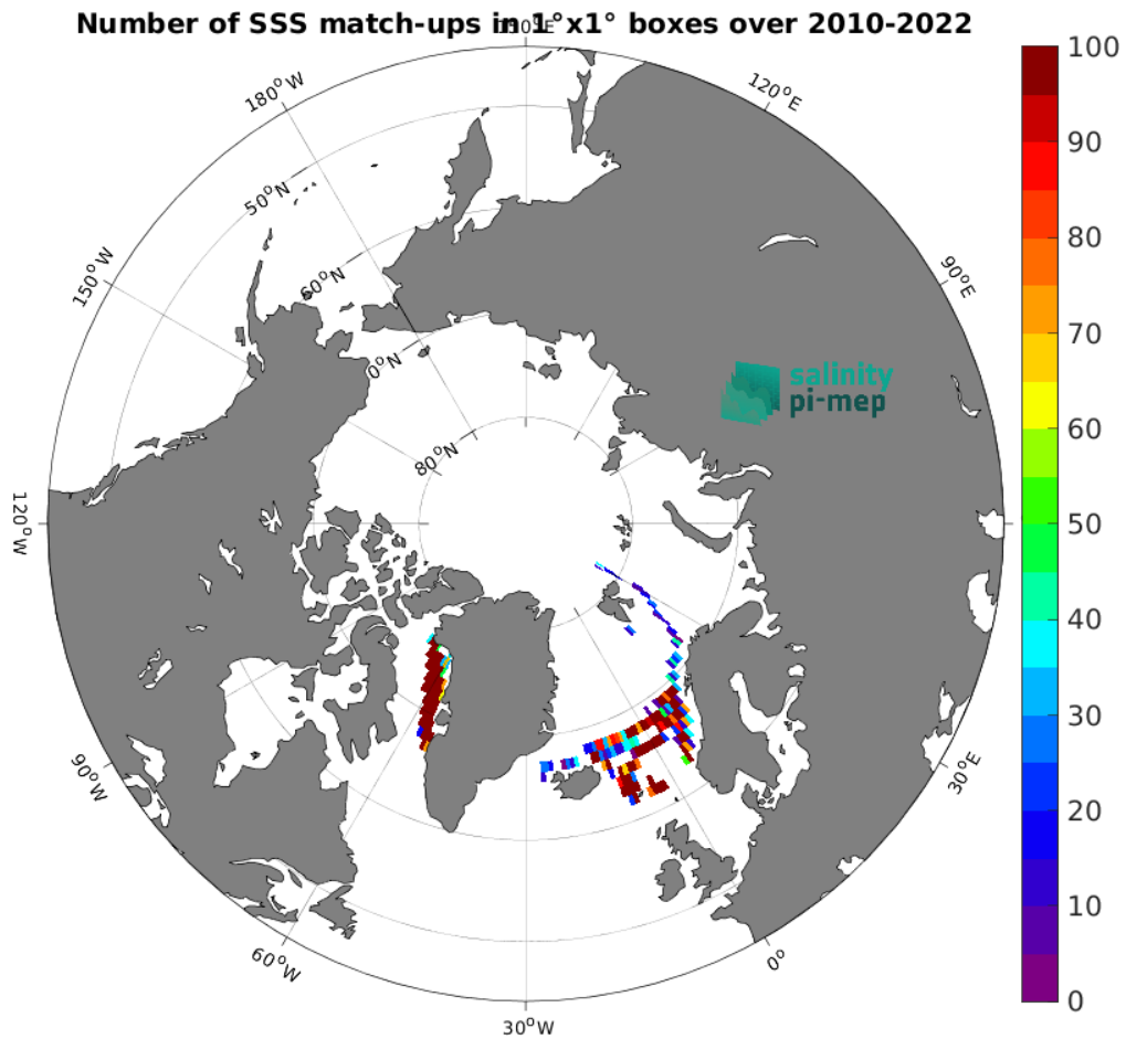
Figure 4: Number of SSS match-ups between TSG (LEGOS-DM) SSS and the CCI SSS L4 POLAR NH Merged-OI v4.4 - 30-day running (ESA) SSS product for the Arctic Ocean Pi-MEP region over 1^{\circ} \times 1^{\circ} boxes and for the full satellite product period.
