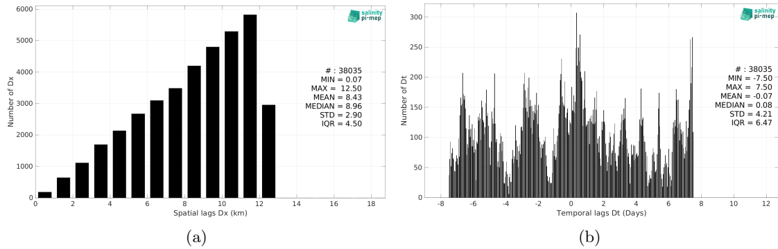
Figure 5: Histograms of the spatial (a) and temporal (b) lags between the location/time of the TSG (LEGOS-DM) measurement and the date of the corresponding CCI SSS L4 POLAR NH Merged-OI v4.4 - 30-day running (ESA) SSS pixel.
