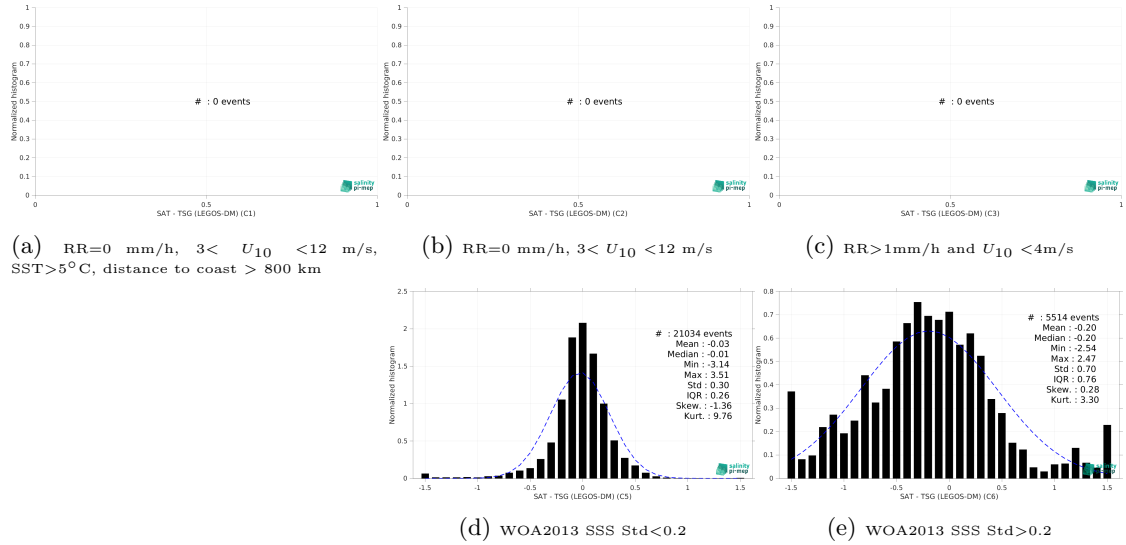
Figure 13: Normalized histogram of \Delta SSS (CCI SSS L4 POLAR NH Merged-OI v4.4 - 30-day running (ESA) - TSG (LEGOS-DM)) for 5 different subdatasets corresponding to: RR=0 mm/h, 3 < U_{10} < 12 m/s, SST>5°C, distance to coast > 800 km (a), RR=0 mm/h, 3 < U_{10} < 12 m/s (b), RR>1mm/h and U_{10} < 4 m/s (c), WOA2013 SSS Std<0.2 (d), WOA2013 SSS Std>0.2 (e).
