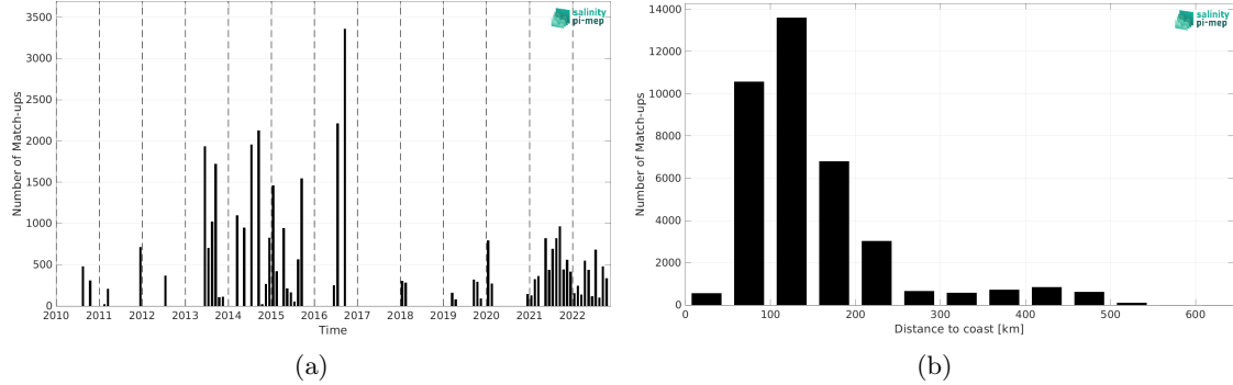
Figure 1: Number of match-ups between TSG (LEGOS-DM) and CCI SSS L4 POLAR NH Merged-OI v4.4 - 30-day running (ESA) SSS as a function of time (a) and as function of the distance to coast (b) over the Arctic Ocean Pi-MEP region and for the full satellite product period.
