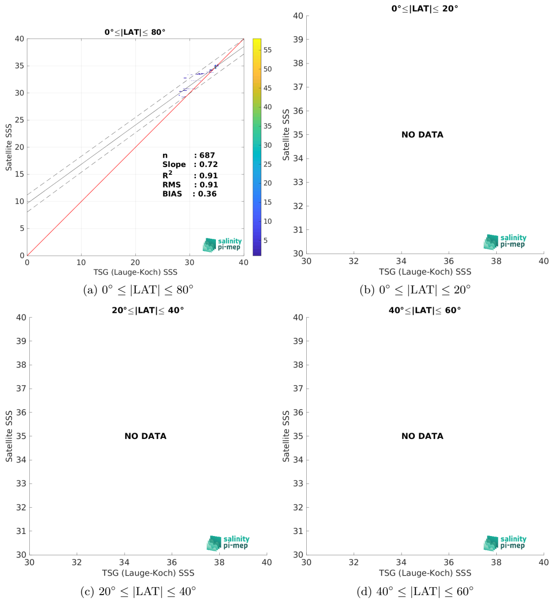
Figure 9: Contour maps of the concentration of CCI SSS L4 POLAR NH Merged-OI v4.4 - 30-day running (ESA) SSS (y-axis) versus TSG (Lauge-Koch) SSS (x-axis) at match-up pairs for different latitude bands. For each plot, the red line shows x=y . The black thin and dashed lines indicate a linear fit through the data cloud and the \pm 95\% confidence levels, respectively. The number match-up pairs n , the slope and R^2 coefficient of the linear fit, the root mean square (RMS) and the mean bias between satellite and in situ data are indicated for each latitude band in each plots.
