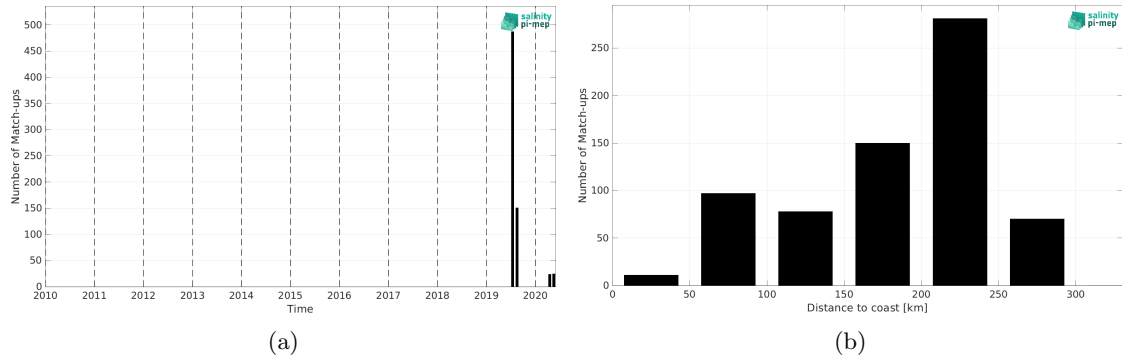
Figure 1: Number of match-ups between TSG (Lauge-Koch) and CCI SSS L4 POLAR NH Merged-OI v4.4 - 30-day running (ESA) SSS as a function of time (a) and as function of the distance to coast (b) over the Arctic Ocean Pi-MEP region and for the full satellite product period.
