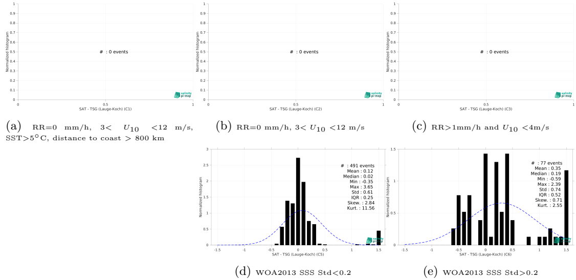
Figure 13: Normalized histogram of \Delta SSS (CCI SSS L4 POLAR NH Merged-OI v4.4 - 30-day running (ESA) - TSG (Lauge-Koch)) for 5 different subdatasets corresponding to: RR=0 mm/h, 3 < U_{10} < 12 m/s, SST>5°C, distance to coast > 800 km (a), RR=0 mm/h, 3 < U_{10} < 12 m/s (b), RR>1mm/h and U_{10} < 4 m/s (c), WOA2013 SSS Std<0.2 (d), WOA2013 SSS Std>0.2 (e).
