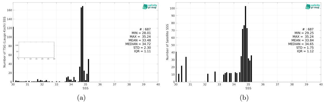
Figure 2: Histograms of SSS from TSG (Lauge-Koch) (a) and CCI SSS L4 POLAR NH Merged-OI v4.4 - 30-day running (ESA) (b) considering all match-up pairs per bins of 0.1 over the Arctic Ocean Pi-MEP region and for the full satellite product period.
