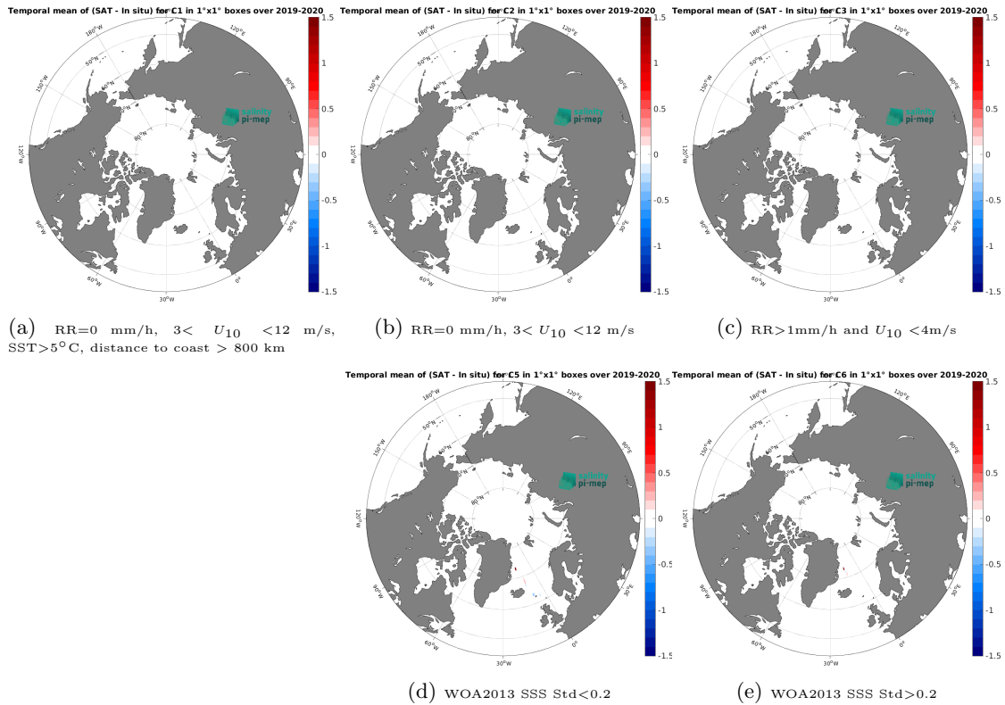
Figure 12: Temporal mean gridded over spatial boxes of size 1^{\circ}\times 1^{\circ} of \Delta\text{SSS} (CCI SSS L4 POLAR NH Merged-OI v4.4 - 30-day running (ESA) - TSG (Lauge-Koch)) for 5 different subdatasets corresponding to:RR=0 mm/h, 3 < U_{10} < 12 m/s, SST >5^{\circ}\text{C} , distance to coast > 800 km (a), RR=0 mm/h, 3 < U_{10} < 12 m/s (b), RR >1 mm/h and U_{10} < 4 m/s (c), WOA2013 SSS Std <0.2 (d), WOA2013 SSS Std >0.2 (e).
