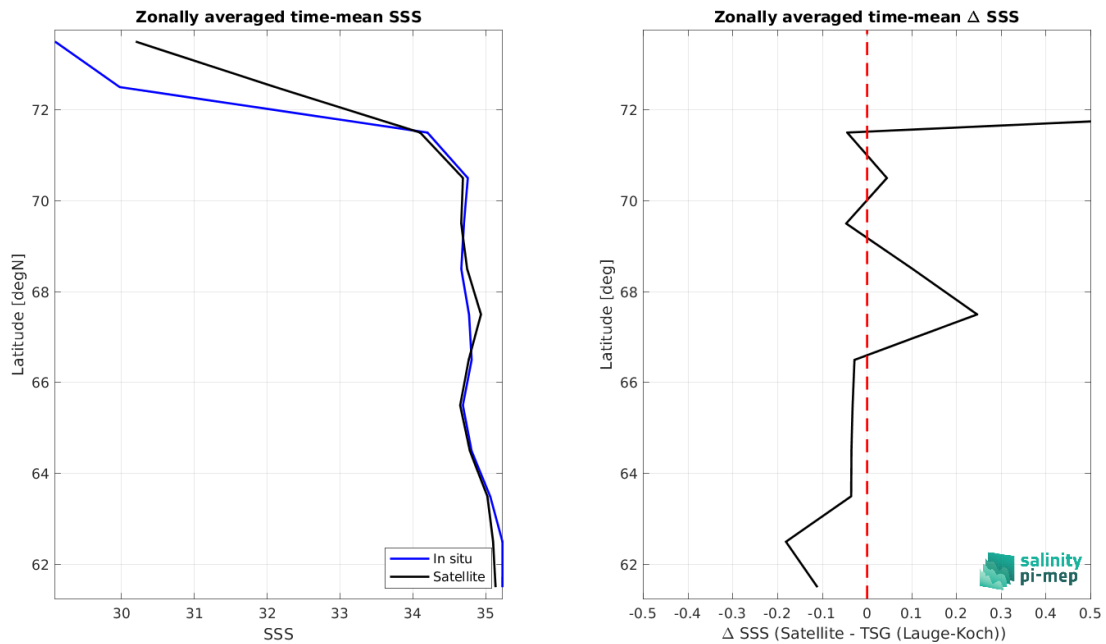
Figure 8: Left panel: Zonal mean SSS from CCI SSS L4 POLAR NH Merged-OI v4.4 - 30-day running (ESA) satellite product (black) and from TSG (Lauge-Koch) (blue). Right panel: Zonal mean of \Delta SSS (Satellite - TSG (Lauge-Koch)) for all the collected Pi-MEP match-up pairs estimated over the full satellite product period.
