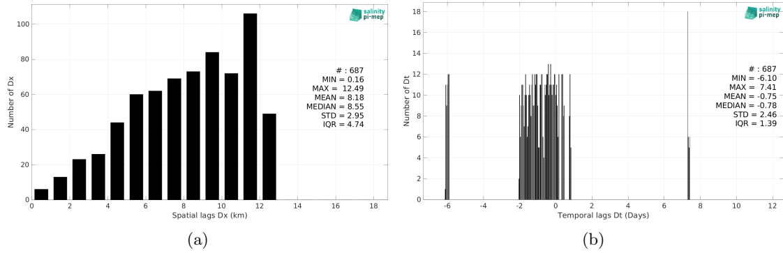
Figure 5: Histograms of the spatial (a) and temporal (b) lags between the location/time of the TSG (Lauge-Koch) measurement and the date of the corresponding CCI SSS L4 POLAR NH Merged-OI v4.4 - 30-day running (ESA) SSS pixel.
