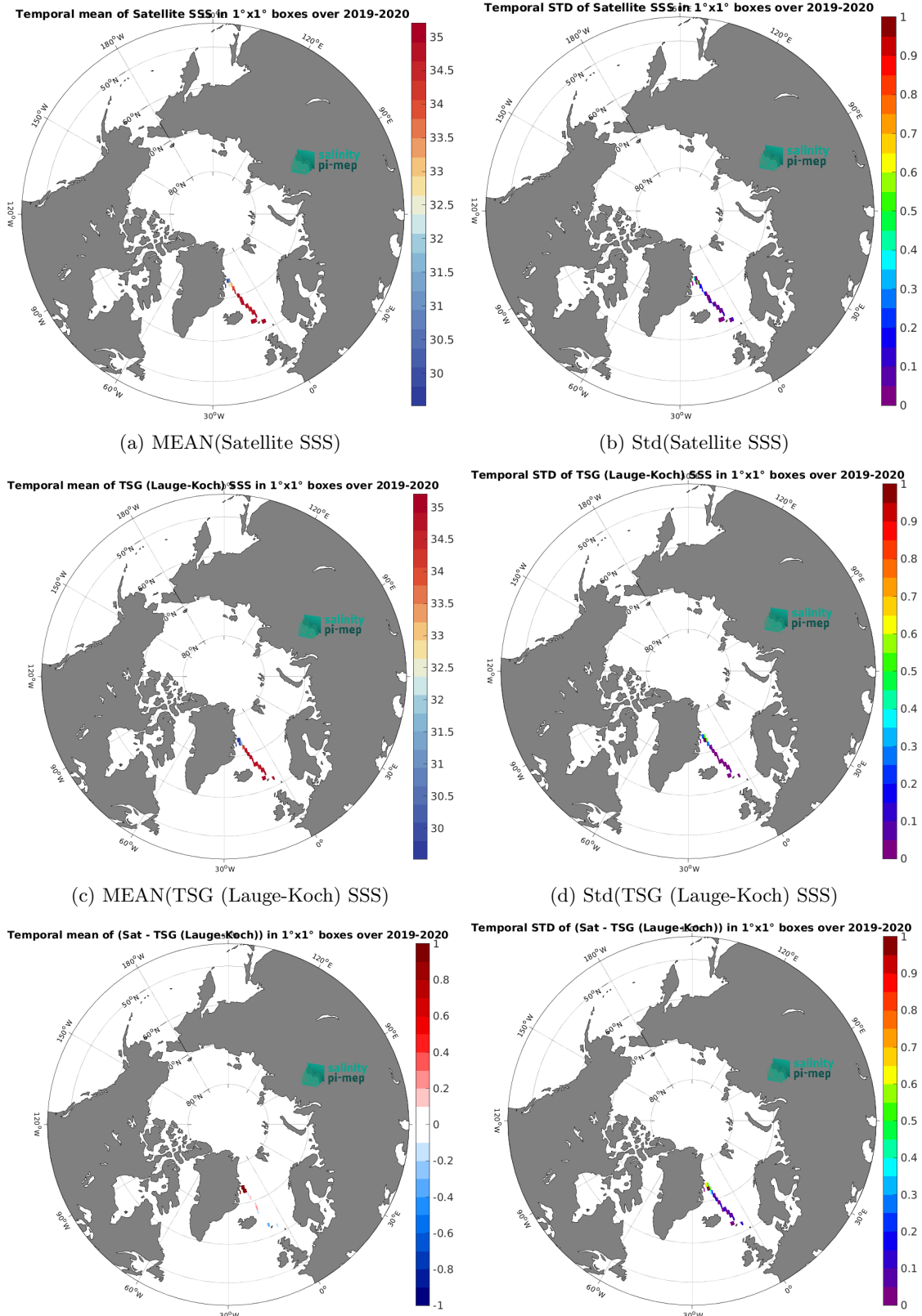
Figure 6: Temporal mean (left) and Std (right) of SSS from CCI SSS L4 POLAR NH Merged-OI v4.4 - 30-day running (ESA) (top), TSG (Lauge-Koch) (middle), and of \Delta SSS (Satellite - TSG (Lauge-Koch)). Only match-up pairs are used to generate these maps.
