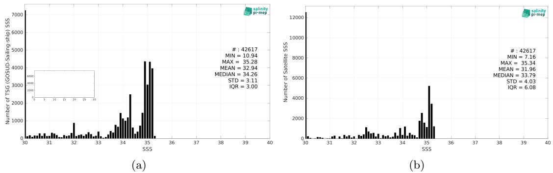
Figure 2: Histograms of SSS from TSG (GOSUD-Sailing-ship) (a) and CCI SSS L4 POLAR NH Merged-OI v4.4 - 30-day running (ESA) (b) considering all match-up pairs per bins of 0.1 over the Arctic Ocean Pi-MEP region and for the full satellite product period.
