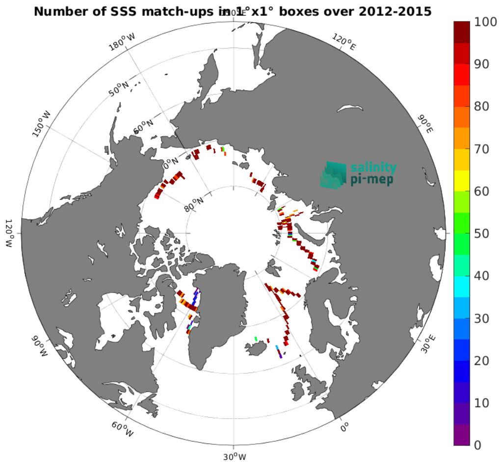
Figure 4: Number of SSS match-ups between TSG (GOSUD-Sailing-ship) SSS and the CCI SSS L4 POLAR NH Merged-OI v4.4 - 30-day running (ESA) SSS product for the Arctic Ocean Pi-MEP region over 1^\circ \times 1^\circ boxes and for the full satellite product period.
