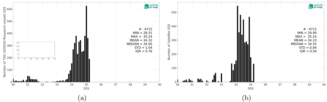
Figure 2: Histograms of SSS from TSG (GOSUD-Research-vessel) (a) and CCI SSS L4 POLAR NH Merged-OI v4.4 - 30-day running (ESA) (b) considering all match-up pairs per bins of 0.1 over the Arctic Ocean Pi-MEP region and for the full satellite product period.
