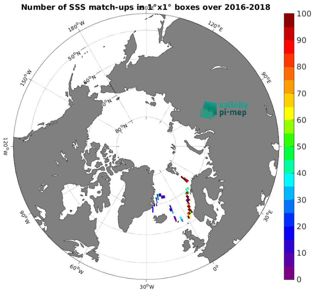
Figure 4: Number of SSS match-ups between TSG (GOSUD-Research-vessel) SSS and the CCI SSS L4 POLAR NH Merged-OI v4.4 - 30-day running (ESA) SSS product for the Arctic Ocean Pi-MEP region over 1^{\circ} \times 1^{\circ} boxes and for the full satellite product period.
