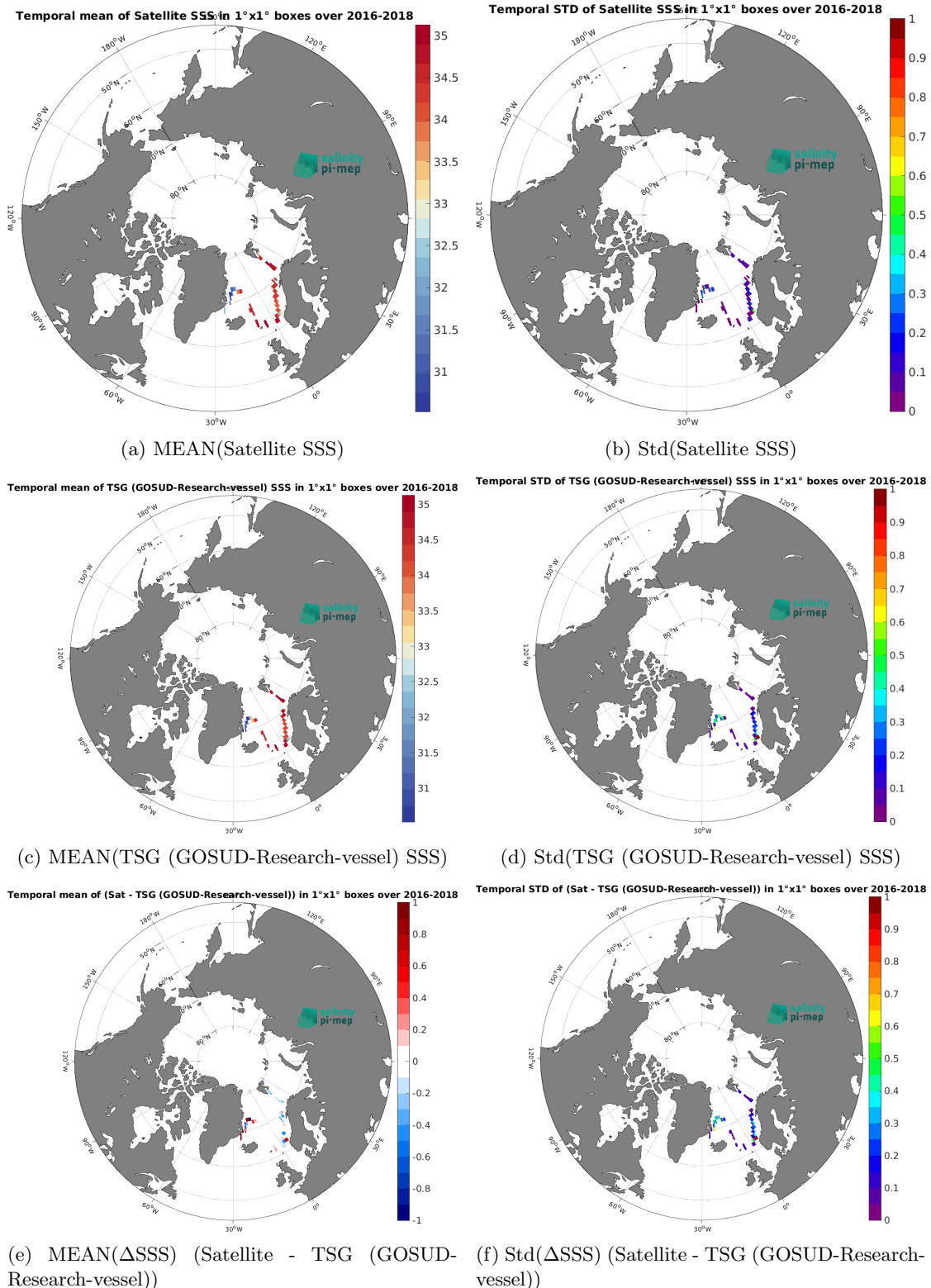
Figure 6: Temporal mean (left) and Std (right) of SSS from CCI SSS L4 POLAR NH Merged-OI v4.4 - 30-day running (ESA) (top), TSG (GOSUD-Research-vessel) (middle), and of \Delta SSS (Satellite - TSG (GOSUD-Research-vessel)). Only match-up pairs are used to generate these maps.
