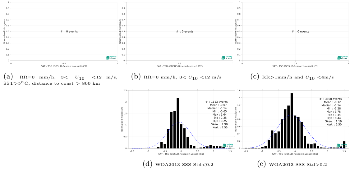
Figure 13: Normalized histogram of \Delta SSS (CCI SSS L4 POLAR NH Merged-OI v4.4 - 30-day running (ESA) - TSG (GOSUD-Research-vessel)) for 5 different subdatasets corresponding to: RR=0 mm/h, 3 < U_{10} < 12 m/s, SST>5°C, distance to coast > 800 km (a), RR=0 mm/h, 3 < U_{10} < 12 m/s (b), RR>1mm/h and U_{10} < 4 m/s (c), WOA2013 SSS Std<0.2 (d), WOA2013 SSS Std>0.2 (e).
