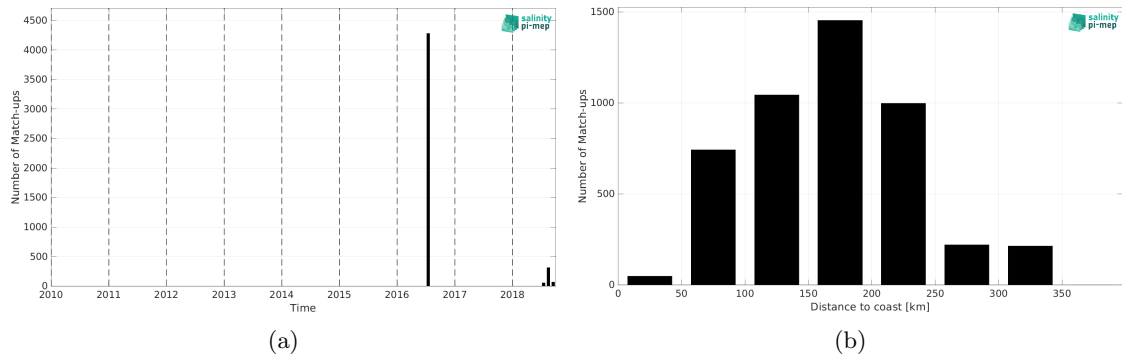
Figure 1: Number of match-ups between TSG (GOSUD-Research-vessel) and CCI SSS L4 POLAR NH Merged-OI v4.4 - 30-day running (ESA) SSS as a function of time (a) and as function of the distance to coast (b) over the Arctic Ocean Pi-MEP region and for the full satellite product period.
