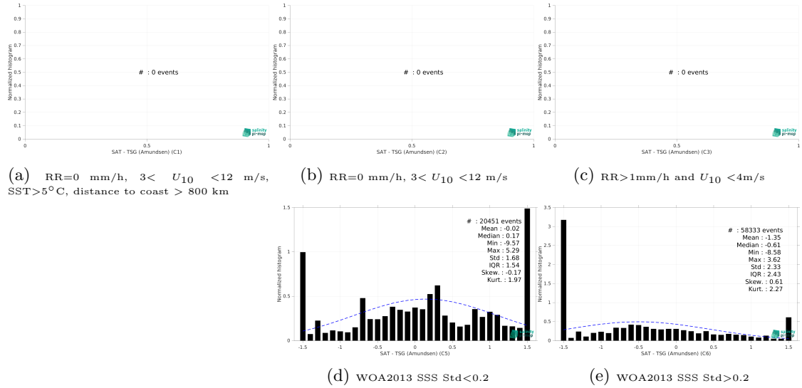
Figure 13: Normalized histogram of \Delta SSS (CCI SSS L4 POLAR NH Merged-OI v4.4 - 30-day running (ESA) - TSG (Amundsen)) for 5 different subdatasets corresponding to: RR=0 mm/h, 3 < U_{10} < 12 m/s, SST > 5°C, distance to coast > 800 km (a), RR=0 mm/h, 3 < U_{10} < 12 m/s (b), RR > 1mm/h and U_{10} < 4 m/s (c), WOA2013 SSS Std < 0.2 (d), WOA2013 SSS Std > 0.2 (e).
