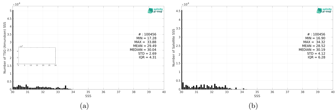
Figure 2: Histograms of SSS from TSG (Amundsen) (a) and CCI SSS L4 POLAR NH Merged-OI v4.4 - 30-day running (ESA) (b) considering all match-up pairs per bins of 0.1 over the Arctic Ocean Pi-MEP region and for the full satellite product period.
