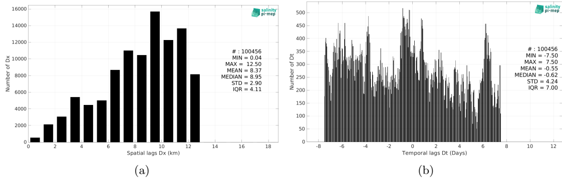
Figure 5: Histograms of the spatial (a) and temporal (b) lags between the location/time of the TSG (Amundsen) measurement and the date of the corresponding CCI SSS L4 POLAR NH Merged-OI v4.4 - 30-day running (ESA) SSS pixel.
