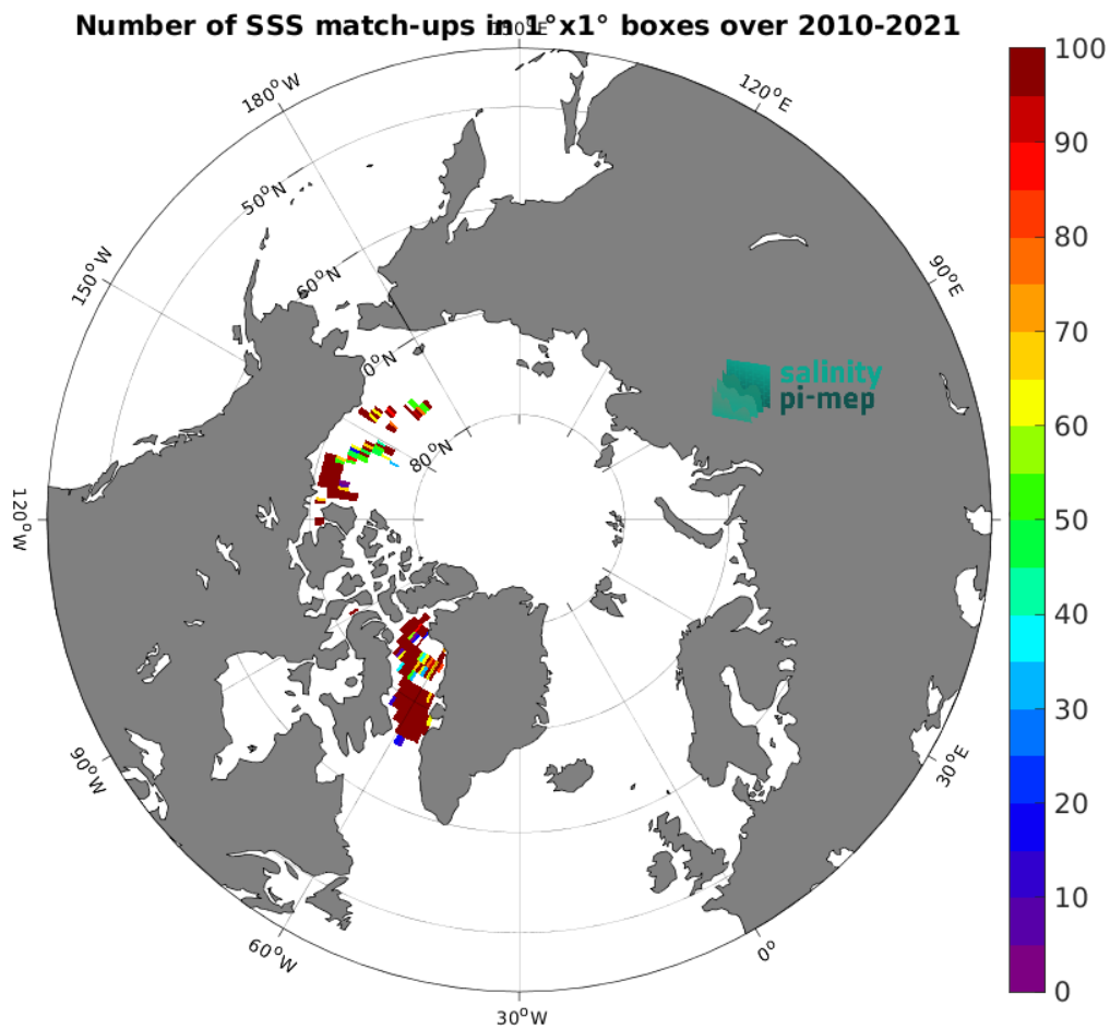
Figure 4: Number of SSS match-ups between TSG (Amundsen) SSS and the CCI SSS L4 POLAR NH Merged-OI v4.4 - 30-day running (ESA) SSS product for the Arctic Ocean Pi-MEP region over 1^{\circ} \times 1^{\circ} boxes and for the full satellite product period.
