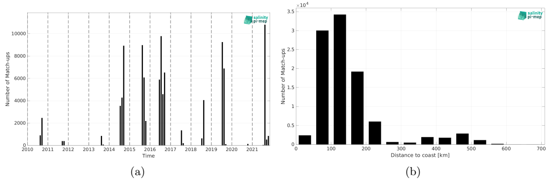
Figure 1: Number of match-ups between TSG (Amundsen) and CCI SSS L4 POLAR NH Merged-OI v4.4 - 30-day running (ESA) SSS as a function of time (a) and as function of the distance to coast (b) over the Arctic Ocean Pi-MEP region and for the full satellite product period.
