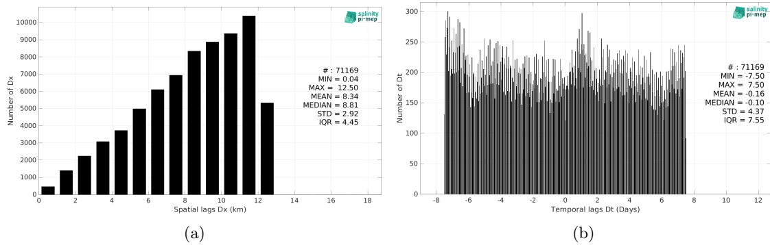
Figure 5: Histograms of the spatial (a) and temporal (b) lags between the location/time of the Saildrone measurement and the date of the corresponding CCI SSS L4 POLAR NH Merged-OI v4.4 - 30-day running (ESA) SSS pixel.
