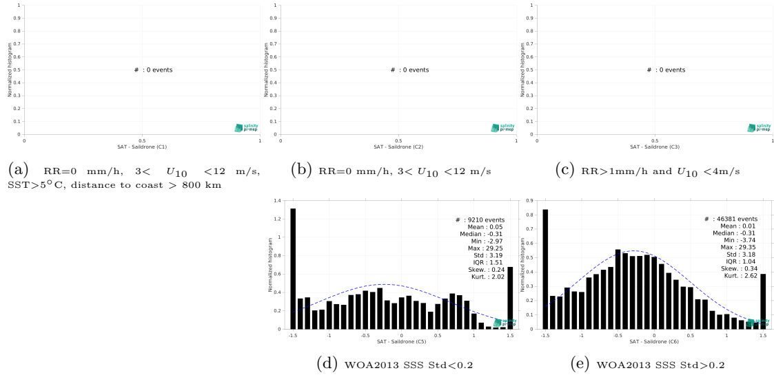
Figure 13: Normalized histogram of \Delta SSS (CCI SSS L4 POLAR NH Merged-OI v4.4 - 30-day running (ESA) - Sairdrone) for 5 different subdatasets corresponding to: RR=0 mm/h, 3 < U_{10} < 12 m/s, SST>5°C, distance to coast > 800 km (a), RR=0 mm/h, 3 < U_{10} < 12 m/s (b), RR>1mm/h and U_{10} < 4 m/s (c), WOA2013 SSS Std<0.2 (d), WOA2013 SSS Std>0.2 (e).
