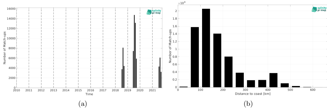
Figure 1: Number of match-ups between Saildrone and CCI SSS L4 POLAR NH Merged-OI v4.4 - 30-day running (ESA) SSS as a function of time (a) and as function of the distance to coast (b) over the Arctic Ocean Pi-MEP region and for the full satellite product period.
