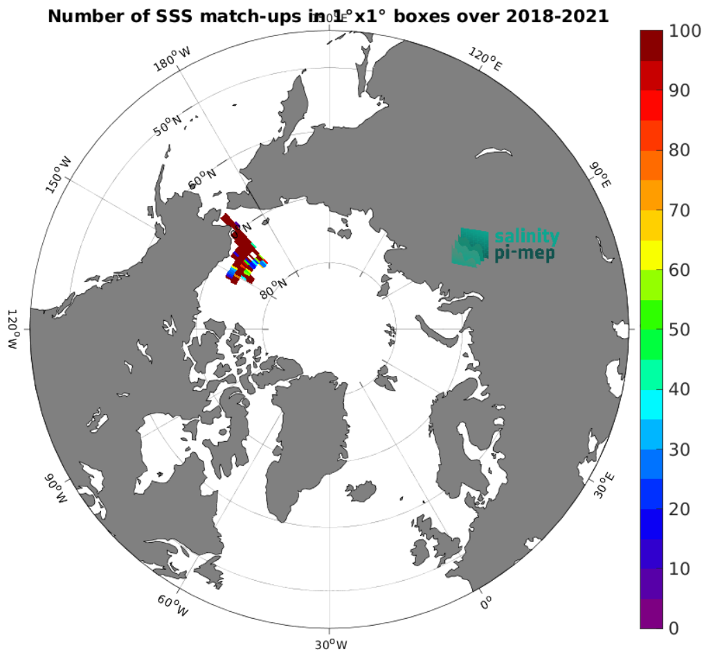
Figure 4: Number of SSS match-ups between Saildrone SSS and the CCI SSS L4 POLAR NH Merged-OI v4.4 - 30-day running (ESA) SSS product for the Arctic Ocean Pi-MEP region over 1^{\circ} \times 1^{\circ} boxes and for the full satellite product period.
