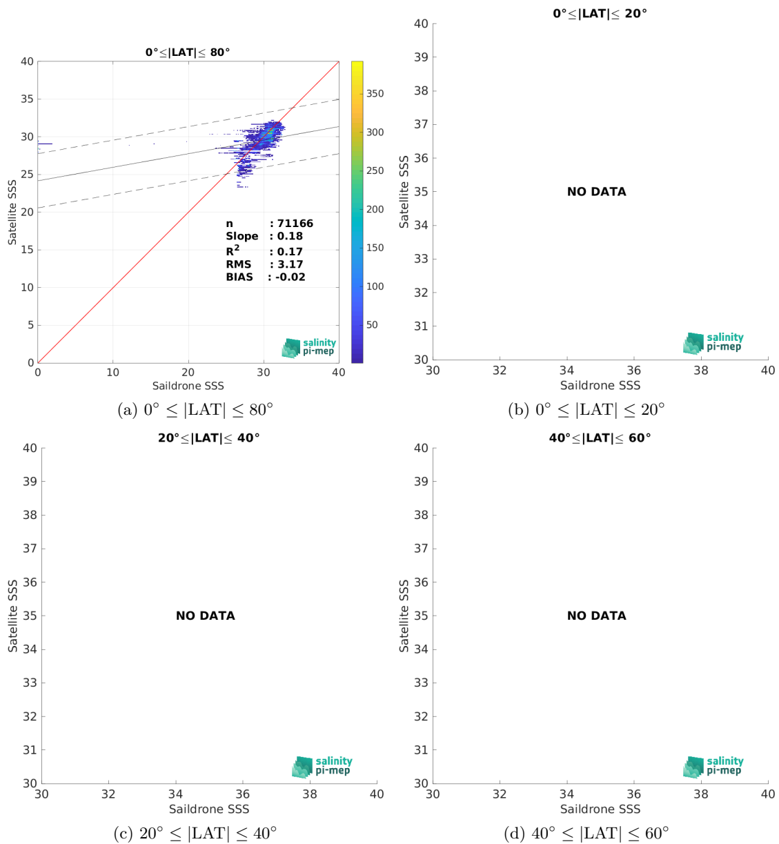
Figure 9: Contour maps of the concentration of CCI SSS L4 POLAR NH Merged-OI v4.4 - 30-day running (ESA) SSS (y-axis) versus Saildrone SSS (x-axis) at match-up pairs for different latitude bands. For each plot, the red line shows x=y . The black thin and dashed lines indicate a linear fit through the data cloud and the \pm 95\% confidence levels, respectively. The number match-up pairs n , the slope and R^2 coefficient of the linear fit, the root mean square (RMS) and the mean bias between satellite and in situ data are indicated for each latitude band in each plots.
