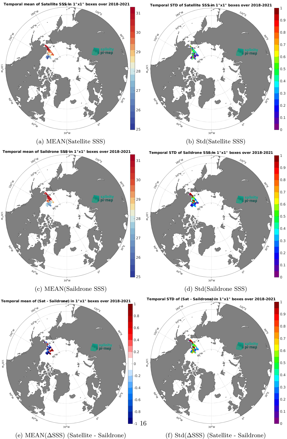
Figure 6: Temporal mean (left) and Std (right) of SSS from CCI SSS L4 POLAR NH Merged-OI v4.4 - 30-day running (ESA) (top), Saildrone (middle), and of \Delta SSS (Satellite - Saildrone). Only match-up pairs are used to generate these maps.
