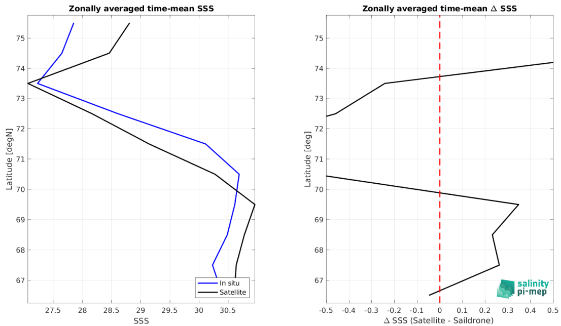
Figure 8: Left panel: Zonal mean SSS from CCI SSS L4 POLAR NH Merged-OI v4.4 - 30-day running (ESA) satellite product (black) and from Sairdron (blue). Right panel: Zonal mean of \Delta SSS (Satellite - Sairdron) for all the collected Pi-MEP match-up pairs estimated over the full satellite product period.
