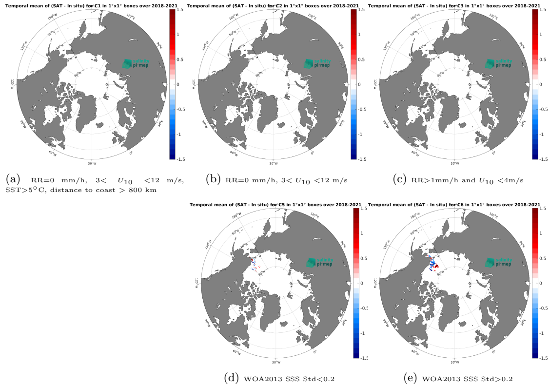
Figure 12: Temporal mean gridded over spatial boxes of size 1^{\circ}\times 1^{\circ} of \Delta\text{SSS} (CCI SSS L4 POLAR NH Merged-OI v4.4 - 30-day running (ESA) - Saildrone) for 5 different subdatasets corresponding to:RR=0 mm/h, 3 < U_{10} < 12 m/s, SST >5^{\circ}\text{C} , distance to coast > 800 km (a), RR=0 mm/h, 3 < U_{10} < 12 m/s (b), RR >1 mm/h and U_{10} < 4 m/s (c), WOA2013 SSS Std <0.2 (d), WOA2013 SSS Std >0.2 (e).
