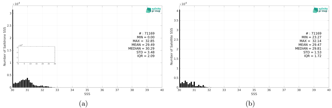
Figure 2: Histograms of SSS from Saildrone (a) and CCI SSS L4 POLAR NH Merged-OI v4.4 - 30-day running (ESA) (b) considering all match-up pairs per bins of 0.1 over the Arctic Ocean Pi-MEP region and for the full satellite product period.
