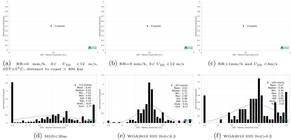
Figure 13: Normalized histogram of \Delta SSS (CCI SSS L4 POLAR NH Merged-OI v4.4 - 30-day running (ESA) - Marine mammals) for 6 different subdatasets corresponding to: RR=0 mm/h, 3 < U_{10} < 12 m/s, SST>5°C, distance to coast > 800 km (a), RR=0 mm/h, 3 < U_{10} < 12 m/s (b), RR>1mm/h and U_{10} < 4 m/s (c), MLD<20m (d), WOA2013 SSS Std<0.2 (e), WOA2013 SSS Std>0.2 (f).
