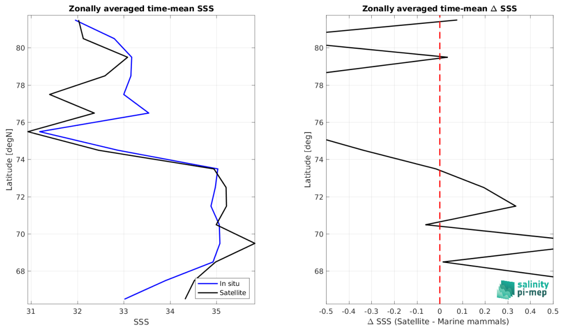
Figure 8: Left panel: Zonal mean SSS from CCI SSS L4 POLAR NH Merged-OI v4.4 - 30-day running (ESA) satellite product (black) and from Marine mammals (blue). Right panel: Zonal mean of \Delta SSS (Satellite - Marine mammals) for all the collected Pi-MEP match-up pairs estimated over the full satellite product period.
