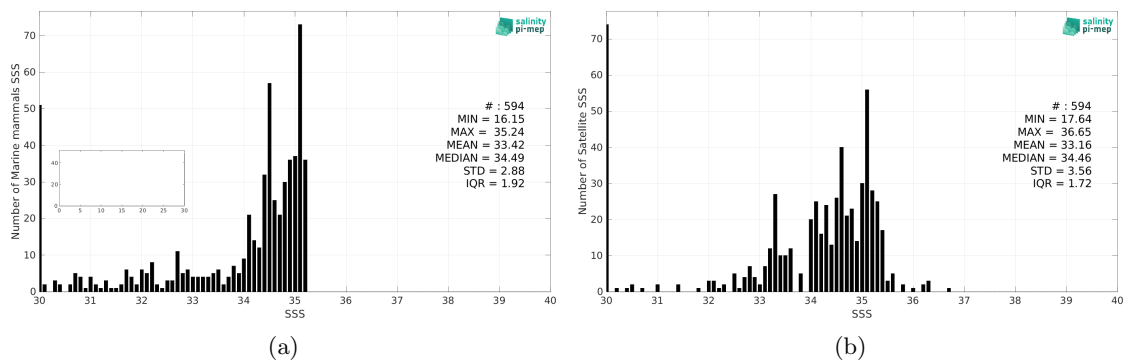
Figure 2: Histograms of SSS from Marine mammals (a) and CCI SSS L4 POLAR NH Merged-OI v4.4 - 30-day running (ESA) (b) considering all match-up pairs per bins of 0.1 over the Arctic Ocean Pi-MEP region and for the full satellite product period.
