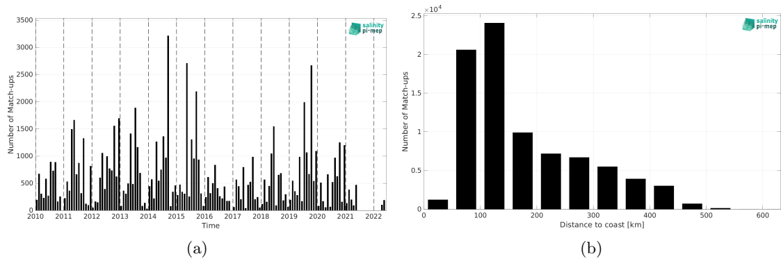
Figure 1: Number of match-ups between ICES and CCI SSS L4 POLAR NH Merged-OI v4.4 - 30-day running (ESA) SSS as a function of time (a) and as function of the distance to coast (b) over the Arctic Ocean Pi-MEP region and for the full satellite product period.
