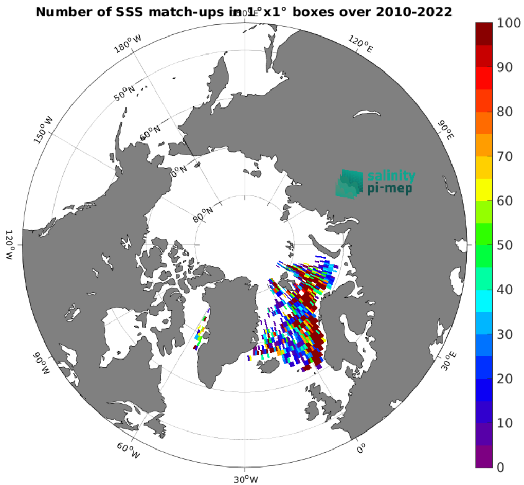
Figure 4: Number of SSS match-ups between ICES SSS and the CCI SSS L4 POLAR NH Merged-OI v4.4 - 30-day running (ESA) SSS product for the Arctic Ocean Pi-MEP region over 1^{\circ} \times 1^{\circ} boxes and for the full satellite product period.
