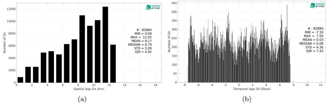
Figure 5: Histograms of the spatial (a) and temporal (b) lags between the location/time of the ICES measurement and the date of the corresponding CCI SSS L4 POLAR NH Merged-OI v4.4 - 30-day running (ESA) SSS pixel.
