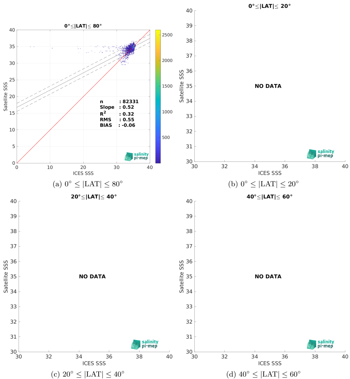
Figure 9: Contour maps of the concentration of CCI SSS L4 POLAR NH Merged-OI v4.4 - 30-day running (ESA) SSS (y-axis) versus ICES SSS (x-axis) at match-up pairs for different latitude bands. For each plot, the red line shows x=y . The black thin and dashed lines indicate a linear fit through the data cloud and the \pm 95\% confidence levels, respectively. The number match-up pairs n , the slope and R^2 coefficient of the linear fit, the root mean square (RMS) and the mean bias between satellite and in situ data are indicated for each latitude band in each plots.
