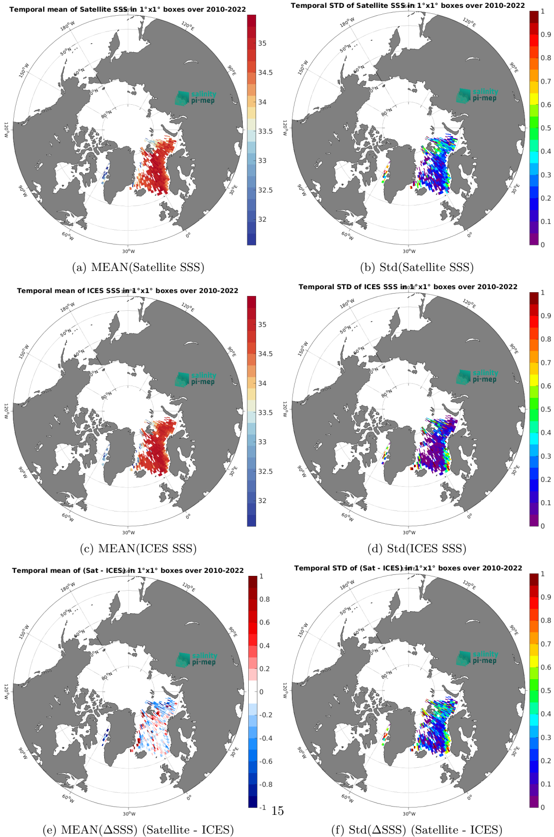
Figure 6: Temporal mean (left) and Std (right) of SSS from CCI SSS L4 POLAR NH Merged-OI v4.4 - 30-day running (ESA) (top), ICES (middle), and of \Delta SSS (Satellite - ICES). Only match-up pairs are used to generate these maps.
