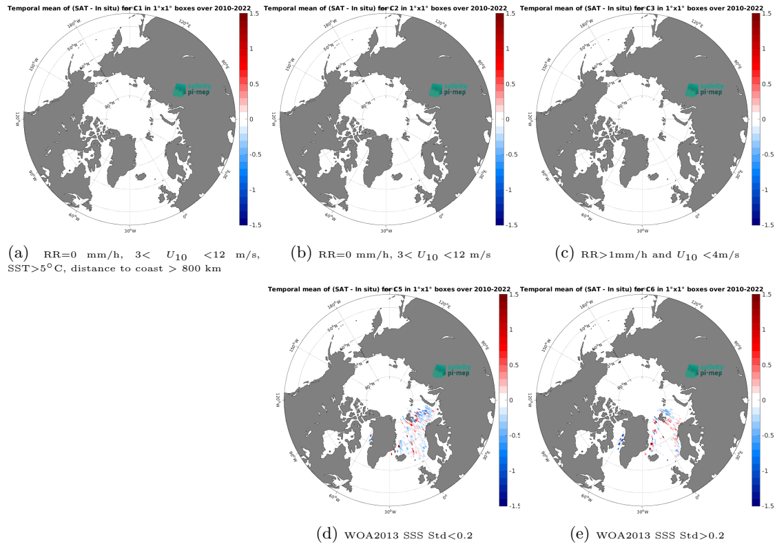
Figure 12: Temporal mean gridded over spatial boxes of size 1^{\circ}\times 1^{\circ} of \Delta\text{SSS} (CCI SSS L4 POLAR NH Merged-OI v4.4 - 30-day running (ESA) - ICES) for 5 different subdatasets corresponding to: RR=0 mm/h, 3 < U_{10} < 12 m/s, SST >5^{\circ}\text{C} , distance to coast > 800 km (a), RR=0 mm/h, 3 < U_{10} < 12 m/s (b), RR >1 mm/h and U_{10} < 4 m/s (c), WOA2013 SSS Std <0.2 (d), WOA2013 SSS Std >0.2 (e).
