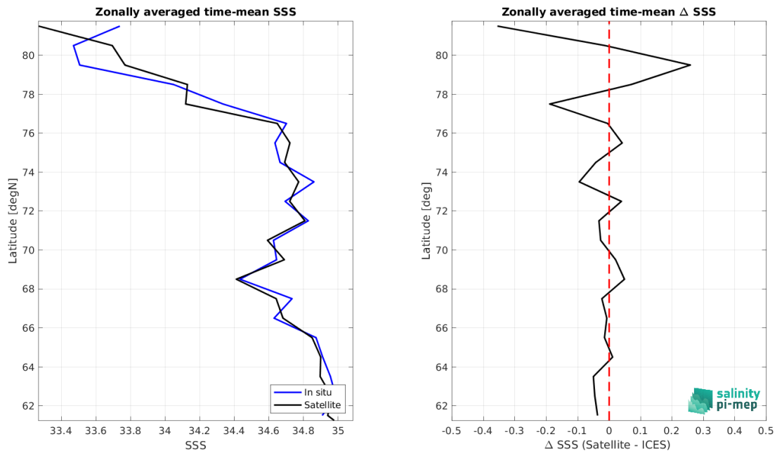
Figure 8: Left panel: Zonal mean SSS from CCI SSS L4 POLAR NH Merged-OI v4.4 - 30-day running (ESA) satellite product (black) and from ICES (blue). Right panel: Zonal mean of \Delta SSS (Satellite - ICES) for all the collected Pi-MEP match-up pairs estimated over the full satellite product period.
