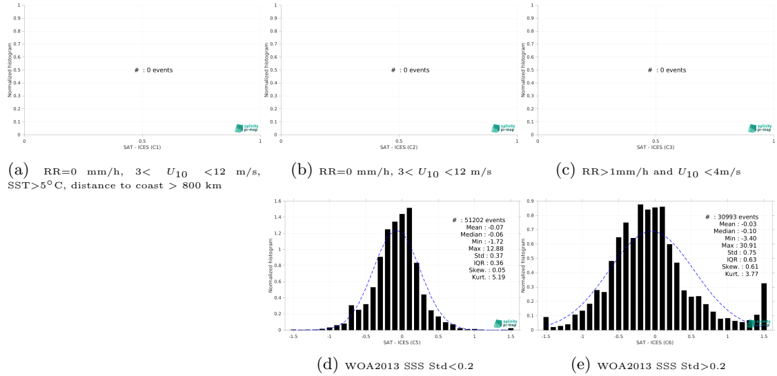
Figure 13: Normalized histogram of \Delta SSS (CCI SSS L4 POLAR NH Merged-OI v4.4 - 30-day running (ESA) - ICES) for 5 different subdatasets corresponding to: RR=0 mm/h, 3 < U_{10} < 12 m/s, SST>5°C, distance to coast > 800 km (a), RR=0 mm/h, 3 < U_{10} < 12 m/s (b), RR>1mm/h and U_{10} < 4 m/s (c), WOA2013 SSS Std<0.2 (d), WOA2013 SSS Std>0.2 (e).
