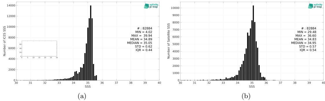
Figure 2: Histograms of SSS from ICES (a) and CCI SSS L4 POLAR NH Merged-OI v4.4 - 30-day running (ESA) (b) considering all match-up pairs per bins of 0.1 over the Arctic Ocean Pi-MEP region and for the full satellite product period.
