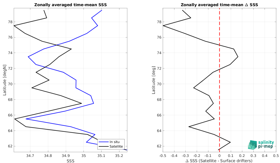
Figure 7: Left panel: Zonal mean SSS from CCI SSS L4 POLAR NH Merged-OI v4.4 - 30-day running (ESA) satellite product (black) and from Surface drifters (blue). Right panel: Zonal mean of \Delta SSS (Satellite - Surface drifters) for all the collected Pi-MEP match-up pairs estimated over the full satellite product period.
