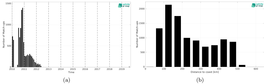
Figure 1: Number of match-ups between Surface drifters and CCI SSS L4 POLAR NH Merged-OI v4.4 - 30-day running (ESA) SSS as a function of time (a) and as function of the distance to coast (b) over the Arctic Ocean Pi-MEP region and for the full satellite product period.
