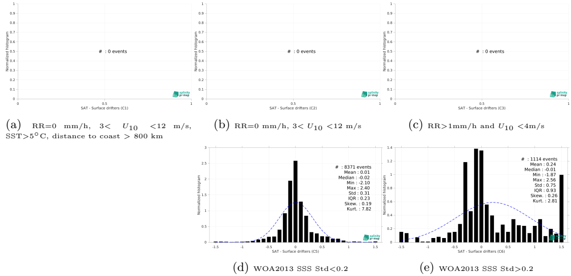
Figure 12: Normalized histogram of \Delta SSS (CCI SSS L4 POLAR NH Merged-OI v4.4 - 30-day running (ESA) - Surface drifters) for 5 different subdatasets corresponding to: RR=0 mm/h, 3 < U_{10} < 12 m/s, SST>5°C, distance to coast > 800 km (a), RR=0 mm/h, 3 < U_{10} < 12 m/s (b), RR>1mm/h and U_{10} < 4 m/s (c), WOA2013 SSS Std<0.2 (d), WOA2013 SSS Std>0.2 (e).
