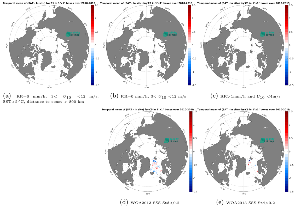
Figure 11: Temporal mean gridded over spatial boxes of size 1^{\circ}\times 1^{\circ} of \Delta\text{SSS} (CCI SSS L4 POLAR NH Merged-OI v4.4 - 30-day running (ESA) - Surface drifters) for 5 different subdatasets corresponding to:RR=0 mm/h, 3 < U_{10} < 12 m/s, SST >5^{\circ}\text{C} , distance to coast > 800 km (a), RR=0 mm/h, 3 < U_{10} < 12 m/s (b), RR >1 mm/h and U_{10} < 4 m/s (c), WOA2013 SSS Std <0.2 (d), WOA2013 SSS Std >0.2 (e).
