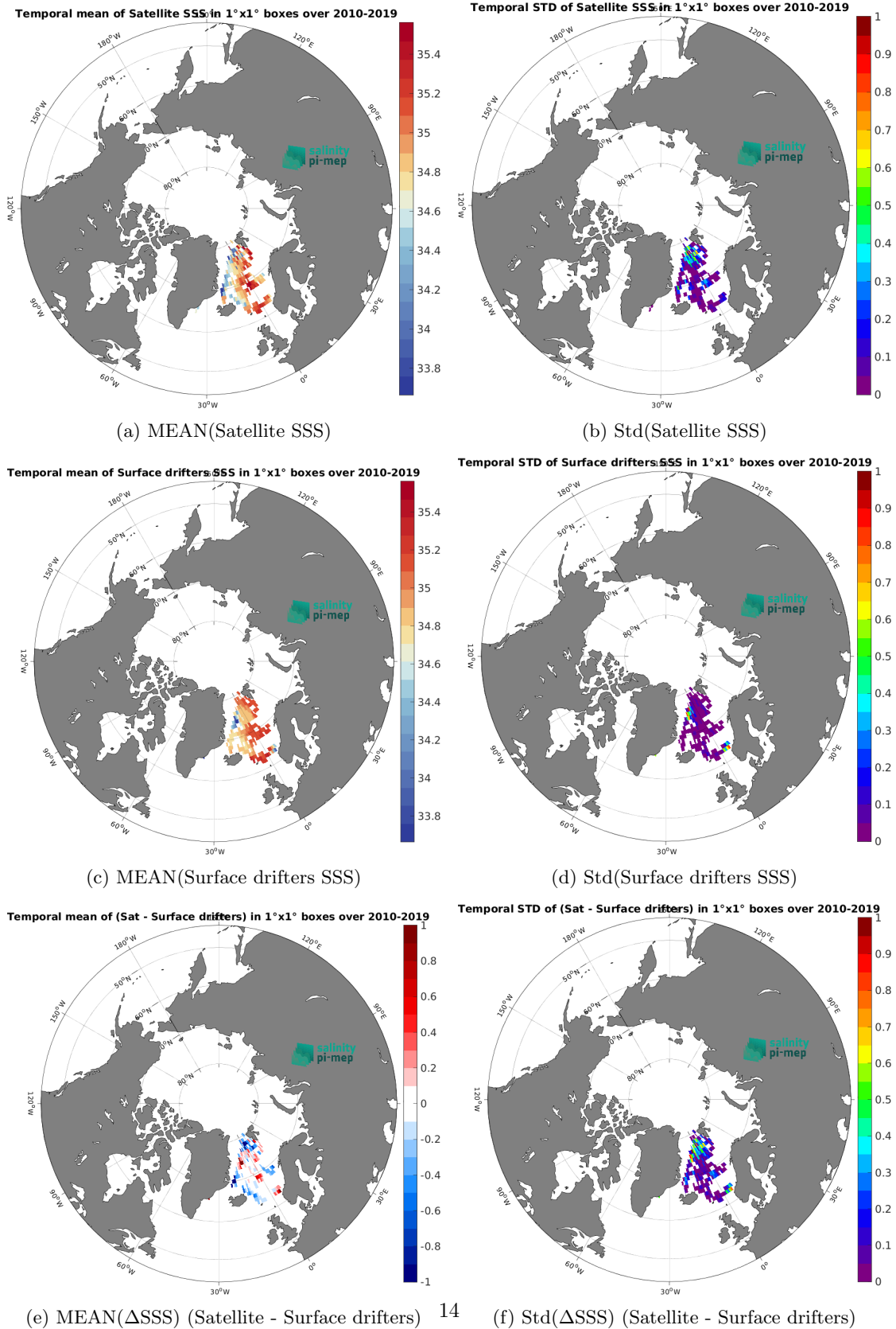
Figure 5: Temporal mean (left) and Std (right) of SSS from CCI SSS L4 POLAR NH Merged-OI v4.4 - 30-day running (ESA) (top), Surface drifters (middle), and of \Delta SSS (Satellite - Surface drifters). Only match-up pairs are used to generate these maps.
