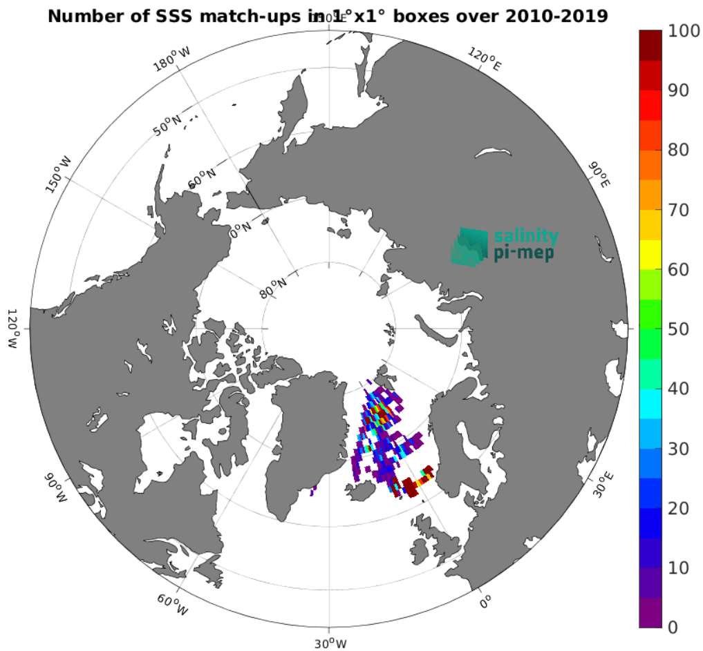
Figure 3: Number of SSS match-ups between Surface drifters SSS and the CCI SSS L4 POLAR NH Merged-OI v4.4 - 30-day running (ESA) SSS product for the Arctic Ocean Pi-MEP region over 1^{\circ} \times 1^{\circ} boxes and for the full satellite product period.
