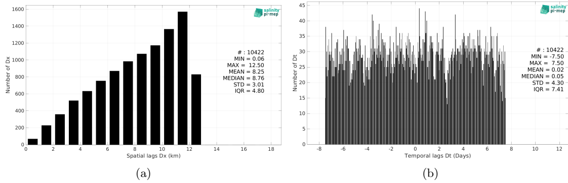
Figure 4: Histograms of the spatial (a) and temporal (b) lags between the location/time of the Surface drifters measurement and the date of the corresponding CCI SSS L4 POLAR NH Merged-OI v4.4 - 30-day running (ESA) SSS pixel.
