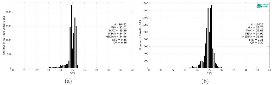
Figure 2: Histograms of SSS from Surface drifters (a) and CCI SSS L4 POLAR NH Merged-OI v4.4 - 30-day running (ESA) (b) considering all match-up pairs per bins of 0.1 over the Arctic Ocean Pi-MEP region and for the full satellite product period.
