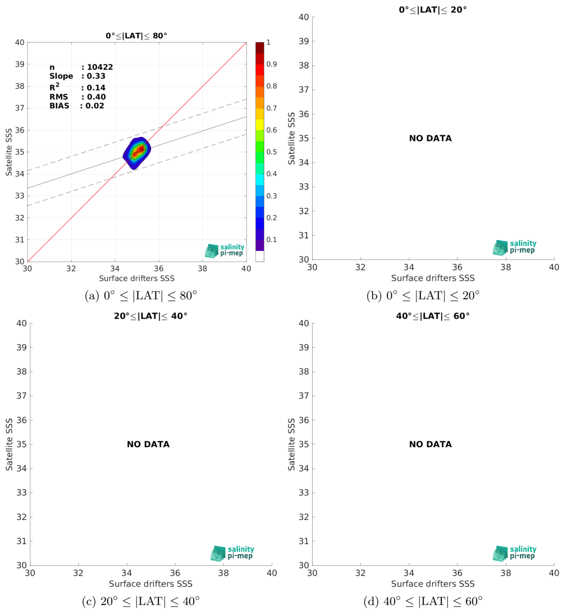
Figure 8: Contour maps of the concentration of CCI SSS L4 POLAR NH Merged-OI v4.4 - 30-day running (ESA) SSS (y-axis) versus Surface drifters SSS (x-axis) at match-up pairs for different latitude bands. For each plot, the red line shows x=y . The black thin and dashed lines indicate a linear fit through the data cloud and the \pm 95\% confidence levels, respectively. The number match-up pairs n , the slope and R^2 coefficient of the linear fit, the root mean square (RMS) and the mean bias between satellite and in situ data are indicated for each latitude band in each plots.
