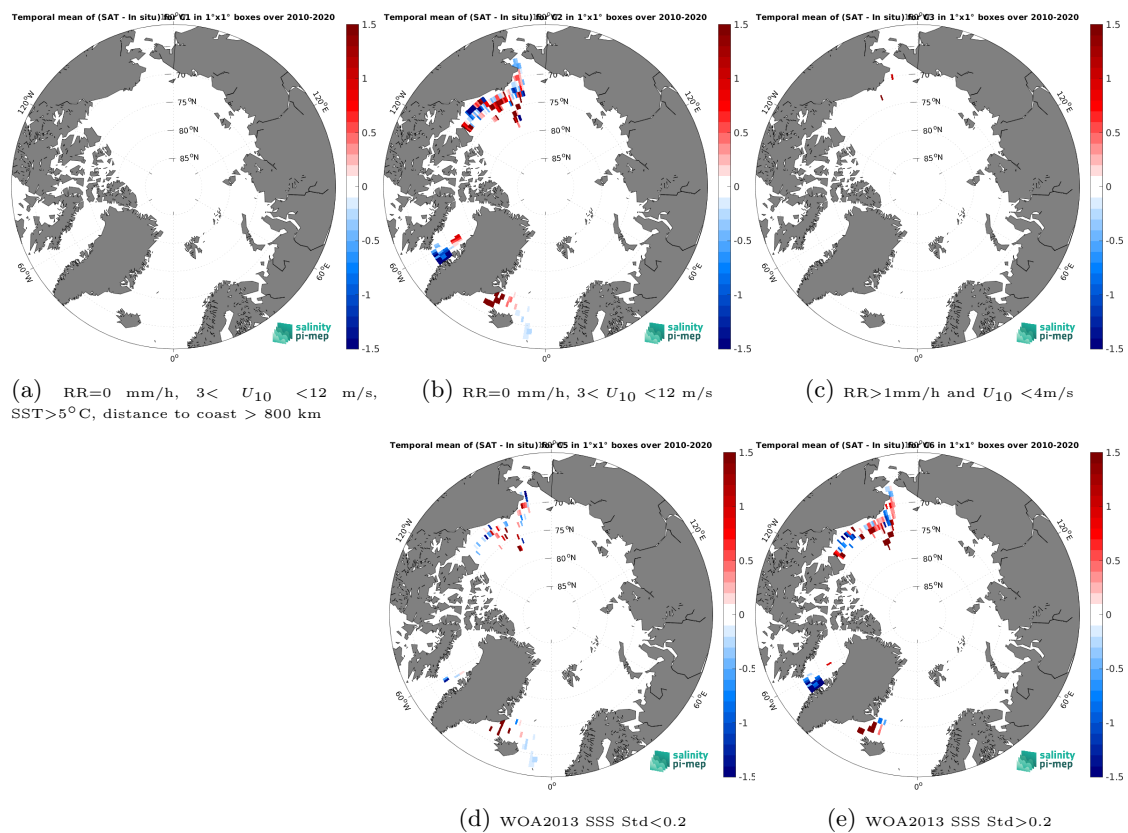
Figure 14: Temporal mean gridded over spatial boxes of size 1^\circ \times 1^\circ of \Delta\text{SSS} (CCI SSS L4 Merged-OI v5.5 - 7-day running (ESA) - TSG (SAMOS)) for 5 different subdatasets corresponding to: RR=0 mm/h, 3 < U_{10} < 12 m/s, SST > 5^\circ\text{C} , distance to coast > 800 km (a), RR=0 mm/h, 3 < U_{10} < 12 m/s (b), RR > 1 mm/h and U_{10} < 4 m/s (c), WOA2013 SSS Std < 0.2 (d), WOA2013 SSS Std > 0.2 (e).
