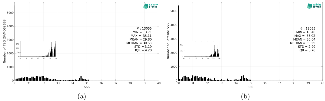
Figure 3: Histograms of SSS from TSG (SAMOS) (a) and CCI SSS L4 Merged-OI v5.5 - 7-day running (ESA) (b) considering all match-up pairs per bins of 0.1 over the Arctic Ocean Pi-MEP region and for the full satellite product period.
