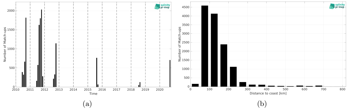
Figure 2: Number of match-ups between TSG (SAMOS) and CCI SSS L4 Merged-OI v5.5 - 7-day running (ESA) SSS as a function of time (a) and as function of the distance to coast (b) over the Arctic Ocean Pi-MEP region and for the full satellite product period.
