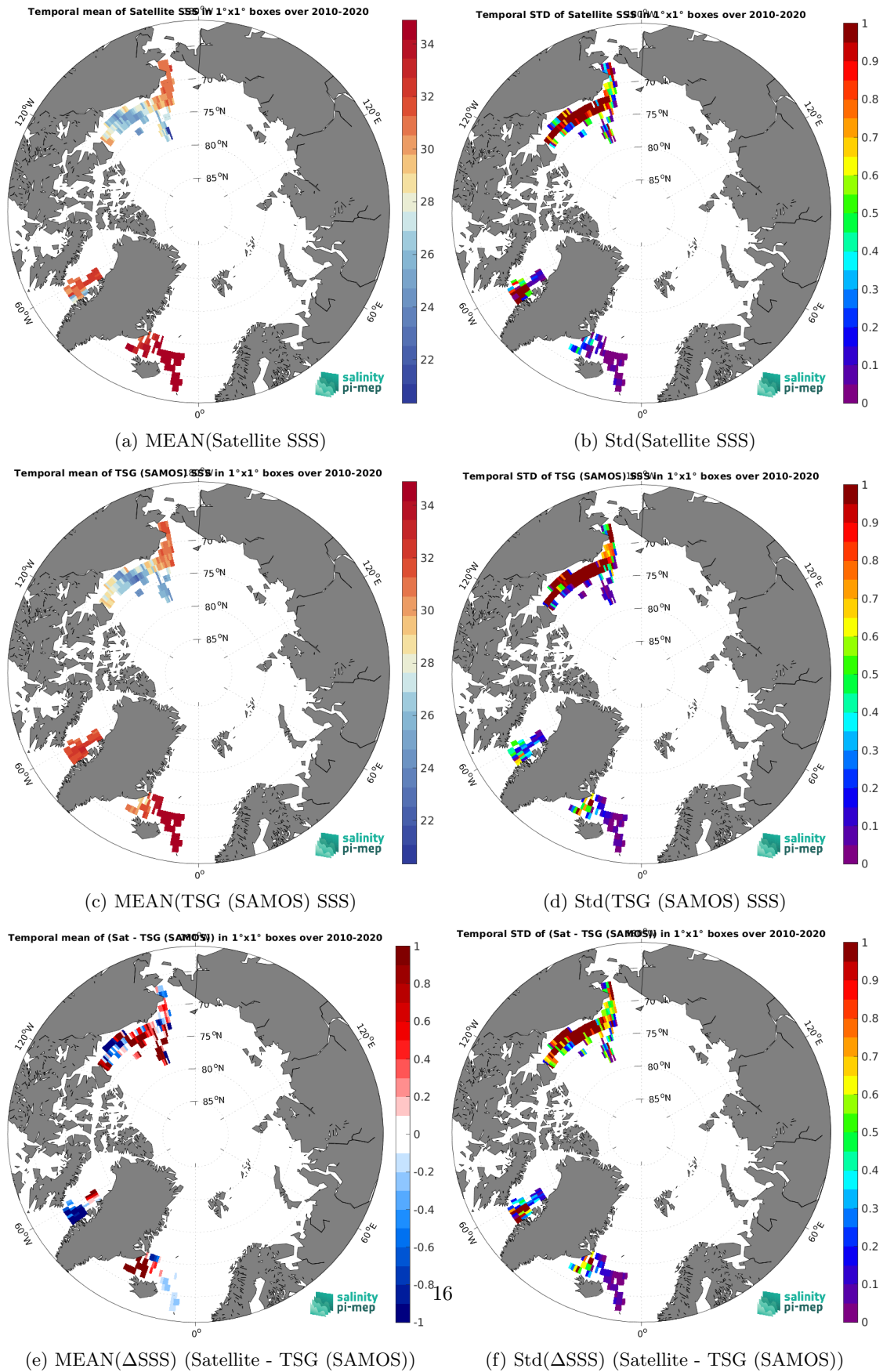
Figure 7: Temporal mean (left) and Std (right) of SSS from CCI SSS L4 Merged-OI v5.5 - 7-day running (ESA) (top), TSG (SAMOS) (middle), and of \Delta SSS (Satellite - TSG (SAMOS)). Only match-up pairs are used to generate these maps.
