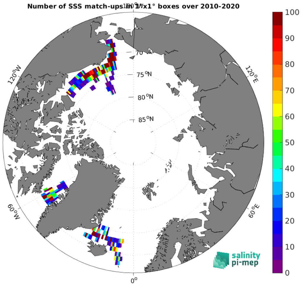
Figure 5: Number of SSS match-ups between TSG (SAMOS) SSS and the CCI SSS L4 Merged-OI v5.5 - 7-day running (ESA) SSS product for the Arctic Ocean Pi-MEP region over 1^\circ \times 1^\circ boxes and for the full satellite product period.
