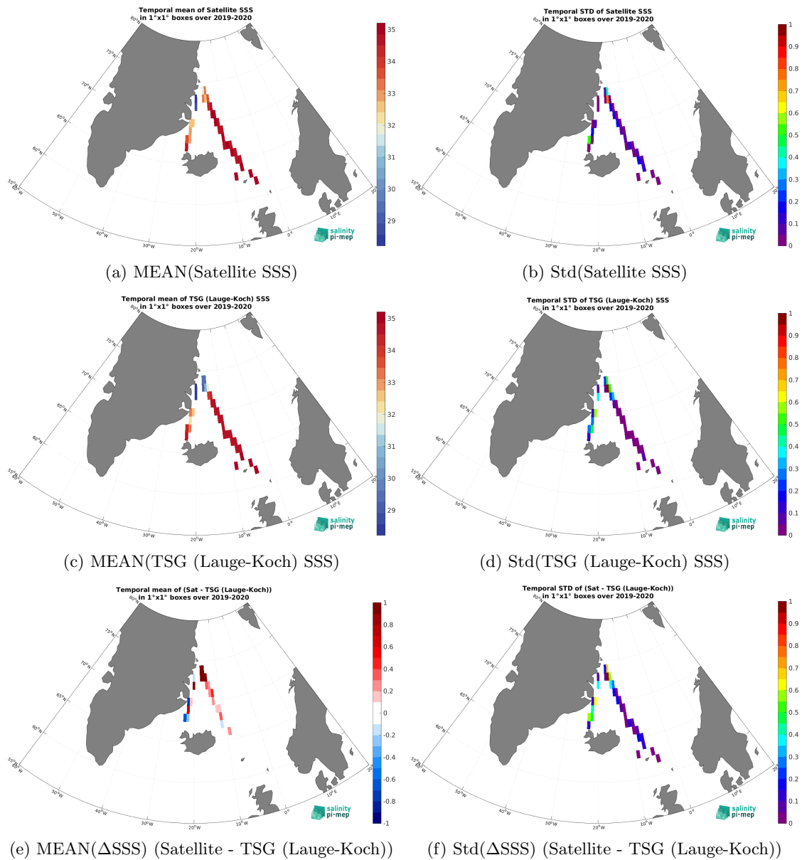
Figure 7: Temporal mean (left) and Std (right) of SSS from CCI SSS L4 Merged-OI v5.5 - 7-day running (ESA) (top), TSG (Lauge-Koch) (middle), and of \Delta SSS (Satellite - TSG (Lauge-Koch)). Only match-up pairs are used to generate these maps.
