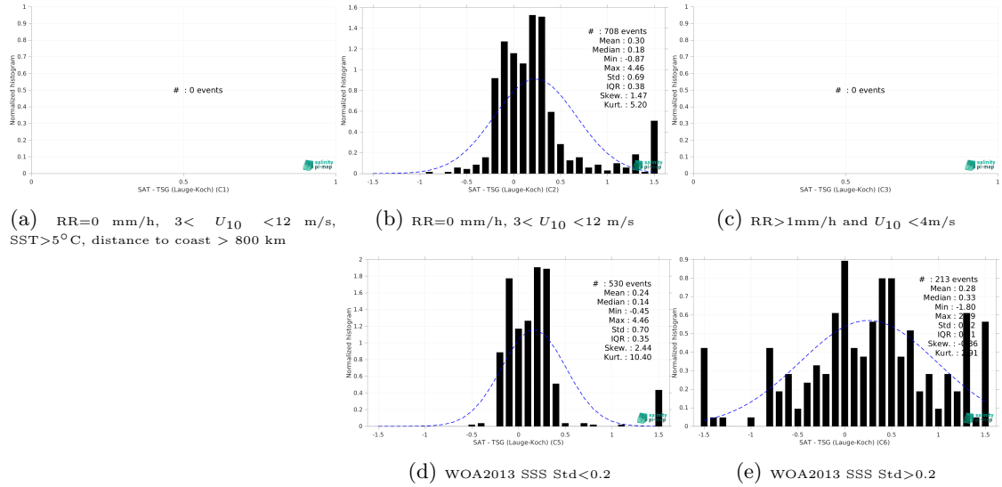
Figure 15: Normalized histogram of \Delta SSS (CCI SSS L4 Merged-OI v5.5 - 7-day running (ESA) - TSG (Lauge-Koch)) for 5 different subdatasets corresponding to: RR=0 mm/h, 3 < U_{10} < 12 m/s, SST > 5°C, distance to coast > 800 km (a), RR=0 mm/h, 3 < U_{10} < 12 m/s (b), RR > 1mm/h and U_{10} < 4 m/s (c), WOA2013 SSS Std < 0.2 (d), WOA2013 SSS Std > 0.2 (e).
