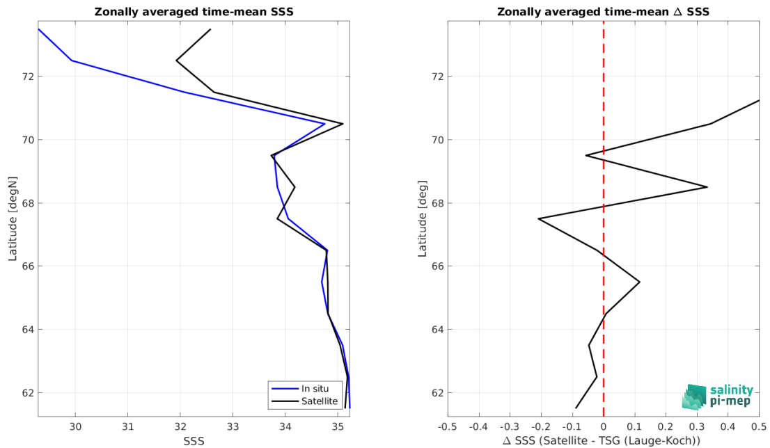
Figure 9: Left panel: Zonal mean SSS from CCI SSS L4 Merged-OI v5.5 - 7-day running (ESA) satellite product (black) and from TSG (Lauge-Koch) (blue). Right panel: Zonal mean of \Delta SSS (Satellite - TSG (Lauge-Koch)) for all the collected Pi-MEP match-up pairs estimated over the full satellite product period.
