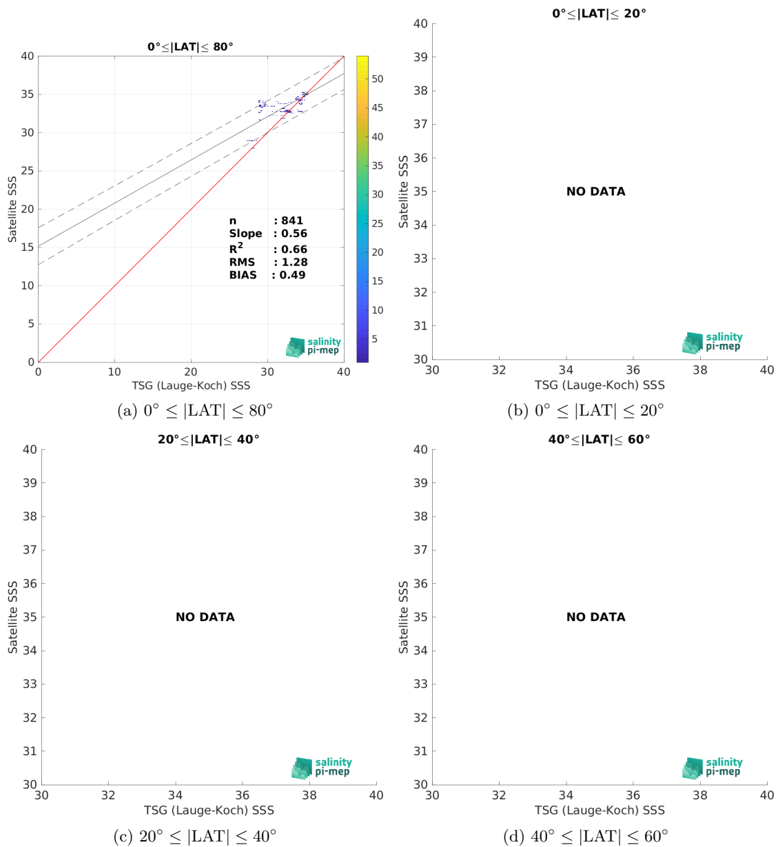
Figure 10: Contour maps of the concentration of CCI SSS L4 Merged-OI v5.5 - 7-day running (ESA) SSS (y-axis) versus TSG (Lauge-Koch) SSS (x-axis) at match-up pairs for different latitude bands. For each plot, the red line shows x=y . The black thin and dashed lines indicate a linear fit through the data cloud and the \pm 95\% confidence levels, respectively. The number match-up pairs n , the slope and R^2 coefficient of the linear fit, the root mean square (RMS) and the mean bias between satellite and in situ data are indicated for each latitude band in each plots.
