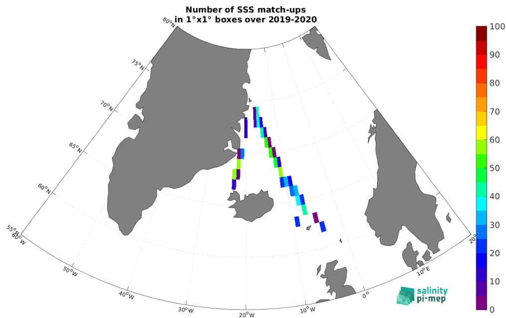
Figure 5: Number of SSS match-ups between TSG (Lauge-Koch) SSS and the CCI SSS L4 Merged-OI v5.5 - 7-day running (ESA) SSS product for the Arctic Ocean Pi-MEP region over 1^\circ \times 1^\circ boxes and for the full satellite product period.
