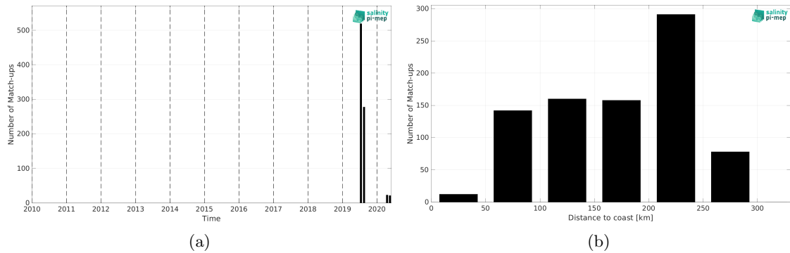
Figure 2: Number of match-ups between TSG (Lauge-Koch) and CCI SSS L4 Merged-OI v5.5 - 7-day running (ESA) SSS as a function of time (a) and as function of the distance to coast (b) over the Arctic Ocean Pi-MEP region and for the full satellite product period.
