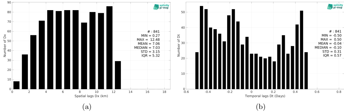
Figure 6: Histograms of the spatial (a) and temporal (b) lags between the location/time of the TSG (Lauge-Koch) measurement and the date of the corresponding CCI SSS L4 Merged-OI v5.5 - 7-day running (ESA) SSS pixel.
