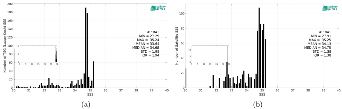
Figure 3: Histograms of SSS from TSG (Lauge-Koch) (a) and CCI SSS L4 Merged-OI v5.5 - 7-day running (ESA) (b) considering all match-up pairs per bins of 0.1 over the Arctic Ocean Pi-MEP region and for the full satellite product period.
