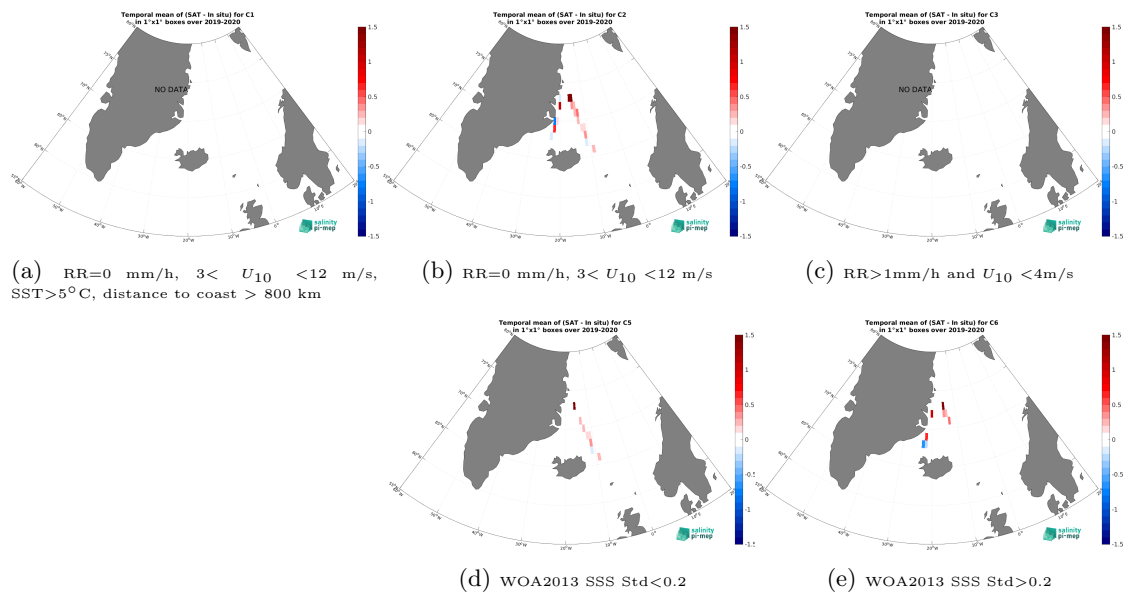
Figure 14: Temporal mean gridded over spatial boxes of size 1^\circ \times 1^\circ of \Delta SSS (CCI SSS L4 Merged-OI v5.5 - 7-day running (ESA) - TSG (Lauge-Koch)) for 5 different subdatasets corresponding to:RR=0 mm/h, 3 < U_{10} < 12 m/s, SST > 5^\circ\text{C} , distance to coast > 800 km (a), RR=0 mm/h, 3 < U_{10} < 12 m/s (b), RR > 1 mm/h and U_{10} < 4 m/s (c), WOA2013 SSS Std < 0.2 (d), WOA2013 SSS Std > 0.2 (e).
