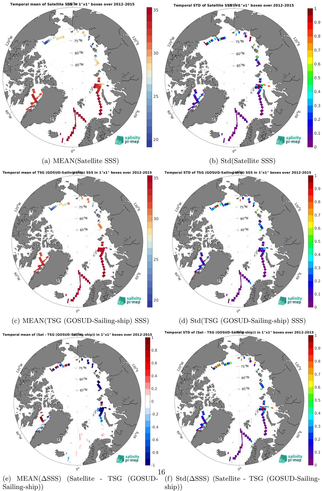
Figure 7: Temporal mean (left) and Std (right) of SSS from CCI SSS L4 Merged-OI v5.5 - 7-day running (ESA) (top), TSG (GOSUD-Sailing-ship) (middle), and of \Delta SSS (Satellite - TSG (GOSUD-Sailing-ship)). Only match-up pairs are used to generate these maps.
