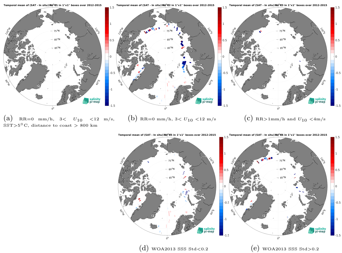
Figure 14: Temporal mean gridded over spatial boxes of size 1^\circ \times 1^\circ of \Delta\text{SSS} (CCI SSS L4 Merged-OI v5.5 - 7-day running (ESA) - TSG (GOSUD-Sailing-ship)) for 5 different subdatasets corresponding to:RR=0 mm/h, 3 < U_{10} < 12 m/s, SST>5°C, distance to coast > 800 km (a), RR=0 mm/h, 3 < U_{10} < 12 m/s (b), RR>1mm/h and U_{10} < 4 m/s (c), WOA2013 SSS Std<0.2 (d), WOA2013 SSS Std>0.2 (e).
