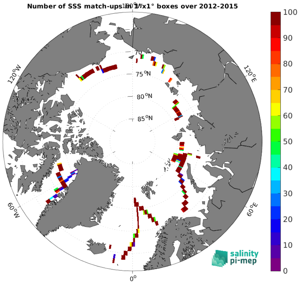
Figure 5: Number of SSS match-ups between TSG (GOSUD-Sailing-ship) SSS and the CCI SSS L4 Merged-OI v5.5 - 7-day running (ESA) SSS product for the Arctic Ocean Pi-MEP region over 1^\circ \times 1^\circ boxes and for the full satellite product period.
