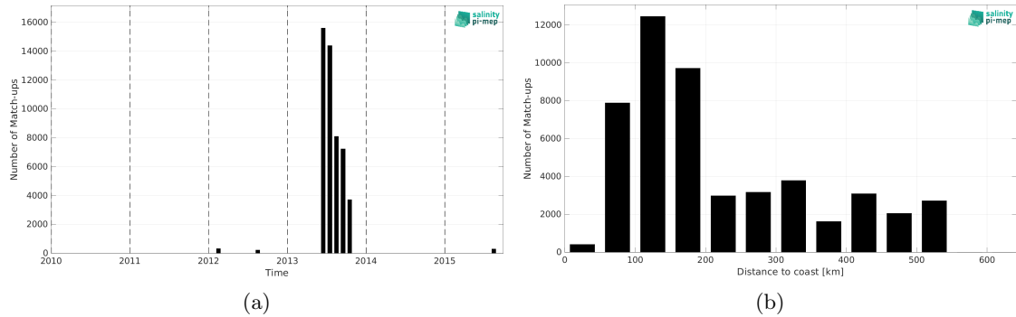
Figure 2: Number of match-ups between TSG (GOSUD-Sailing-ship) and CCI SSS L4 Merged-OI v5.5 - 7-day running (ESA) SSS as a function of time (a) and as function of the distance to coast (b) over the Arctic Ocean Pi-MEP region and for the full satellite product period.
