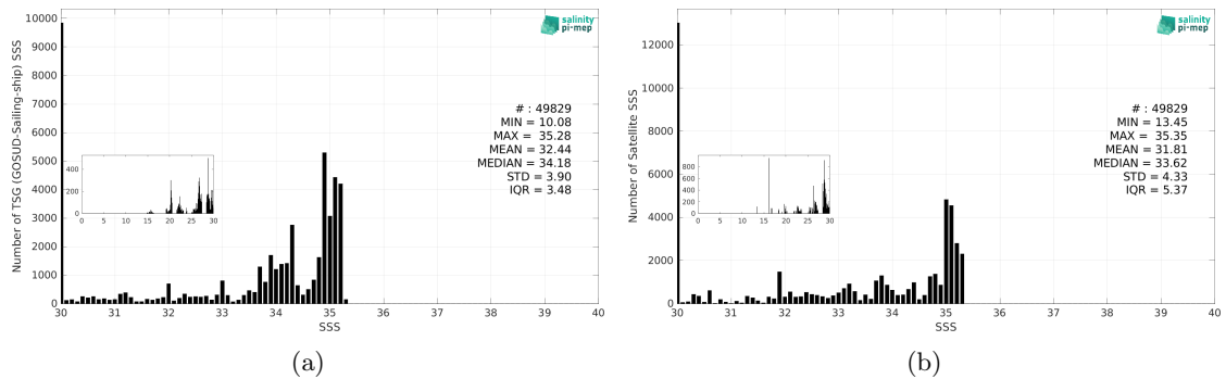
Figure 3: Histograms of SSS from TSG (GOSUD-Sailing-ship) (a) and CCI SSS L4 Merged-OI v5.5 - 7-day running (ESA) (b) considering all match-up pairs per bins of 0.1 over the Arctic Ocean Pi-MEP region and for the full satellite product period.
