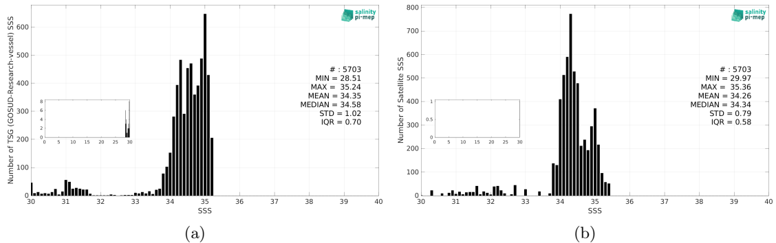
Figure 3: Histograms of SSS from TSG (GOSUD-Research-vessel) (a) and CCI SSS L4 Merged-OI v5.5 - 7-day running (ESA) (b) considering all match-up pairs per bins of 0.1 over the Arctic Ocean Pi-MEP region and for the full satellite product period.
