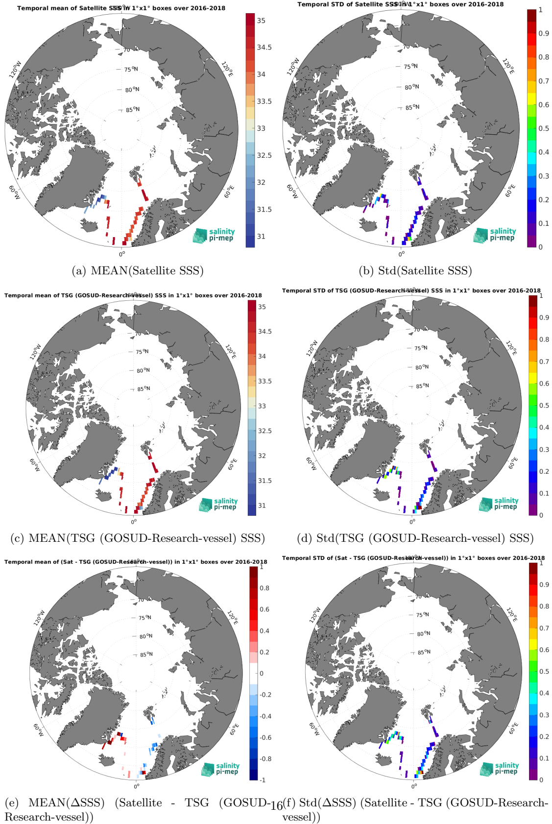
Figure 7: Temporal mean (left) and Std (right) of SSS from CCI SSS L4 Merged-OI v5.5 - 7-day running (ESA) (top), TSG (GOSUD-Research-vessel) (middle), and of \Delta SSS (Satellite - TSG (GOSUD-Research-vessel)). Only match-up pairs are used to generate these maps.
