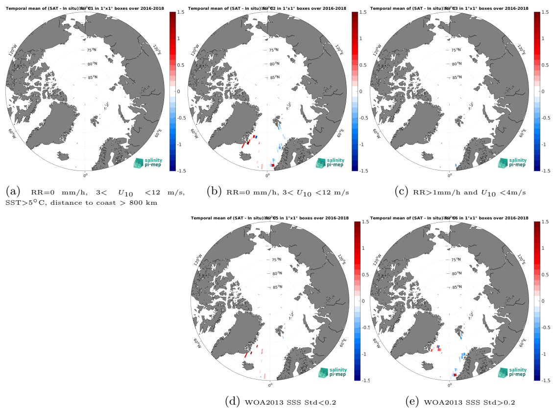
Figure 14: Temporal mean gridded over spatial boxes of size 1^\circ \times 1^\circ of \Delta SSS (CCI SSS L4 Merged-OI v5.5 - 7-day running (ESA) - TSG (GOSUD-Research-vessel)) for 5 different subdatasets corresponding to: RR=0 mm/h, 3 < U_{10} < 12 m/s, SST > 5^\circ\text{C} , distance to coast > 800 km (a), RR=0 mm/h, 3 < U_{10} < 12 m/s (b), RR > 1 mm/h and U_{10} < 4 m/s (c), WOA2013 SSS Std < 0.2 (d), WOA2013 SSS Std > 0.2 (e).
