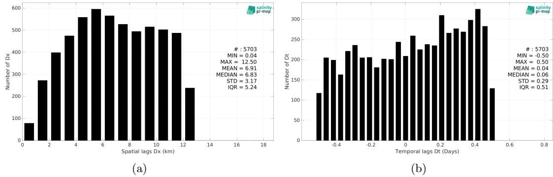
Figure 6: Histograms of the spatial (a) and temporal (b) lags between the location/time of the TSG (GOSUD-Research-vessel) measurement and the date of the corresponding CCI SSS L4 Merged-OI v5.5 - 7-day running (ESA) SSS pixel.
