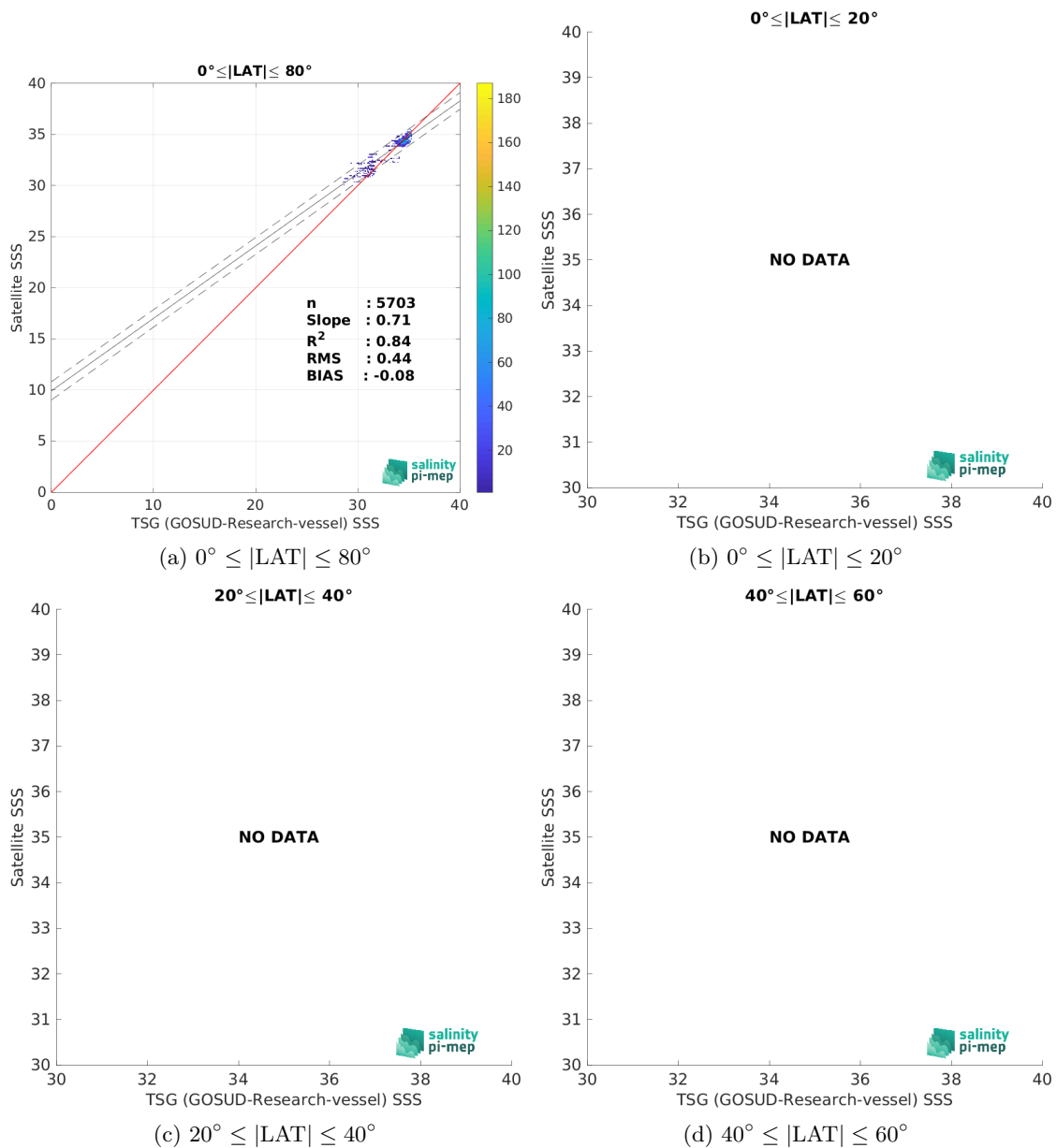
Figure 10: Contour maps of the concentration of CCI SSS L4 Merged-OI v5.5 - 7-day running (ESA) SSS (y-axis) versus TSG (GOSUD-Research-vessel) SSS (x-axis) at match-up pairs for different latitude bands. For each plot, the red line shows x=y . The black thin and dashed lines indicate a linear fit through the data cloud and the \pm 95\% confidence levels, respectively. The number match-up pairs n , the slope and R^2 coefficient of the linear fit, the root mean square (RMS) and the mean bias between satellite and in situ data are indicated for each latitude band in each plots.
