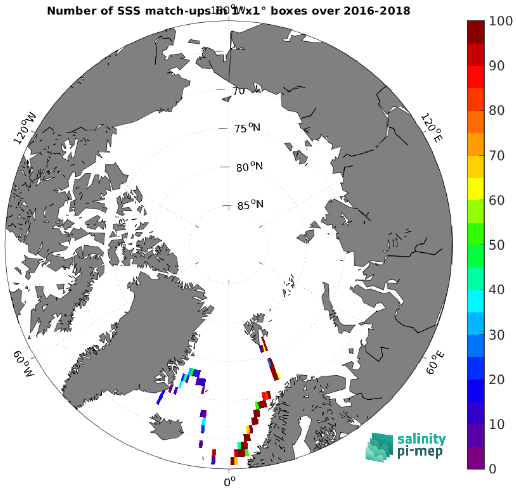
Figure 5: Number of SSS match-ups between TSG (GOSUD-Research-vessel) SSS and the CCI SSS L4 Merged-OI v5.5 - 7-day running (ESA) SSS product for the Arctic Ocean Pi-MEP region over 1^\circ \times 1^\circ boxes and for the full satellite product period.
