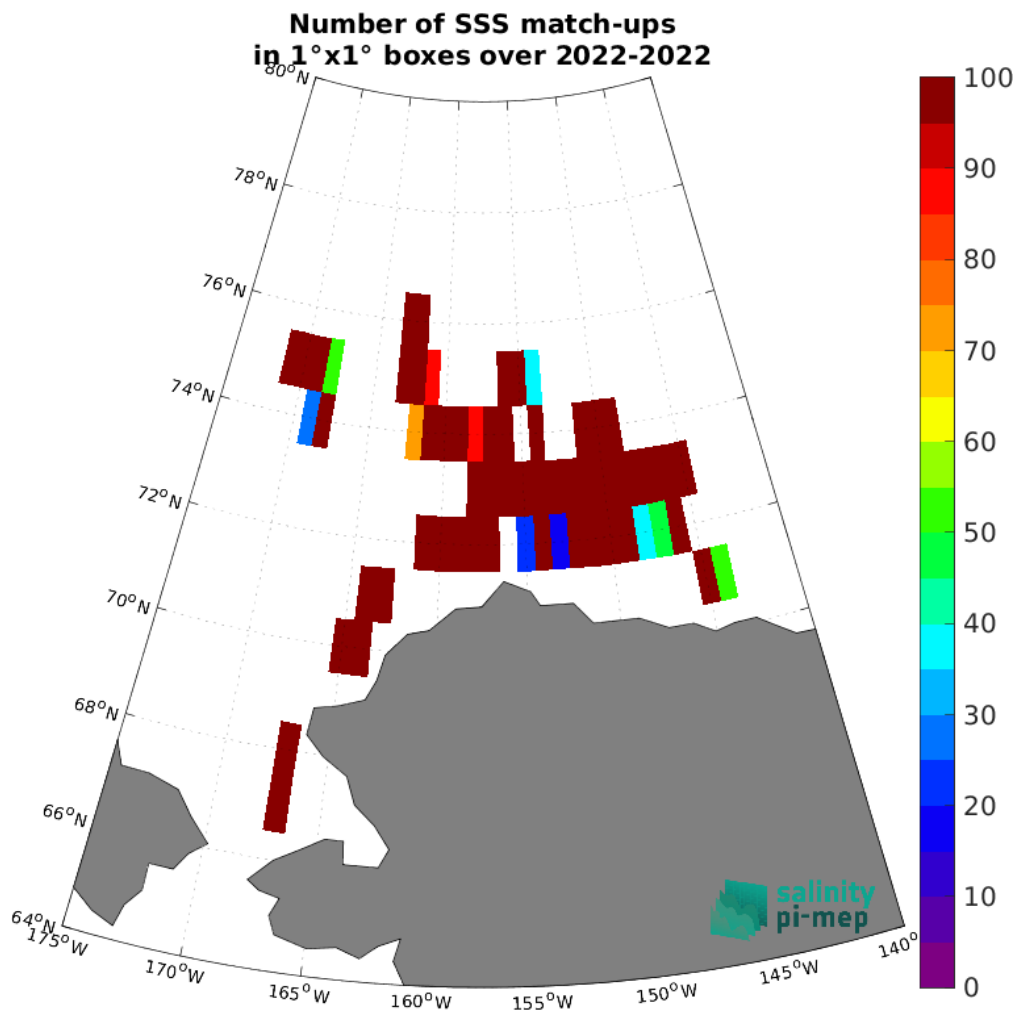
Figure 5: Number of SSS match-ups between SASSIE SSS and the CCI SSS L4 Merged-OI v5.5 - 7-day running (ESA) SSS product for the Arctic Ocean Pi-MEP region over 1^\circ \times 1^\circ boxes and for the full satellite product period.
