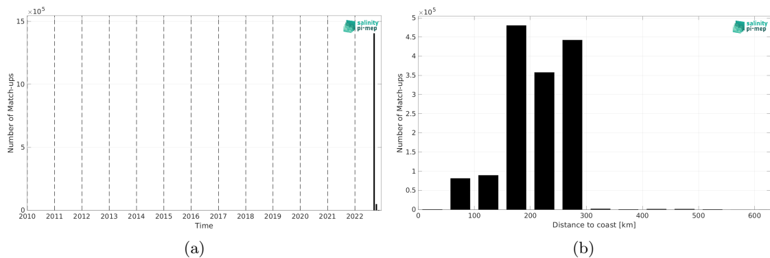
Figure 2: Number of match-ups between SASSIE and CCI SSS L4 Merged-OI v5.5 - 7-day running (ESA) SSS as a function of time (a) and as function of the distance to coast (b) over the Arctic Ocean Pi-MEP region and for the full satellite product period.
