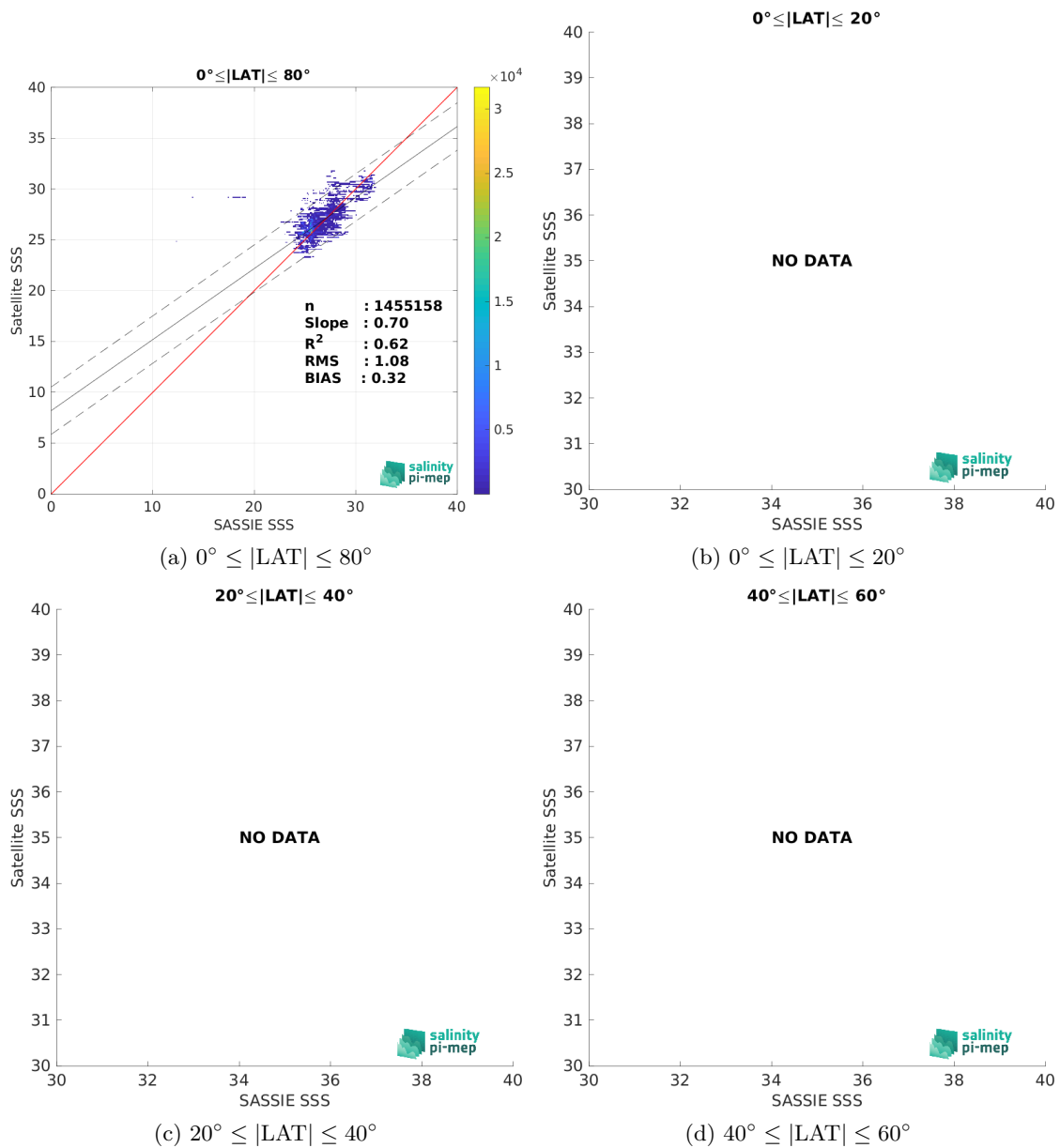
Figure 10: Contour maps of the concentration of CCI SSS L4 Merged-OI v5.5 - 7-day running (ESA) SSS (y-axis) versus SASSIE SSS (x-axis) at match-up pairs for different latitude bands. For each plot, the red line shows x=y . The black thin and dashed lines indicate a linear fit through the data cloud and the \pm 95\% confidence levels, respectively. The number match-up pairs n , the slope and R^2 coefficient of the linear fit, the root mean square (RMS) and the mean bias between satellite and in situ data are indicated for each latitude band in each plots.
