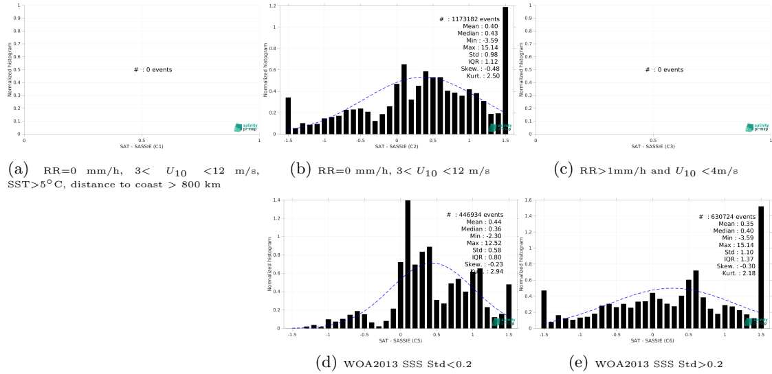
Figure 15: Normalized histogram of \Delta SSS (CCI SSS L4 Merged-OI v5.5 - 7-day running (ESA) - SASSIE) for 5 different subdatasets corresponding to: RR=0 mm/h, 3 < U_{10} < 12 m/s, SST > 5°C, distance to coast > 800 km (a), RR=0 mm/h, 3 < U_{10} < 12 m/s (b), RR > 1mm/h and U_{10} < 4 m/s (c), WOA2013 SSS Std < 0.2 (d), WOA2013 SSS Std > 0.2 (e).
