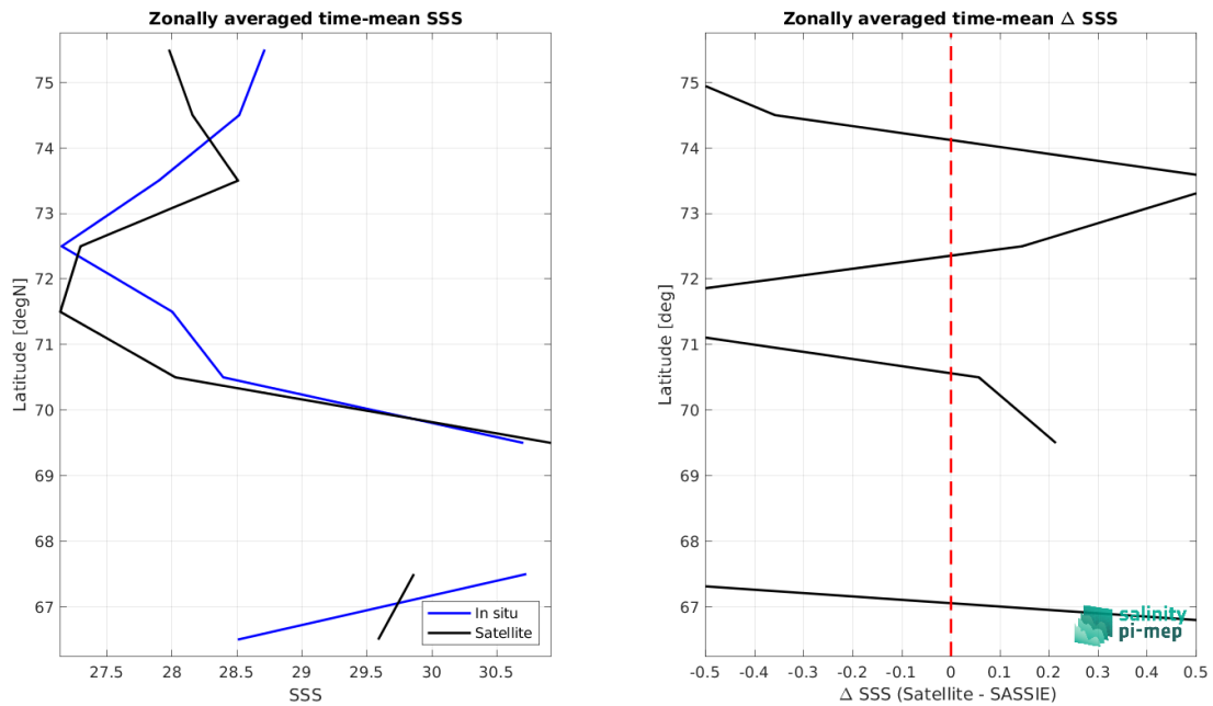
Figure 9: Left panel: Zonal mean SSS from CCI SSS L4 Merged-OI v5.5 - 7-day running (ESA) satellite product (black) and from SASSIE (blue). Right panel: Zonal mean of \Delta SSS (Satellite - SASSIE) for all the collected Pi-MEP match-up pairs estimated over the full satellite product period.
