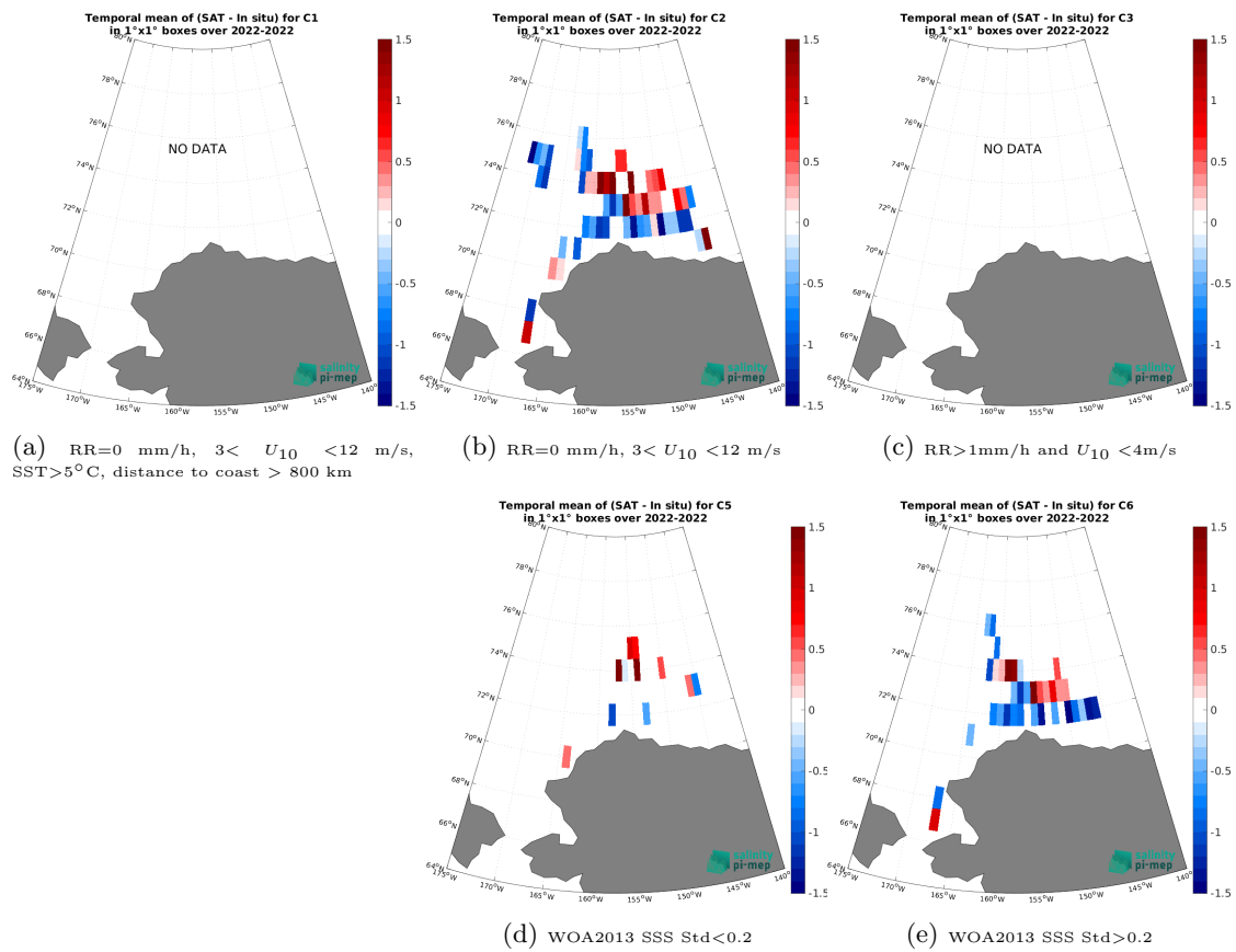
Figure 14: Temporal mean gridded over spatial boxes of size 1^\circ \times 1^\circ of \Delta\text{SSS} (CCI SSS L4 Merged-OI v5.5 - 7-day running (ESA) - SASSIE) for 5 different subdatasets corresponding to:RR=0 mm/h, 3 < U_{10} < 12 m/s, SST>5°C, distance to coast > 800 km (a), RR=0 mm/h, 3 < U_{10} < 12 m/s (b), RR>1mm/h and U_{10} < 4 m/s (c), WOA2013 SSS Std<0.2 (d), WOA2013 SSS Std>0.2 (e).
