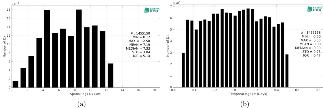
Figure 6: Histograms of the spatial (a) and temporal (b) lags between the location/time of the SASSIE measurement and the date of the corresponding CCI SSS L4 Merged-OI v5.5 - 7-day running (ESA) SSS pixel.
