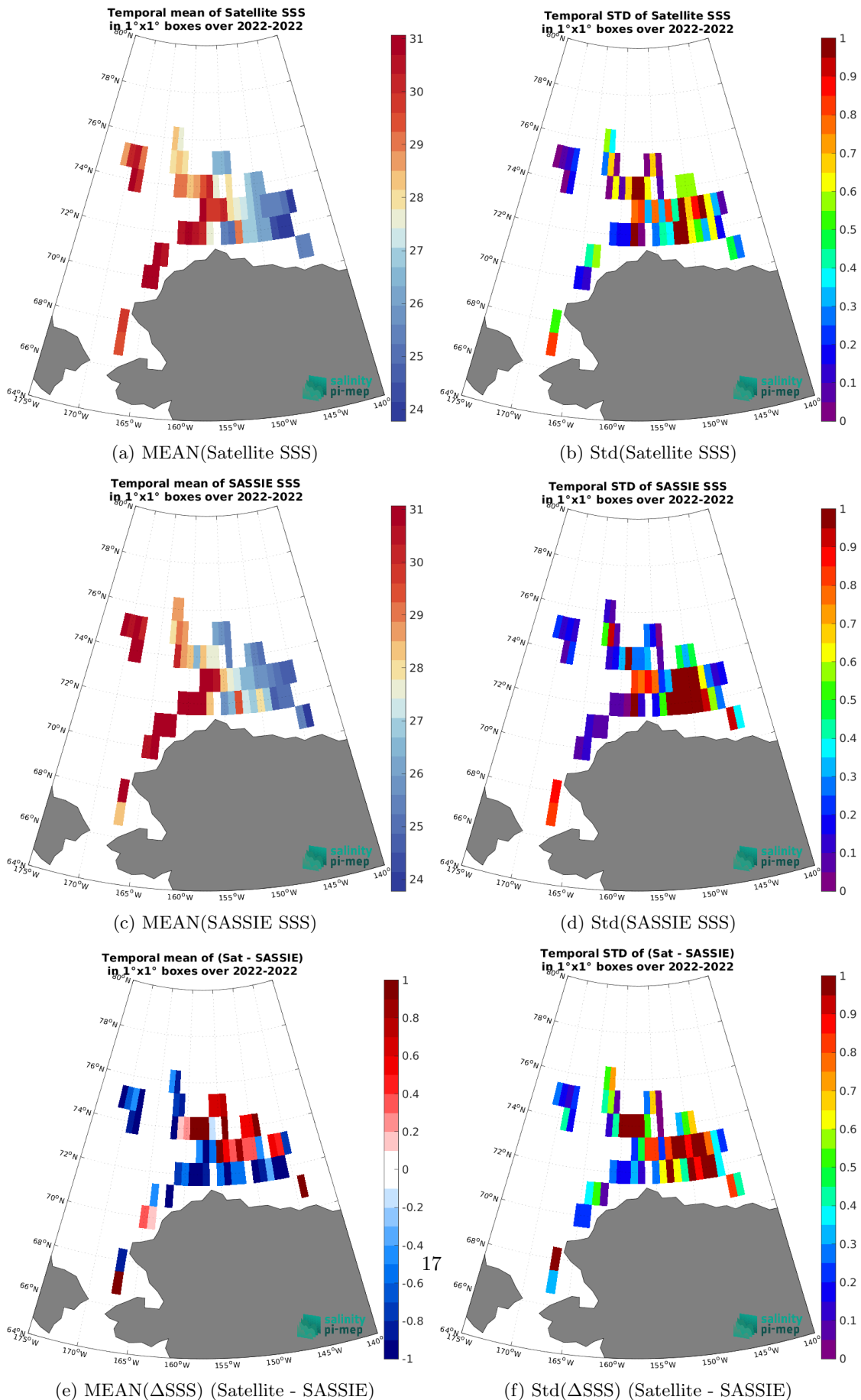
Figure 7: Temporal mean (left) and Std (right) of SSS from CCI SSS L4 Merged-OI v5.5 - 7-day running (ESA) (top), SASSIE (middle), and of \Delta SSS (Satellite - SASSIE). Only match-up pairs are used to generate these maps.
