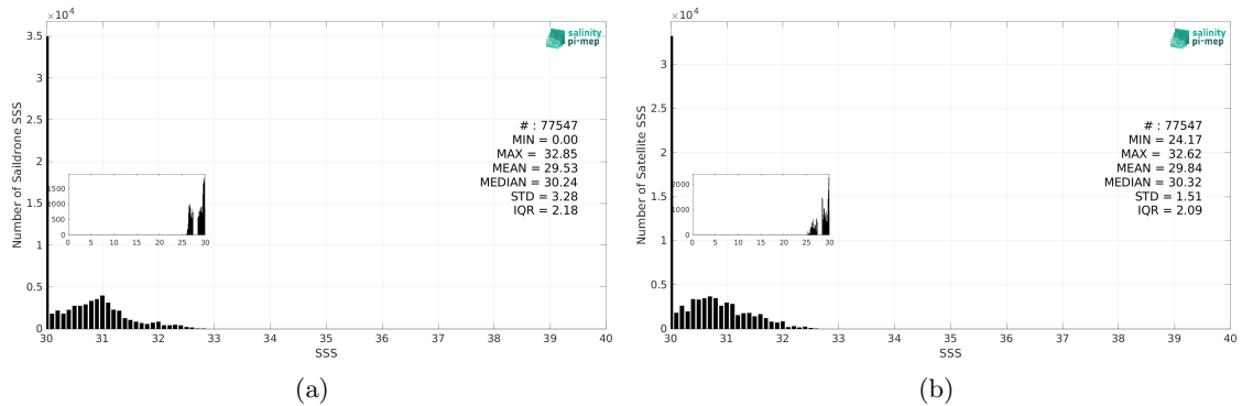
Figure 3: Histograms of SSS from Saildrone (a) and CCI SSS L4 Merged-OI v5.5 - 7-day running (ESA) (b) considering all match-up pairs per bins of 0.1 over the Arctic Ocean Pi-MEP region and for the full satellite product period.
