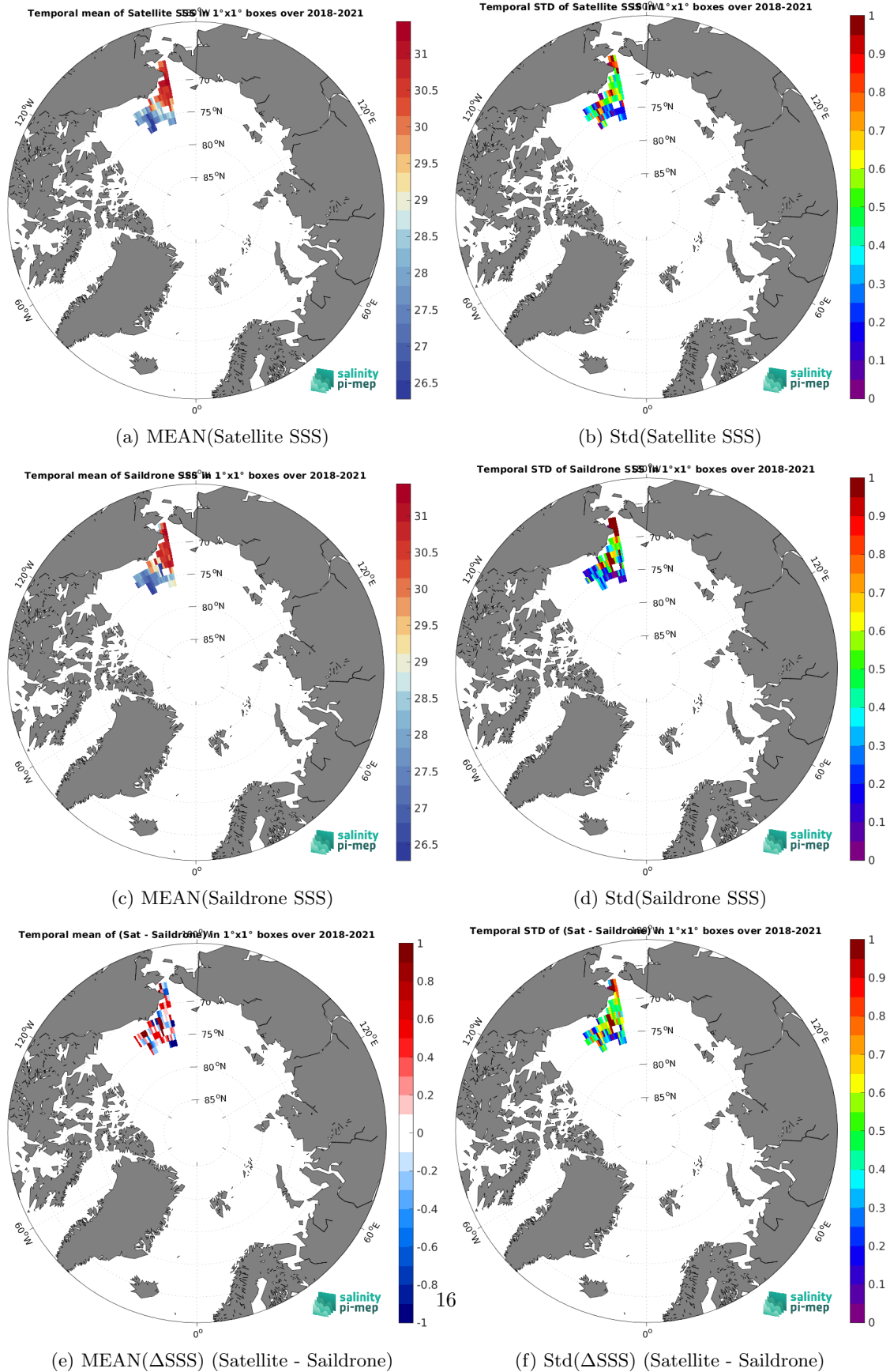
Figure 7: Temporal mean (left) and Std (right) of SSS from CCI SSS L4 Merged-OI v5.5 - 7-day running (ESA) (top), Saildrone (middle), and of \Delta SSS (Satellite - Saildrone). Only match-up pairs are used to generate these maps.
