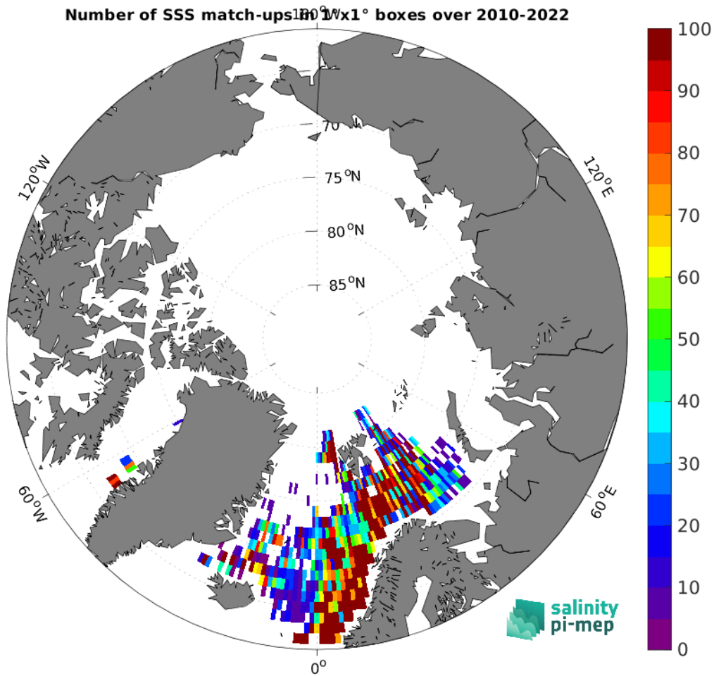
Figure 5: Number of SSS match-ups between ICES SSS and the CCI SSS L4 Merged-OI v5.5 - 7-day running (ESA) SSS product for the Arctic Ocean Pi-MEP region over 1^\circ \times 1^\circ boxes and for the full satellite product period.
