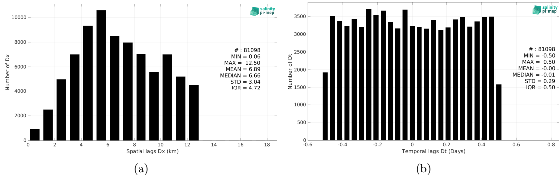
Figure 6: Histograms of the spatial (a) and temporal (b) lags between the location/time of the ICES measurement and the date of the corresponding CCI SSS L4 Merged-OI v5.5 - 7-day running (ESA) SSS pixel.
