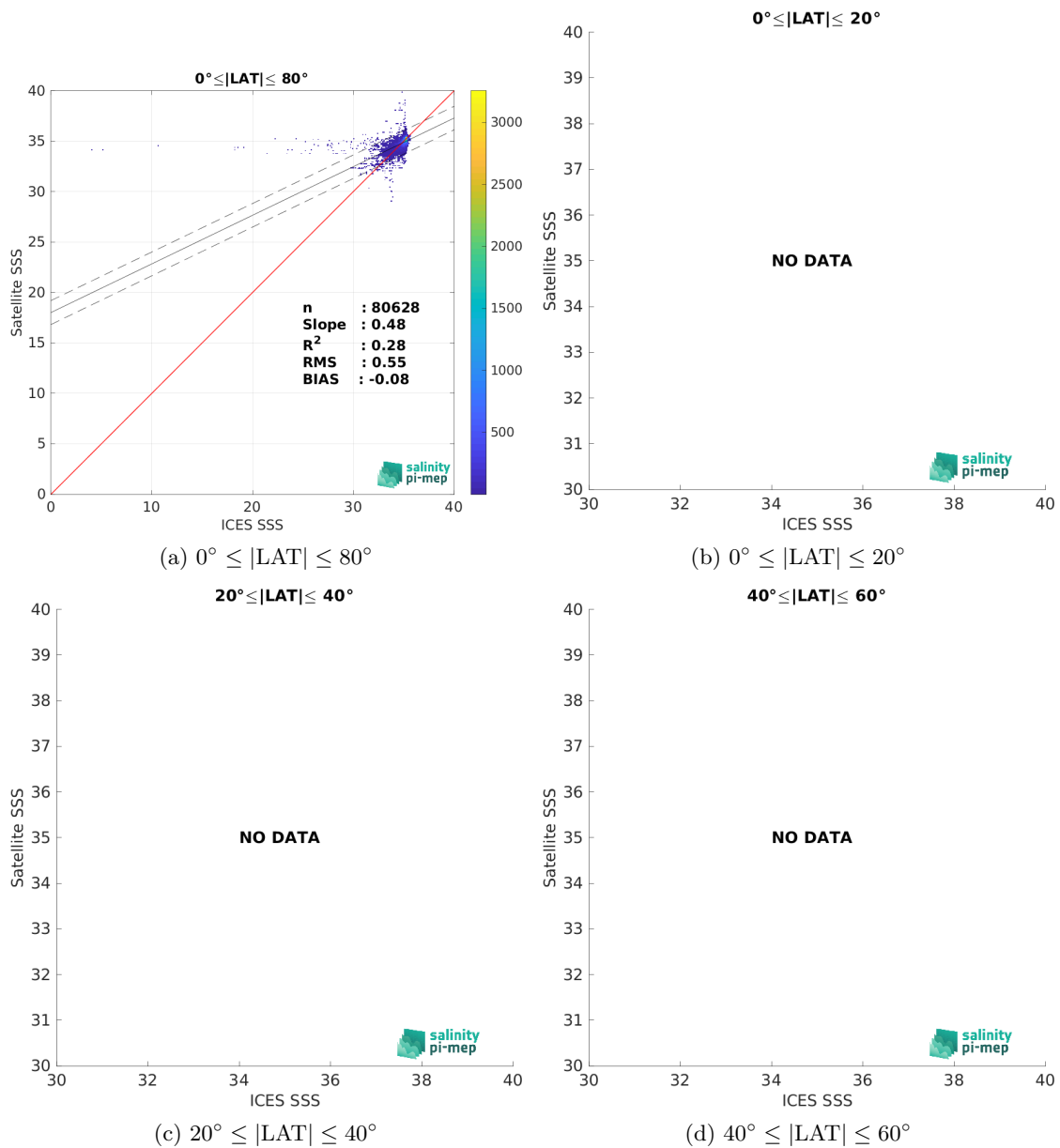
Figure 10: Contour maps of the concentration of CCI SSS L4 Merged-OI v5.5 - 7-day running (ESA) SSS (y-axis) versus ICES SSS (x-axis) at match-up pairs for different latitude bands. For each plot, the red line shows x=y . The black thin and dashed lines indicate a linear fit through the data cloud and the \pm 95\% confidence levels, respectively. The number match-up pairs n , the slope and R^2 coefficient of the linear fit, the root mean square (RMS) and the mean bias between satellite and in situ data are indicated for each latitude band in each plots.
