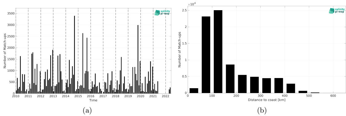
Figure 2: Number of match-ups between ICES and CCI SSS L4 Merged-OI v5.5 - 7-day running (ESA) SSS as a function of time (a) and as function of the distance to coast (b) over the Arctic Ocean Pi-MEP region and for the full satellite product period.
