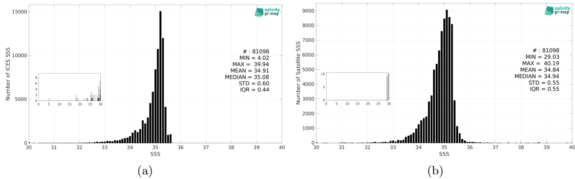
Figure 3: Histograms of SSS from ICES (a) and CCI SSS L4 Merged-OI v5.5 - 7-day running (ESA) (b) considering all match-up pairs per bins of 0.1 over the Arctic Ocean Pi-MEP region and for the full satellite product period.
