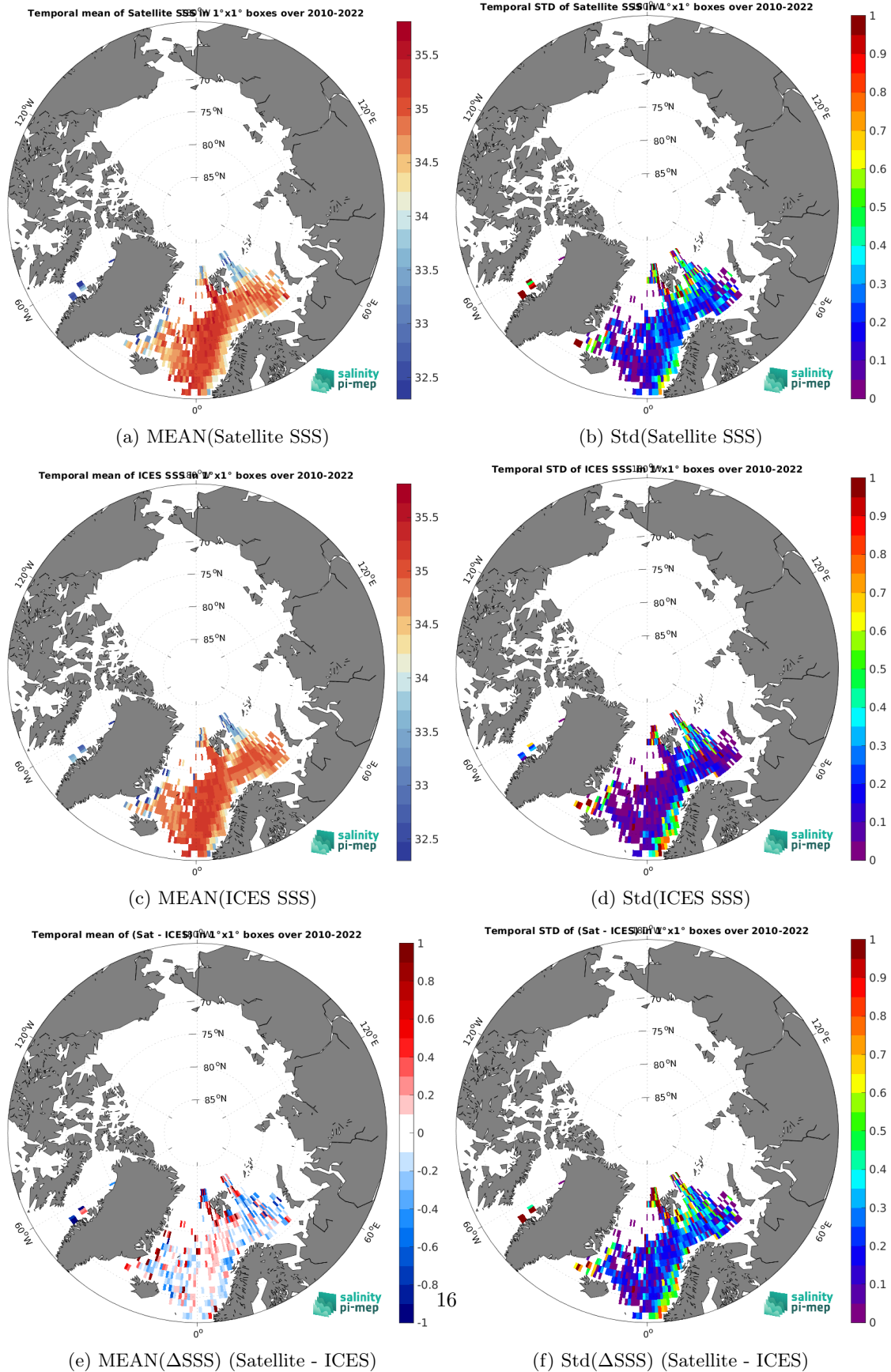
Figure 7: Temporal mean (left) and Std (right) of SSS from CCI SSS L4 Merged-OI v5.5 - 7-day running (ESA) (top), ICES (middle), and of \Delta SSS (Satellite - ICES). Only match-up pairs are used to generate these maps.
