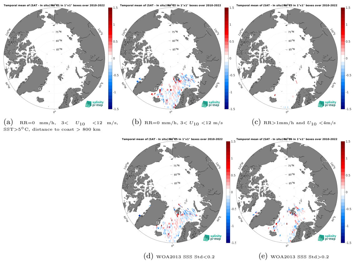
Figure 14: Temporal mean gridded over spatial boxes of size 1^\circ \times 1^\circ of \Delta SSS (CCI SSS L4 Merged-OI v5.5 - 7-day running (ESA) - ICES) for 5 different subdatasets corresponding to:RR=0 mm/h, 3 < U_{10} < 12 m/s, SST >5^\circ C, distance to coast > 800 km (a), RR=0 mm/h, 3 < U_{10} < 12 m/s (b), RR >1 mm/h and U_{10} < 4 m/s (c), WOA2013 SSS Std <0.2 (d), WOA2013 SSS Std >0.2 (e).
