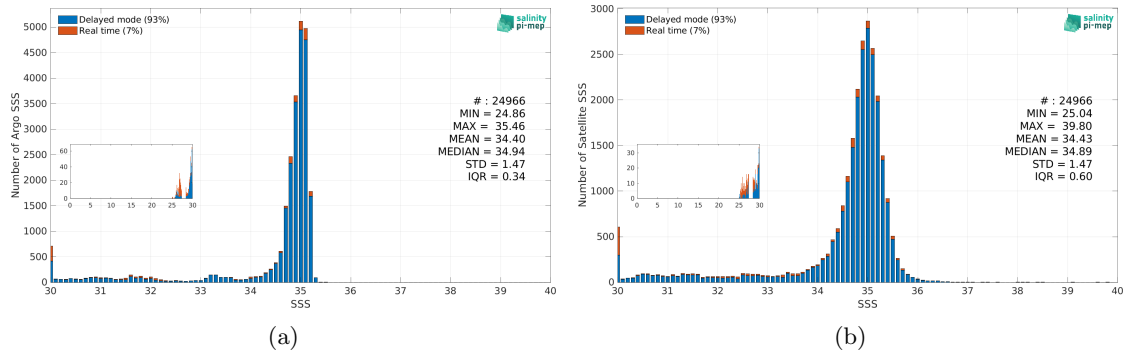
Figure 3: Histograms of SSS from Argo (a) and CCI SSS L4 Merged-OI v5.5 - 7-day running (ESA) (b) considering all match-up pairs per bins of 0.1 over the Arctic Ocean Pi-MEP region and for the full satellite product period.
