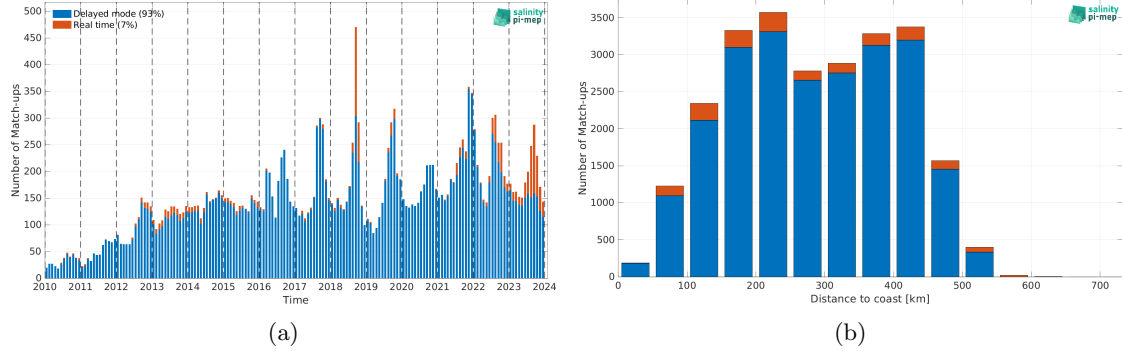
Figure 2: Number of match-ups between Argo and CCI SSS L4 Merged-OI v5.5 - 7-day running (ESA) SSS as a function of time (a) and as function of the distance to coast (b) over the Arctic Ocean Pi-MEP region and for the full satellite product period.
