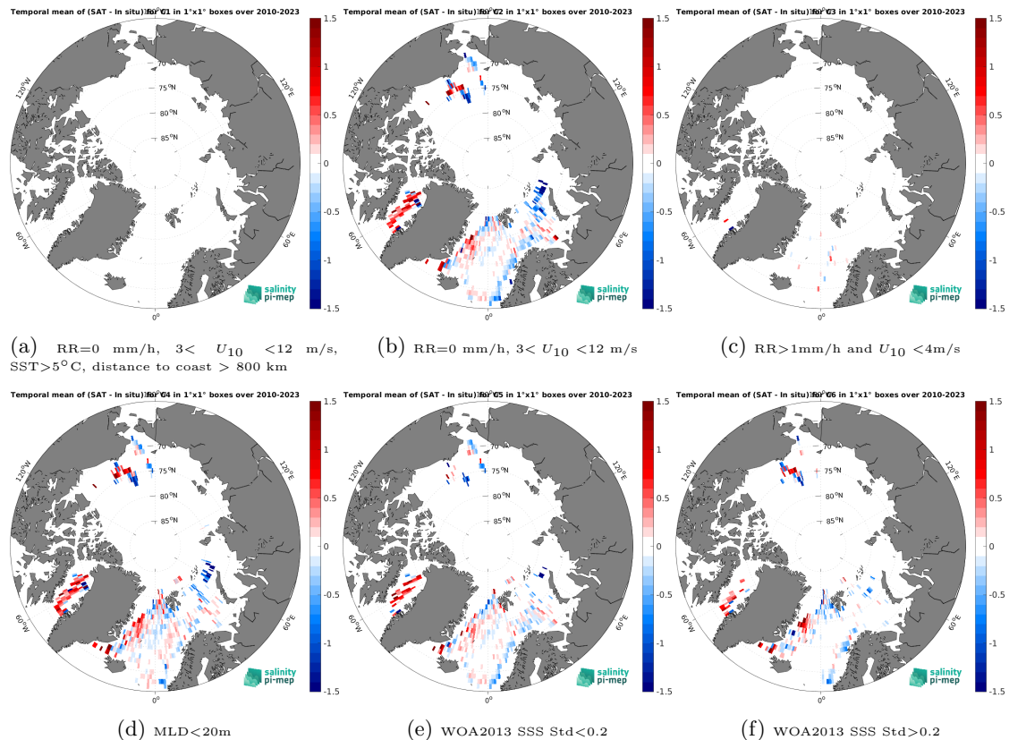
Figure 14: Temporal mean gridded over spatial boxes of size 1^\circ \times 1^\circ of \Delta\text{SSS} (CCI SSS L4 Merged-OI v5.5 - 7-day running (ESA) - Argo) for 6 different subdatasets corresponding to: RR=0 mm/h, 3 < U_{10} < 12 m/s, SST > 5°C, distance to coast > 800 km (a), RR=0 mm/h, 3 < U_{10} < 12 m/s (b), RR > 1mm/h and U_{10} < 4 m/s (c), MLD < 20m (d), WOA2013 SSS Std < 0.2 (e), WOA2013 SSS Std > 0.2 (f).
