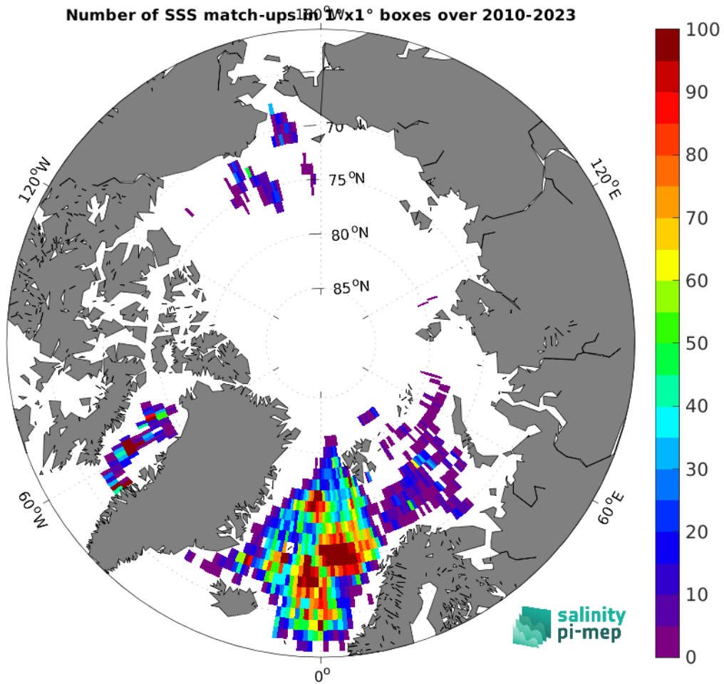
Figure 5: Number of SSS match-ups between Argo SSS and the CCI SSS L4 Merged-OI v5.5 - 7-day running (ESA) SSS product for the Arctic Ocean Pi-MEP region over 1^\circ \times 1^\circ boxes and for the full satellite product period.
