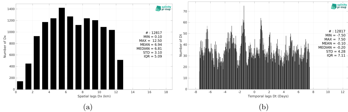
Figure 6: Histograms of the spatial (a) and temporal (b) lags between the location/time of the TSG (SAMOS) measurement and the date of the corresponding CCI SSS L4 Merged-OI v5.5 - 30-day running (ESA) SSS pixel.
