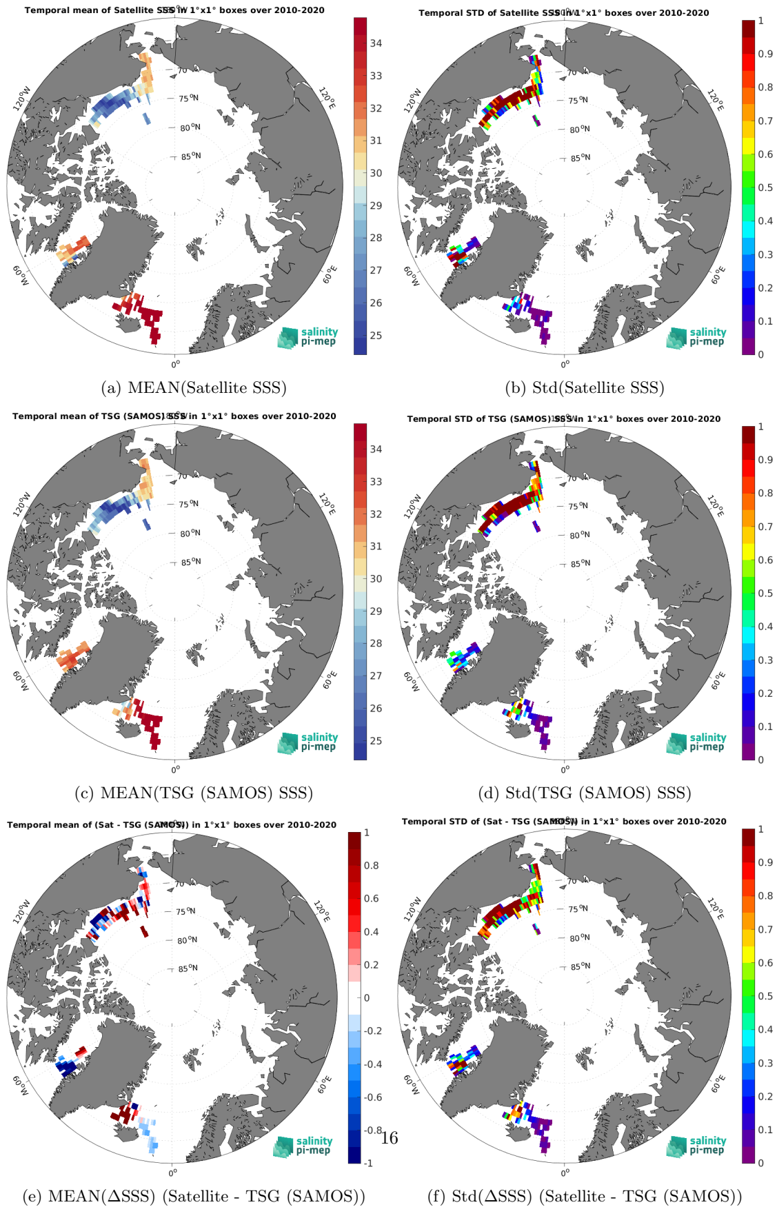
Figure 7: Temporal mean (left) and Std (right) of SSS from CCI SSS L4 Merged-OI v5.5 - 30-day running (ESA) (top), TSG (SAMOS) (middle), and of \Delta SSS (Satellite - TSG (SAMOS)). Only match-up pairs are used to generate these maps.
