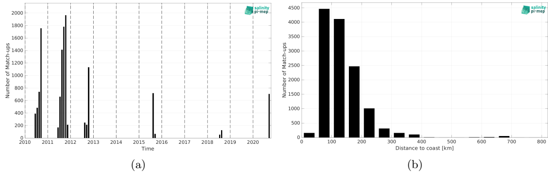
Figure 2: Number of match-ups between TSG (SAMOS) and CCI SSS L4 Merged-OI v5.5 - 30-day running (ESA) SSS as a function of time (a) and as function of the distance to coast (b) over the Arctic Ocean Pi-MEP region and for the full satellite product period.
