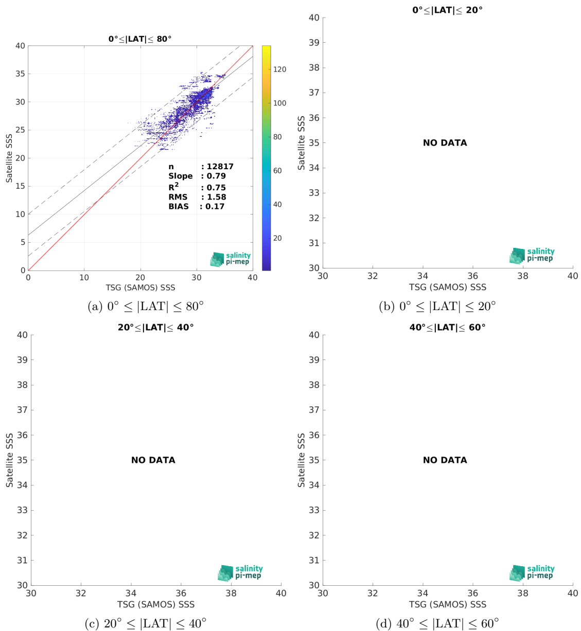
Figure 10: Contour maps of the concentration of CCI SSS L4 Merged-OI v5.5 - 30-day running (ESA) SSS (y-axis) versus TSG (SAMOS) SSS (x-axis) at match-up pairs for different latitude bands. For each plot, the red line shows x=y . The black thin and dashed lines indicate a linear fit through the data cloud and the \pm 95\% confidence levels, respectively. The number match-up pairs n , the slope and R^2 coefficient of the linear fit, the root mean square (RMS) and the mean bias between satellite and in situ data are indicated for each latitude band in each plots.
