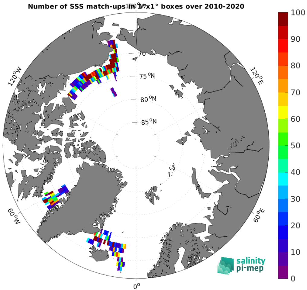
Figure 5: Number of SSS match-ups between TSG (SAMOS) SSS and the CCI SSS L4 Merged-OI v5.5 - 30-day running (ESA) SSS product for the Arctic Ocean Pi-MEP region over 1^\circ \times 1^\circ boxes and for the full satellite product period.
