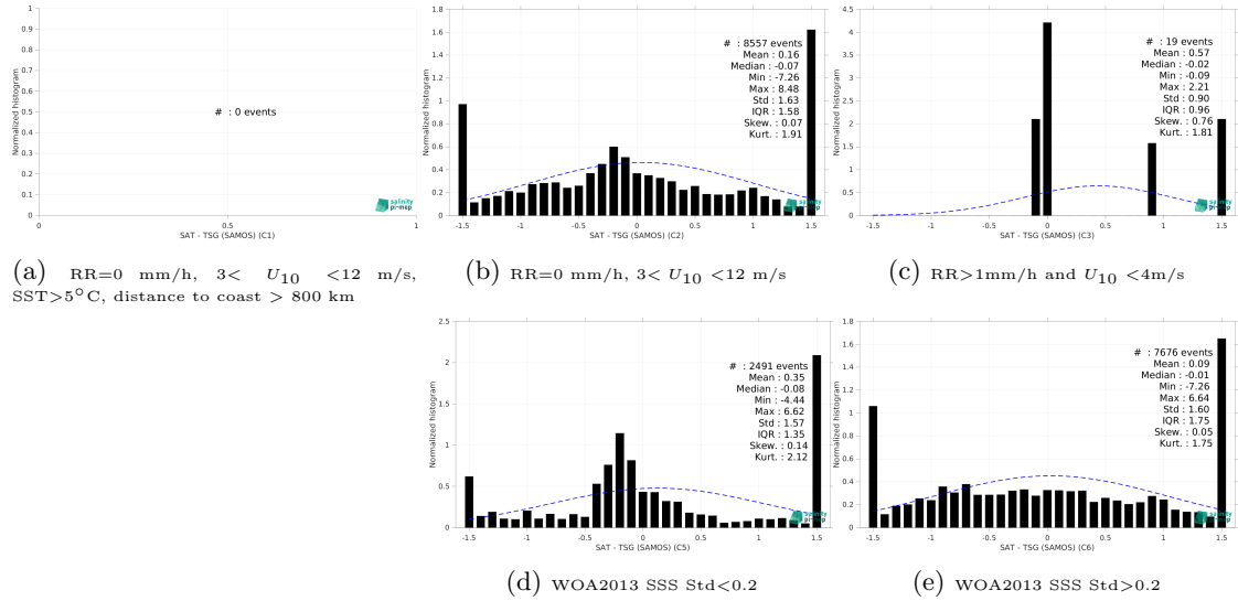
Figure 15: Normalized histogram of \Delta SSS (CCI SSS L4 Merged-OI v5.5 - 30-day running (ESA) - TSG (SAMOS)) for 5 different subdatasets corresponding to: RR=0 mm/h, 3 < U_{10} < 12 m/s, SST > 5°C, distance to coast > 800 km (a), RR=0 mm/h, 3 < U_{10} < 12 m/s (b), RR > 1mm/h and U_{10} < 4 m/s (c), WOA2013 SSS Std < 0.2 (d), WOA2013 SSS Std > 0.2 (e).
