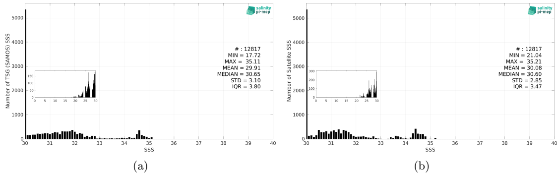
Figure 3: Histograms of SSS from TSG (SAMOS) (a) and CCI SSS L4 Merged-OI v5.5 - 30-day running (ESA) (b) considering all match-up pairs per bins of 0.1 over the Arctic Ocean Pi-MEP region and for the full satellite product period.
