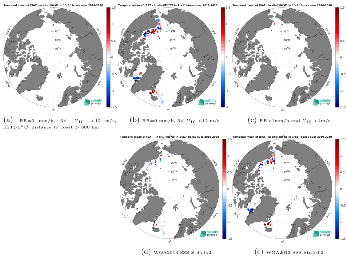
Figure 14: Temporal mean gridded over spatial boxes of size 1^\circ \times 1^\circ of \Delta\text{SSS} (CCI SSS L4 Merged-OI v5.5 - 30-day running (ESA) - TSG (SAMOS)) for 5 different subdatasets corresponding to: RR=0 mm/h, 3 < U_{10} < 12 m/s, SST > 5^\circ\text{C} , distance to coast > 800 km (a), RR=0 mm/h, 3 < U_{10} < 12 m/s (b), RR > 1 mm/h and U_{10} < 4 m/s (c), WOA2013 SSS Std < 0.2 (d), WOA2013 SSS Std > 0.2 (e).
