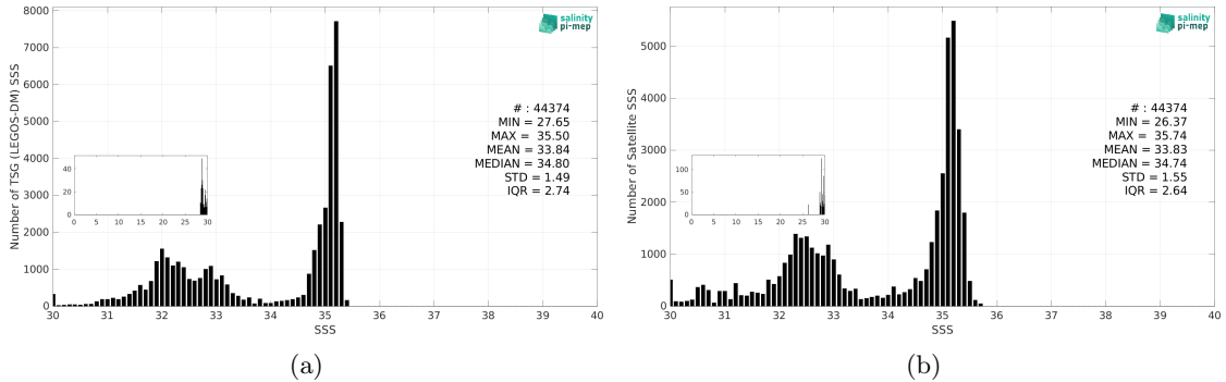
Figure 3: Histograms of SSS from TSG (LEGOS-DM) (a) and CCI SSS L4 Merged-OI v5.5 - 30-day running (ESA) (b) considering all match-up pairs per bins of 0.1 over the Arctic Ocean Pi-MEP region and for the full satellite product period.
