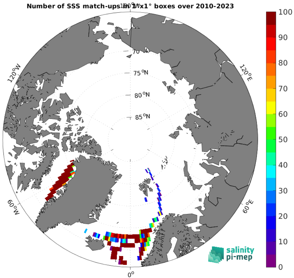
Figure 5: Number of SSS match-ups between TSG (LEGOS-DM) SSS and the CCI SSS L4 Merged-OI v5.5 - 30-day running (ESA) SSS product for the Arctic Ocean Pi-MEP region over 1^\circ \times 1^\circ boxes and for the full satellite product period.
