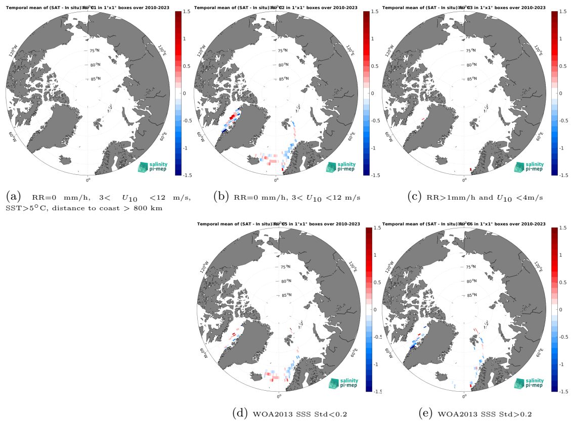
Figure 14: Temporal mean gridded over spatial boxes of size 1^\circ \times 1^\circ of \Delta\text{SSS} (CCI SSS L4 Merged-OI v5.5 - 30-day running (ESA) - TSG (LEGOS-DM)) for 5 different subdatasets corresponding to:RR=0 mm/h, 3 < U_{10} < 12 m/s, SST > 5°C, distance to coast > 800 km (a), RR=0 mm/h, 3 < U_{10} < 12 m/s (b), RR > 1mm/h and U_{10} < 4 m/s (c), WOA2013 SSS Std < 0.2 (d), WOA2013 SSS Std > 0.2 (e).
