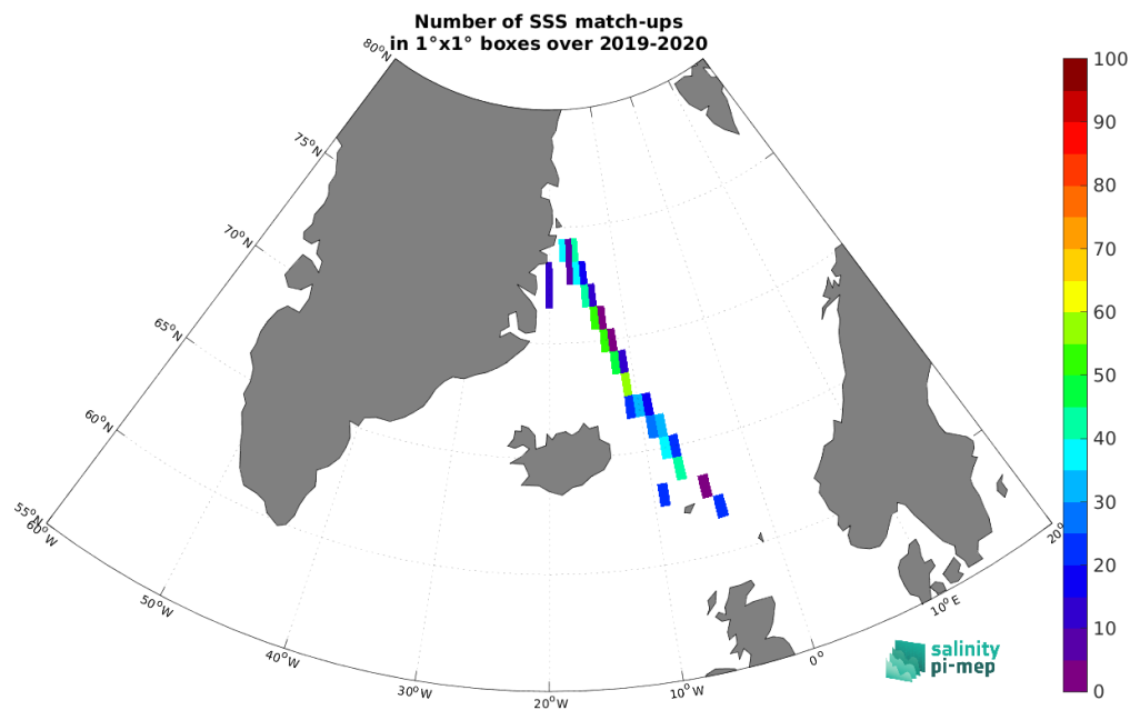
Figure 5: Number of SSS match-ups between TSG (Lauge-Koch) SSS and the CCI SSS L4 Merged-OI v5.5 - 30-day running (ESA) SSS product for the Arctic Ocean Pi-MEP region over 1^\circ \times 1^\circ boxes and for the full satellite product period.
