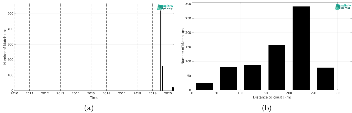
Figure 2: Number of match-ups between TSG (Lauge-Koch) and CCI SSS L4 Merged-OI v5.5 - 30-day running (ESA) SSS as a function of time (a) and as function of the distance to coast (b) over the Arctic Ocean Pi-MEP region and for the full satellite product period.
