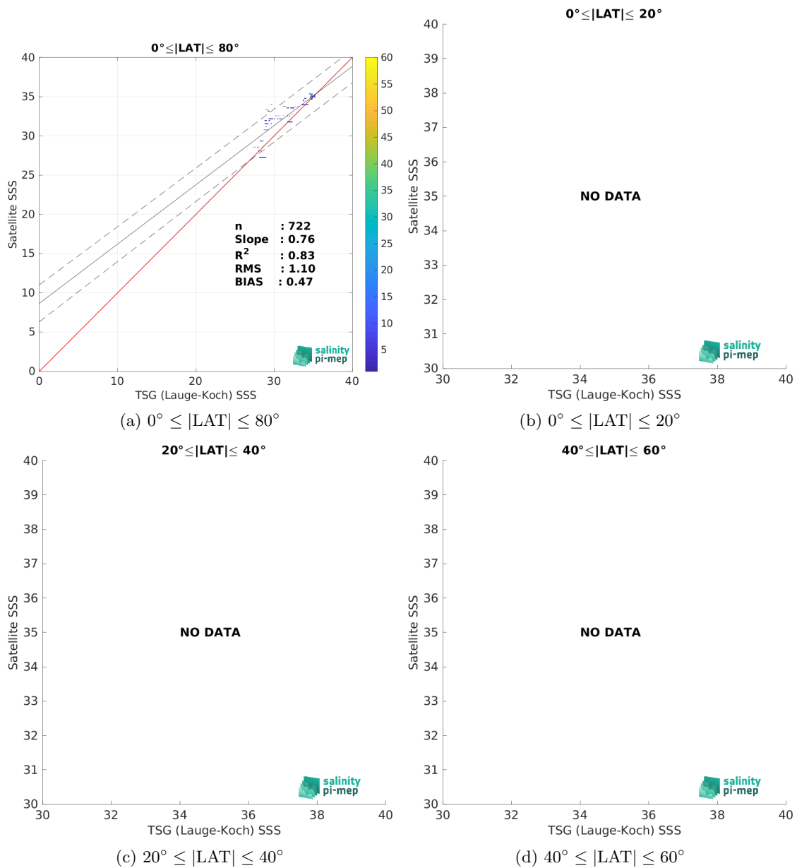
Figure 10: Contour maps of the concentration of CCI SSS L4 Merged-OI v5.5 - 30-day running (ESA) SSS (y-axis) versus TSG (Lauge-Koch) SSS (x-axis) at match-up pairs for different latitude bands. For each plot, the red line shows x=y . The black thin and dashed lines indicate a linear fit through the data cloud and the \pm 95\% confidence levels, respectively. The number match-up pairs n , the slope and R^2 coefficient of the linear fit, the root mean square (RMS) and the mean bias between satellite and in situ data are indicated for each latitude band in each plots.
