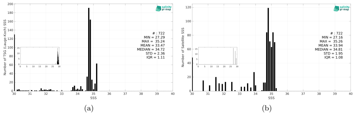
Figure 3: Histograms of SSS from TSG (Lauge-Koch) (a) and CCI SSS L4 Merged-OI v5.5 - 30-day running (ESA) (b) considering all match-up pairs per bins of 0.1 over the Arctic Ocean Pi-MEP region and for the full satellite product period.
