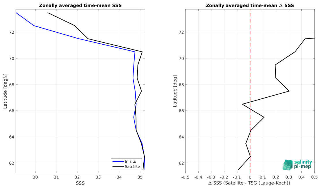
Figure 9: Left panel: Zonal mean SSS from CCI SSS L4 Merged-OI v5.5 - 30-day running (ESA) satellite product (black) and from TSG (Lauge-Koch) (blue). Right panel: Zonal mean of \Delta SSS (Satellite - TSG (Lauge-Koch)) for all the collected Pi-MEP match-up pairs estimated over the full satellite product period.
