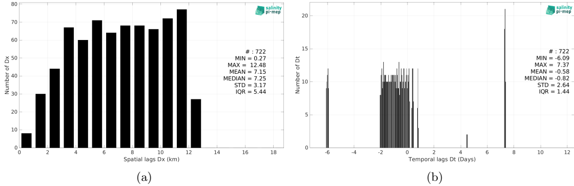
Figure 6: Histograms of the spatial (a) and temporal (b) lags between the location/time of the TSG (Lauge-Koch) measurement and the date of the corresponding CCI SSS L4 Merged-OI v5.5 - 30-day running (ESA) SSS pixel.
