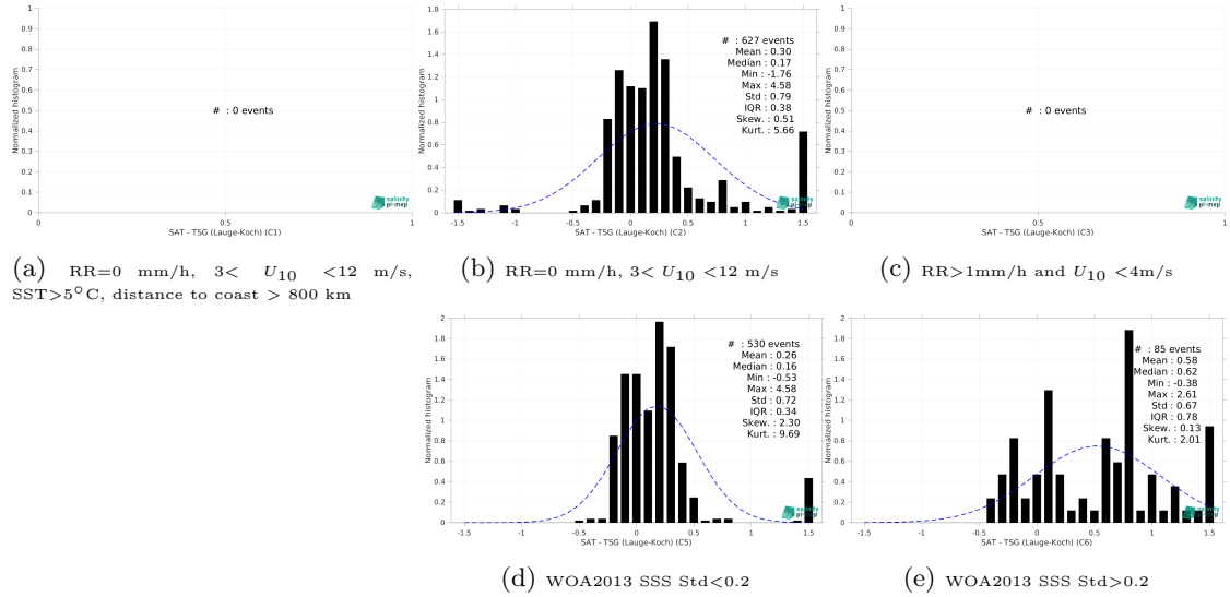
Figure 15: Normalized histogram of \Delta SSS (CCI SSS L4 Merged-OI v5.5 - 30-day running (ESA) - TSG (Lauge-Koch)) for 5 different subdatasets corresponding to: RR=0 mm/h, 3 < U_{10} < 12 m/s, SST>5°C, distance to coast > 800 km (a), RR=0 mm/h, 3 < U_{10} < 12 m/s (b), RR>1mm/h and U_{10} < 4 m/s (c), WOA2013 SSS Std<0.2 (d), WOA2013 SSS Std>0.2 (e).
