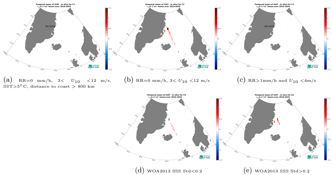
Figure 14: Temporal mean gridded over spatial boxes of size 1^\circ \times 1^\circ of \Delta SSS (CCI SSS L4 Merged-OI v5.5 - 30-day running (ESA) - TSG (Lauge-Koch)) for 5 different subdatasets corresponding to:RR=0 mm/h, 3 < U_{10} < 12 m/s, SST > 5^\circ C, distance to coast > 800 km (a), RR=0 mm/h, 3 < U_{10} < 12 m/s (b), RR > 1 mm/h and U_{10} < 4 m/s (c), WOA2013 SSS Std < 0.2 (d), WOA2013 SSS Std > 0.2 (e).
