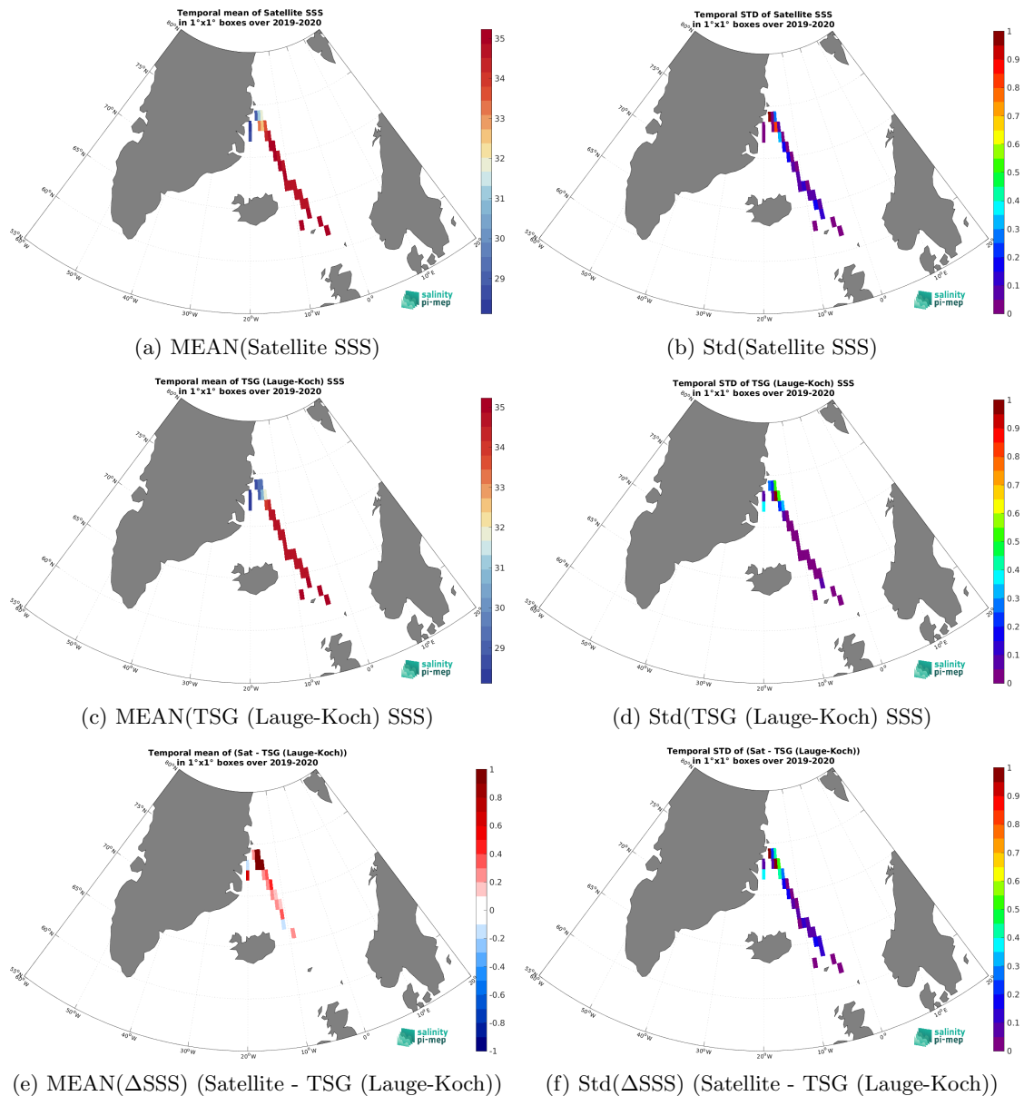
Figure 7: Temporal mean (left) and Std (right) of SSS from CCI SSS L4 Merged-OI v5.5 - 30-day running (ESA) (top), TSG (Lauge-Koch) (middle), and of \Delta SSS (Satellite - TSG (Lauge-Koch)). Only match-up pairs are used to generate these maps.
