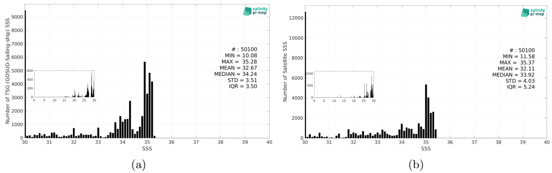
Figure 3: Histograms of SSS from TSG (GOSUD-Sailing-ship) (a) and CCI SSS L4 Merged-OI v5.5 - 30-day running (ESA) (b) considering all match-up pairs per bins of 0.1 over the Arctic Ocean Pi-MEP region and for the full satellite product period.
