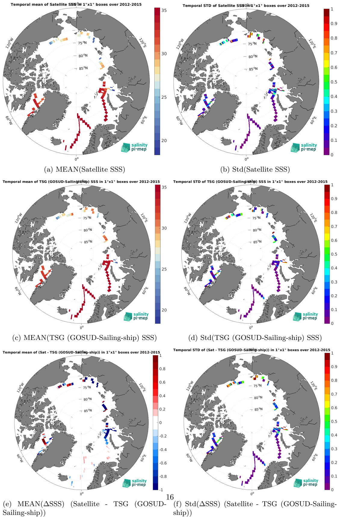
Figure 7: Temporal mean (left) and Std (right) of SSS from CCI SSS L4 Merged-OI v5.5 - 30-day running (ESA) (top), TSG (GOSUD-Sailing-ship) (middle), and of \Delta SSS (Satellite - TSG (GOSUD-Sailing-ship)). Only match-up pairs are used to generate these maps.
