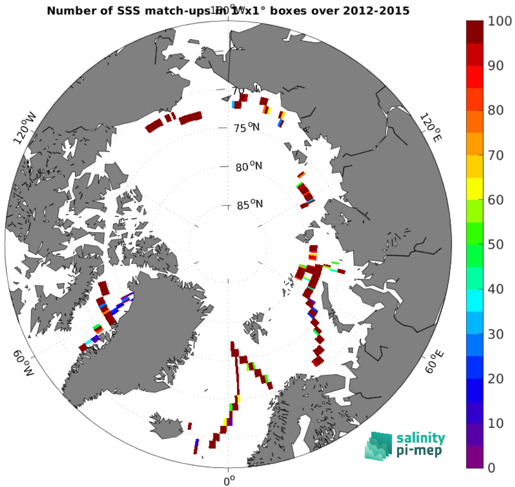
Figure 5: Number of SSS match-ups between TSG (GOSUD-Sailing-ship) SSS and the CCI SSS L4 Merged-OI v5.5 - 30-day running (ESA) SSS product for the Arctic Ocean Pi-MEP region over 1^{\circ} \times 1^{\circ} boxes and for the full satellite product period.
