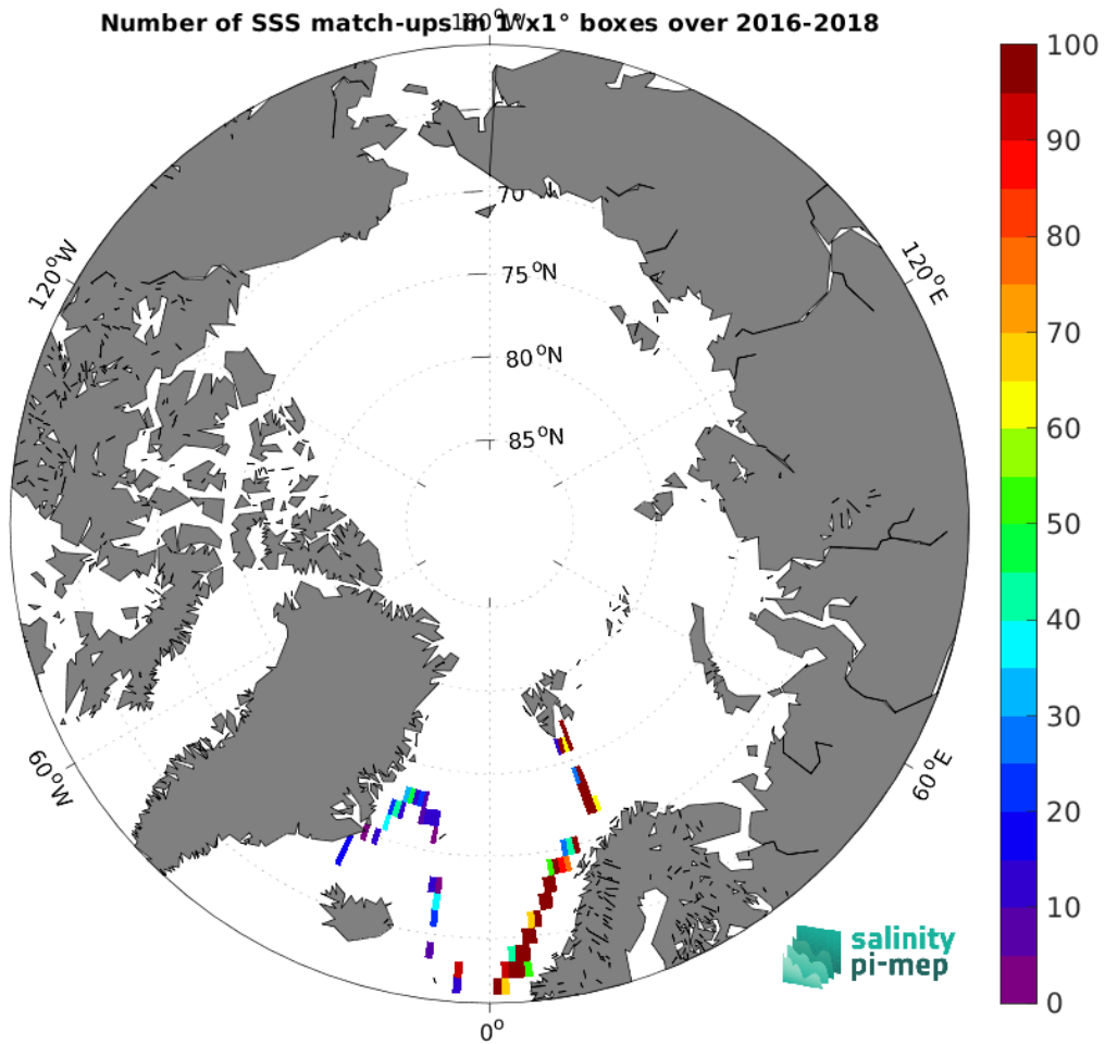
Figure 5: Number of SSS match-ups between TSG (GOSUD-Research-vessel) SSS and the CCI SSS L4 Merged-OI v5.5 - 30-day running (ESA) SSS product for the Arctic Ocean Pi-MEP region over 1^\circ \times 1^\circ boxes and for the full satellite product period.
