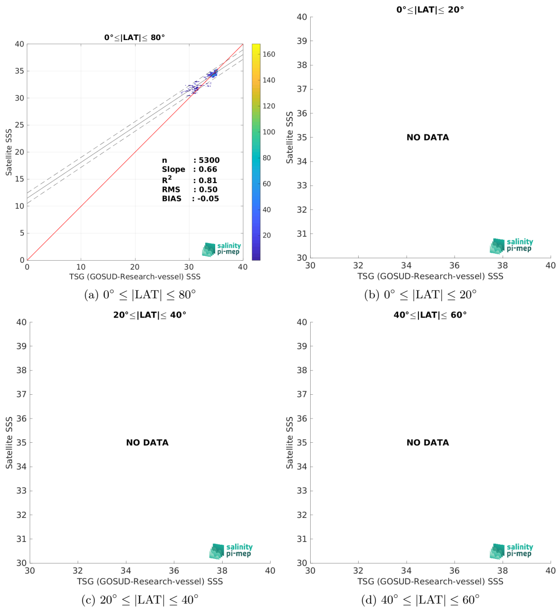
Figure 10: Contour maps of the concentration of CCI SSS L4 Merged-OI v5.5 - 30-day running (ESA) SSS (y-axis) versus TSG (GOSUD-Research-vessel) SSS (x-axis) at match-up pairs for different latitude bands. For each plot, the red line shows x=y . The black thin and dashed lines indicate a linear fit through the data cloud and the \pm 95\% confidence levels, respectively. The number match-up pairs n , the slope and R^2 coefficient of the linear fit, the root mean square (RMS) and the mean bias between satellite and in situ data are indicated for each latitude band in each plots.
