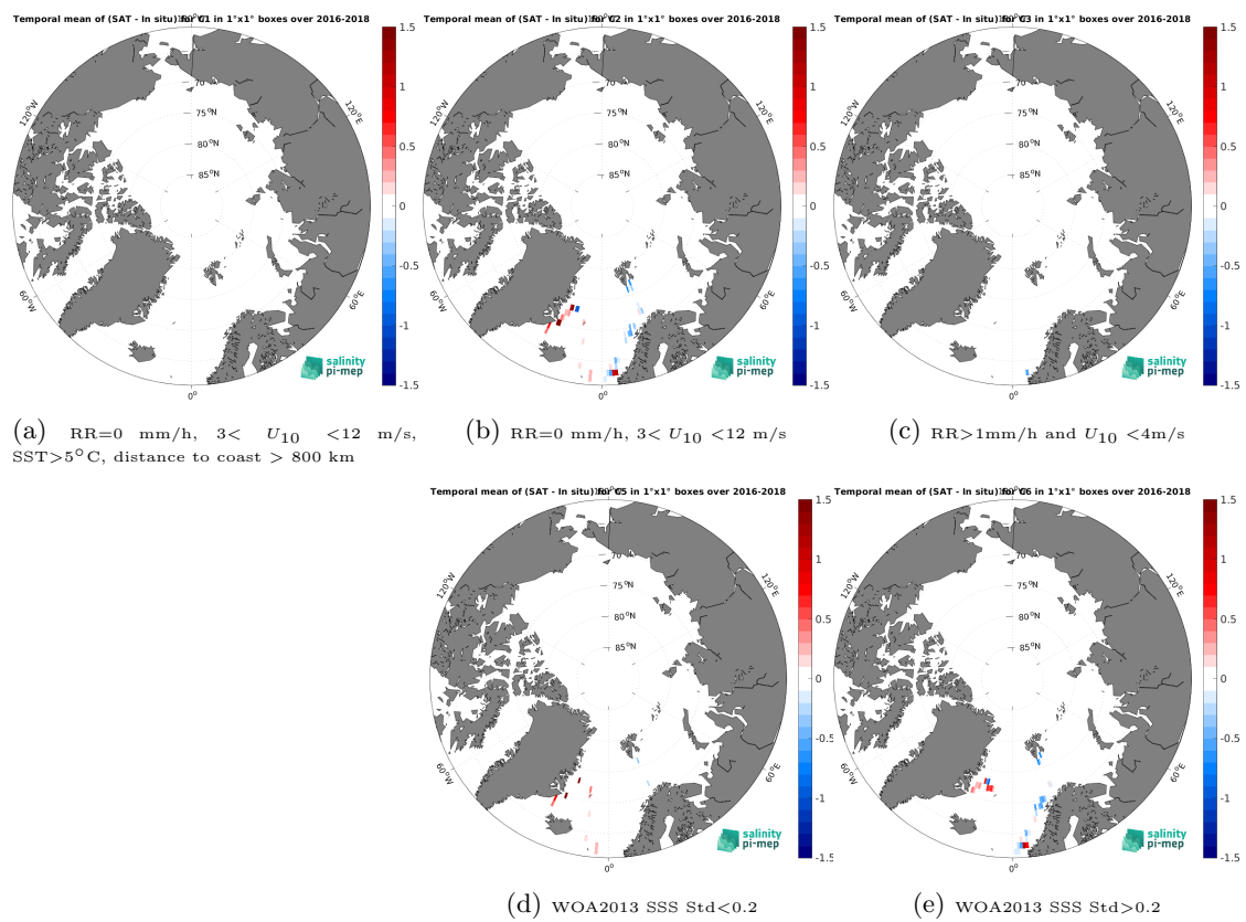
Figure 14: Temporal mean gridded over spatial boxes of size 1^\circ \times 1^\circ of \Delta\text{SSS} (CCI SSS L4 Merged-OI v5.5 - 30-day running (ESA) - TSG (GOSUD-Research-vessel)) for 5 different subdatasets corresponding to: RR=0 mm/h, 3 < U_{10} < 12 m/s, SST > 5°C, distance to coast > 800 km (a), RR=0 mm/h, 3 < U_{10} < 12 m/s (b), RR > 1mm/h and U_{10} < 4 m/s (c), WOA2013 SSS Std < 0.2 (d), WOA2013 SSS Std > 0.2 (e).
