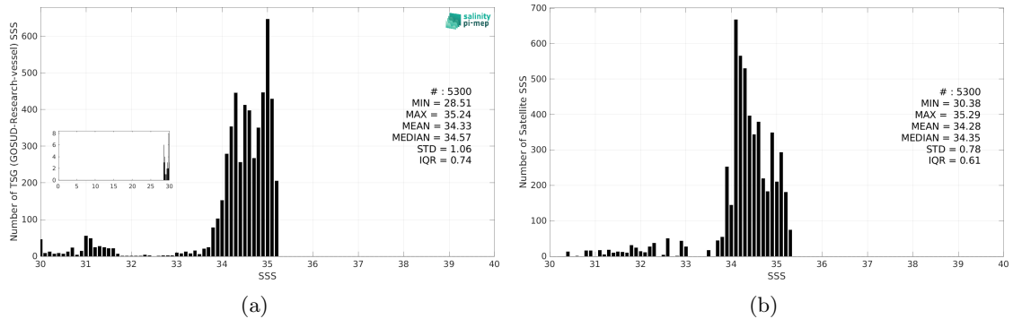
Figure 3: Histograms of SSS from TSG (GOSUD-Research-vessel) (a) and CCI SSS L4 Merged-OI v5.5 - 30-day running (ESA) (b) considering all match-up pairs per bins of 0.1 over the Arctic Ocean Pi-MEP region and for the full satellite product period.
