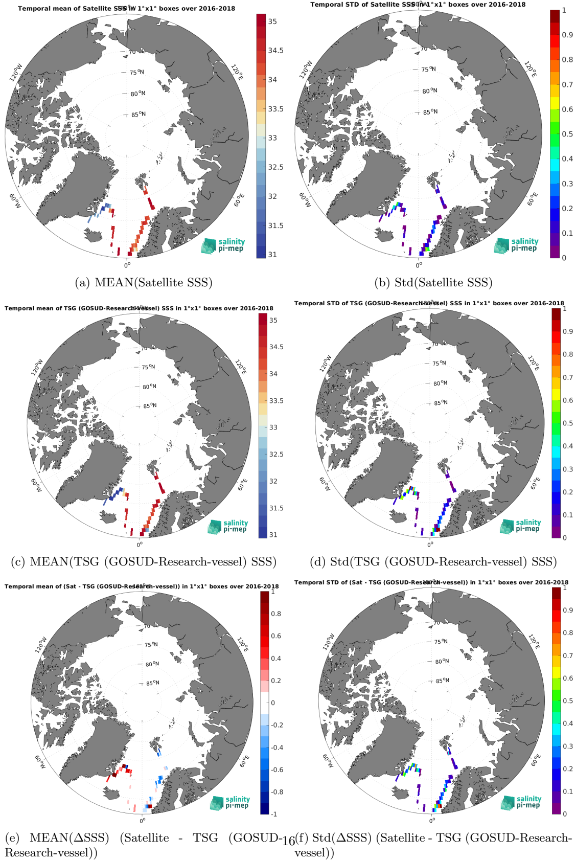
Figure 7: Temporal mean (left) and Std (right) of SSS from CCI SSS L4 Merged-OI v5.5 - 30-day running (ESA) (top), TSG (GOSUD-Research-vessel) (middle), and of \Delta SSS (Satellite - TSG (GOSUD-Research-vessel)). Only match-up pairs are used to generate these maps.
