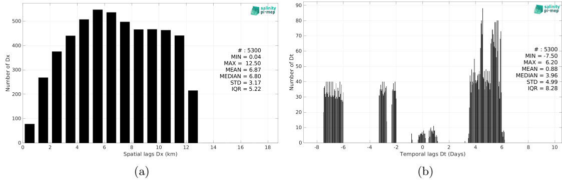
Figure 6: Histograms of the spatial (a) and temporal (b) lags between the location/time of the TSG (GOSUD-Research-vessel) measurement and the date of the corresponding CCI SSS L4 Merged-OI v5.5 - 30-day running (ESA) SSS pixel.
