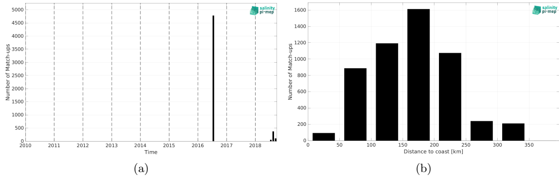
Figure 2: Number of match-ups between TSG (GOSUD-Research-vessel) and CCI SSS L4 Merged-OI v5.5 - 30-day running (ESA) SSS as a function of time (a) and as function of the distance to coast (b) over the Arctic Ocean Pi-MEP region and for the full satellite product period.
