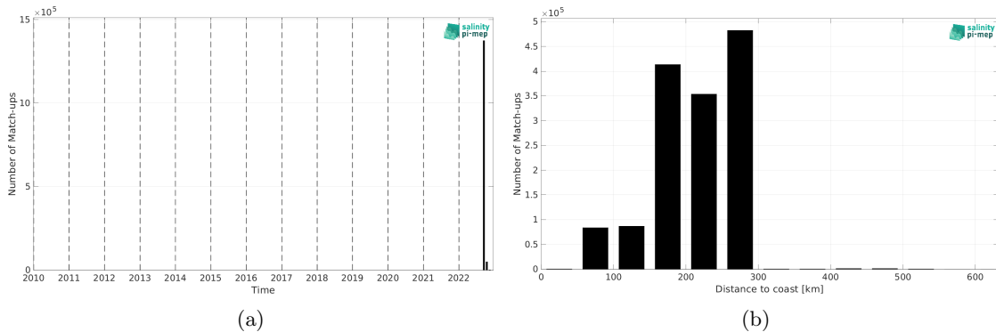
Figure 2: Number of match-ups between SASSIE and CCI SSS L4 Merged-OI v5.5 - 30-day running (ESA) SSS as a function of time (a) and as function of the distance to coast (b) over the Arctic Ocean Pi-MEP region and for the full satellite product period.
