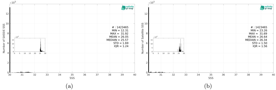
Figure 3: Histograms of SSS from SASSIE (a) and CCI SSS L4 Merged-OI v5.5 - 30-day running (ESA) (b) considering all match-up pairs per bins of 0.1 over the Arctic Ocean Pi-MEP region and for the full satellite product period.
