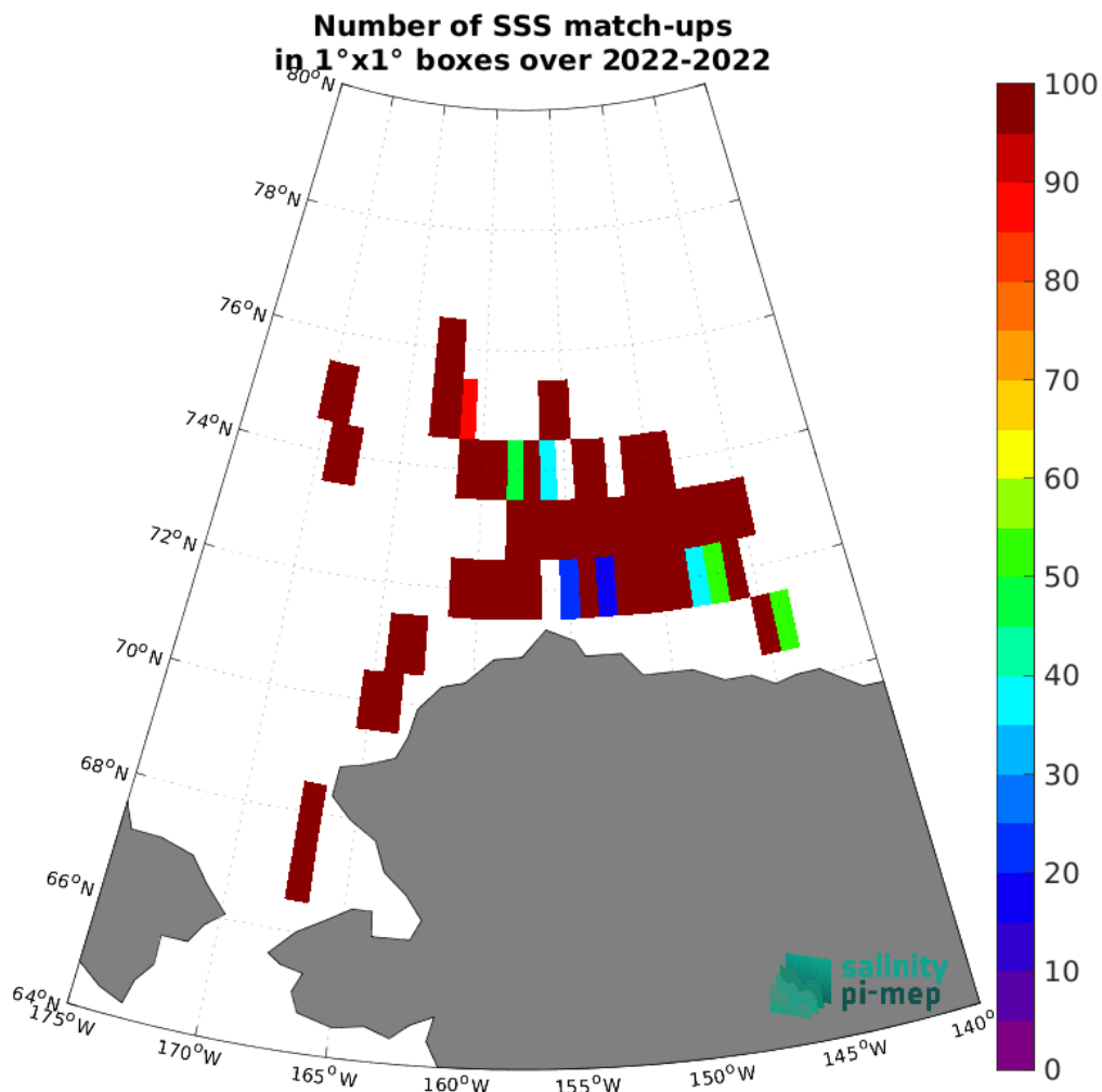
Figure 5: Number of SSS match-ups between SASSIE SSS and the CCI SSS L4 Merged-OI v5.5 - 30-day running (ESA) SSS product for the Arctic Ocean Pi-MEP region over 1^\circ \times 1^\circ boxes and for the full satellite product period.
