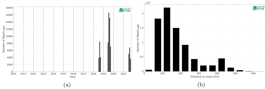
Figure 2: Number of match-ups between Saildrone and CCI SSS L4 Merged-OI v5.5 - 30-day running (ESA) SSS as a function of time (a) and as function of the distance to coast (b) over the Arctic Ocean Pi-MEP region and for the full satellite product period.
