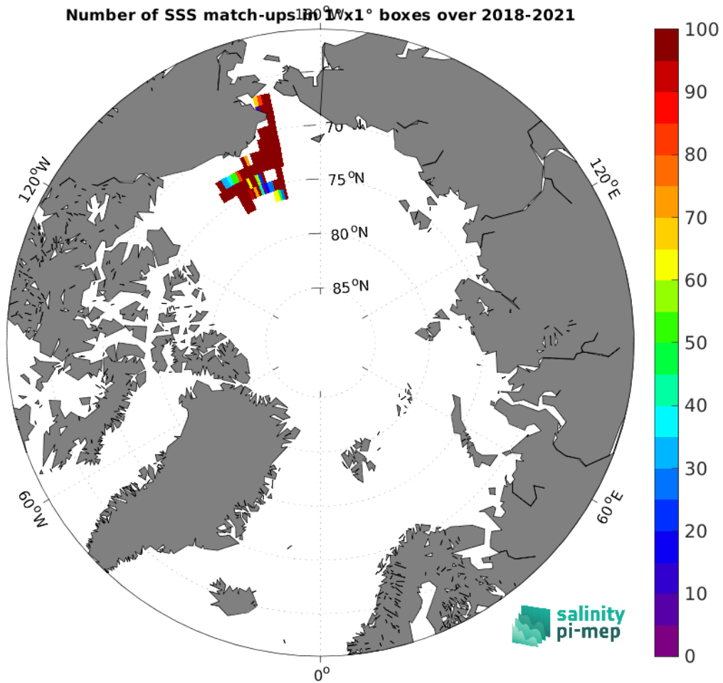
Figure 5: Number of SSS match-ups between Saildrone SSS and the CCI SSS L4 Merged-OI v5.5 - 30-day running (ESA) SSS product for the Arctic Ocean Pi-MEP region over 1^\circ \times 1^\circ boxes and for the full satellite product period.
