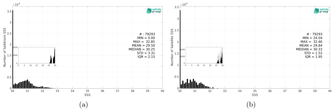
Figure 3: Histograms of SSS from Saildrone (a) and CCI SSS L4 Merged-OI v5.5 - 30-day running (ESA) (b) considering all match-up pairs per bins of 0.1 over the Arctic Ocean Pi-MEP region and for the full satellite product period.
