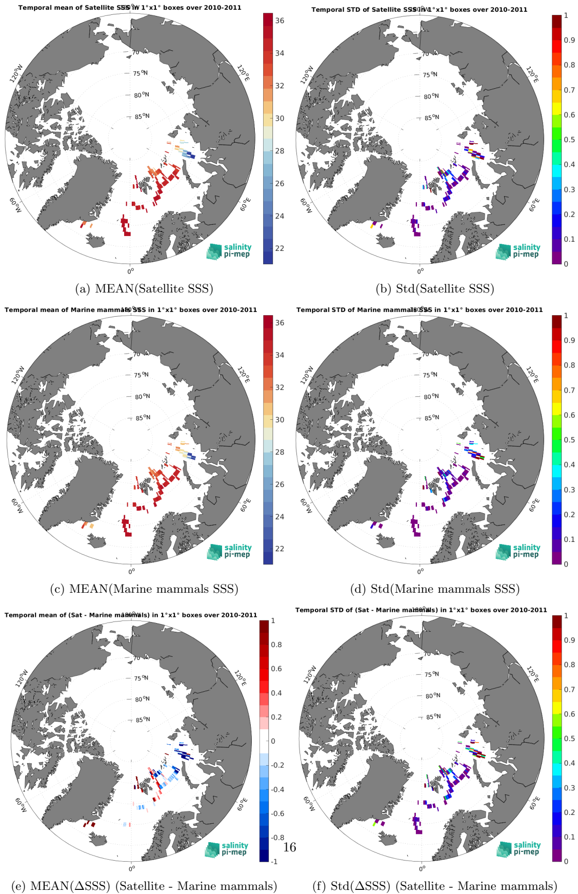
Figure 7: Temporal mean (left) and Std (right) of SSS from CCI SSS L4 Merged-OI v5.5 - 30-day running (ESA) (top), Marine mammals (middle), and of \Delta SSS (Satellite - Marine mammals). Only match-up pairs are used to generate these maps.
