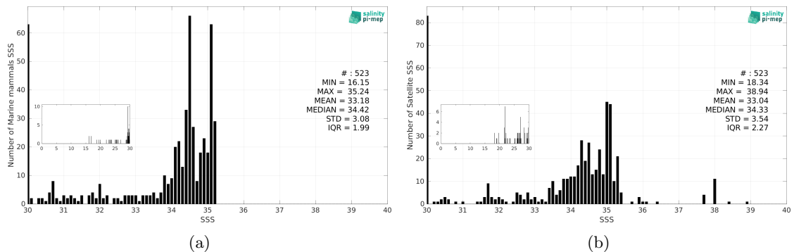
Figure 3: Histograms of SSS from Marine mammals (a) and CCI SSS L4 Merged-OI v5.5 - 30-day running (ESA) (b) considering all match-up pairs per bins of 0.1 over the Arctic Ocean Pi-MEP region and for the full satellite product period.
