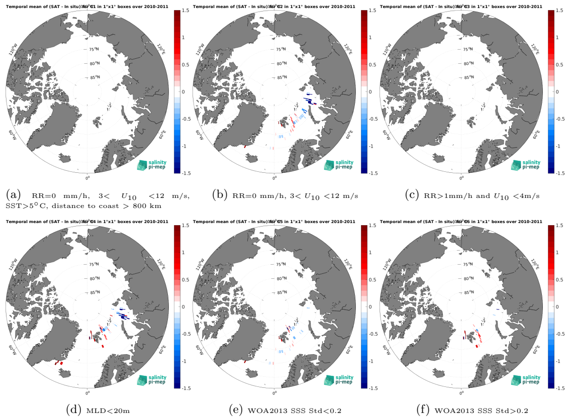
Figure 14: Temporal mean gridded over spatial boxes of size 1^\circ \times 1^\circ of \Delta\text{SSS} (CCI SSS L4 Merged-OI v5.5 - 30-day running (ESA) - Marine mammals) for 6 different subdatasets corresponding to:RR=0 mm/h, 3 < U_{10} < 12 m/s, SST>5°C, distance to coast > 800 km (a), RR=0 mm/h, 3 < U_{10} < 12 m/s (b), RR>1mm/h and U_{10} < 4 m/s (c),MLD<20m (d),WOA2013 SSS Std<0.2 (e),WOA2013 SSS Std>0.2 (f).
