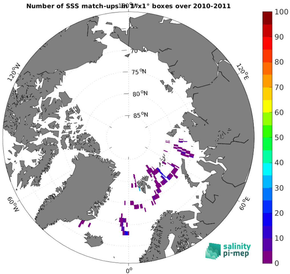
Figure 5: Number of SSS match-ups between Marine mammals SSS and the CCI SSS L4 Merged-OI v5.5 - 30-day running (ESA) SSS product for the Arctic Ocean Pi-MEP region over 1^\circ \times 1^\circ boxes and for the full satellite product period.
