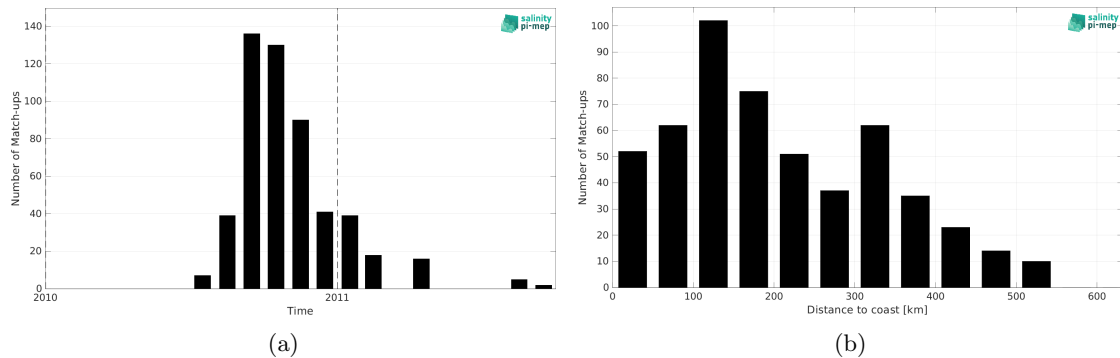
Figure 2: Number of match-ups between Marine mammals and CCI SSS L4 Merged-OI v5.5 - 30-day running (ESA) SSS as a function of time (a) and as function of the distance to coast (b) over the Arctic Ocean Pi-MEP region and for the full satellite product period.
