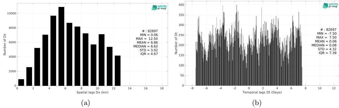
Figure 6: Histograms of the spatial (a) and temporal (b) lags between the location/time of the ICES measurement and the date of the corresponding CCI SSS L4 Merged-OI v5.5 - 30-day running (ESA) SSS pixel.
