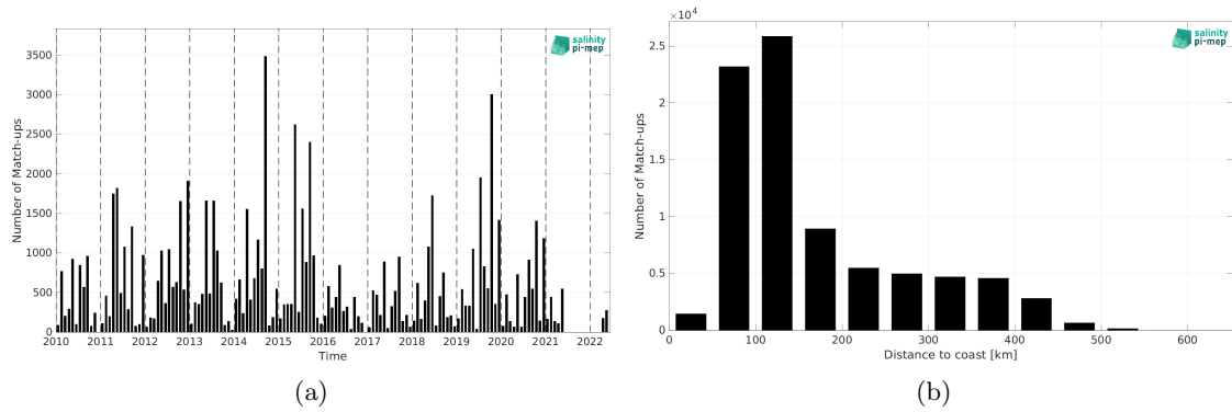
Figure 2: Number of match-ups between ICES and CCI SSS L4 Merged-OI v5.5 - 30-day running (ESA) SSS as a function of time (a) and as function of the distance to coast (b) over the Arctic Ocean Pi-MEP region and for the full satellite product period.
