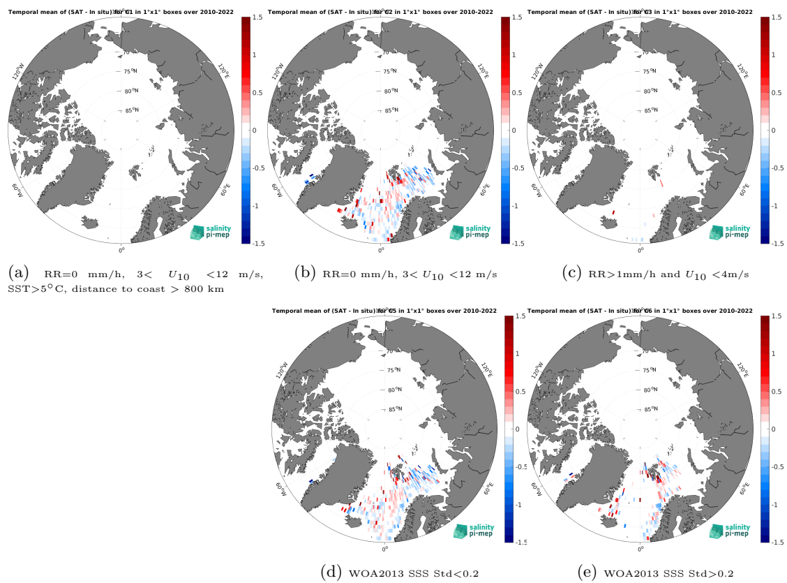
Figure 14: Temporal mean gridded over spatial boxes of size 1^\circ \times 1^\circ of \Delta\text{SSS} (CCI SSS L4 Merged-OI v5.5 - 30-day running (ESA) - ICES) for 5 different subdatasets corresponding to:RR=0 mm/h, 3 < U_{10} < 12 m/s, SST > 5^\circ\text{C} , distance to coast > 800 km (a), RR=0 mm/h, 3 < U_{10} < 12 m/s (b), RR > 1 mm/h and U_{10} < 4 m/s (c), WOA2013 SSS Std < 0.2 (d), WOA2013 SSS Std > 0.2 (e).
