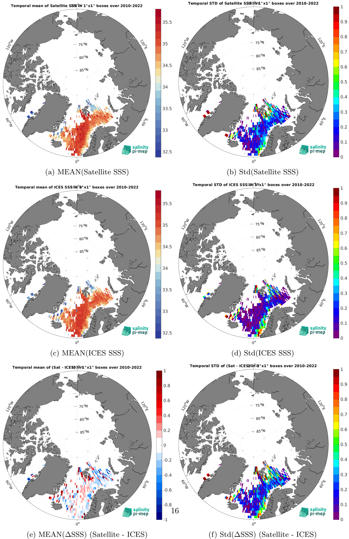
Figure 7: Temporal mean (left) and Std (right) of SSS from CCI SSS L4 Merged-OI v5.5 - 30-day running (ESA) (top), ICES (middle), and of \Delta SSS (Satellite - ICES). Only match-up pairs are used to generate these maps.
