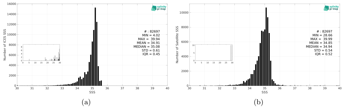
Figure 3: Histograms of SSS from ICES (a) and CCI SSS L4 Merged-OI v5.5 - 30-day running (ESA) (b) considering all match-up pairs per bins of 0.1 over the Arctic Ocean Pi-MEP region and for the full satellite product period.
