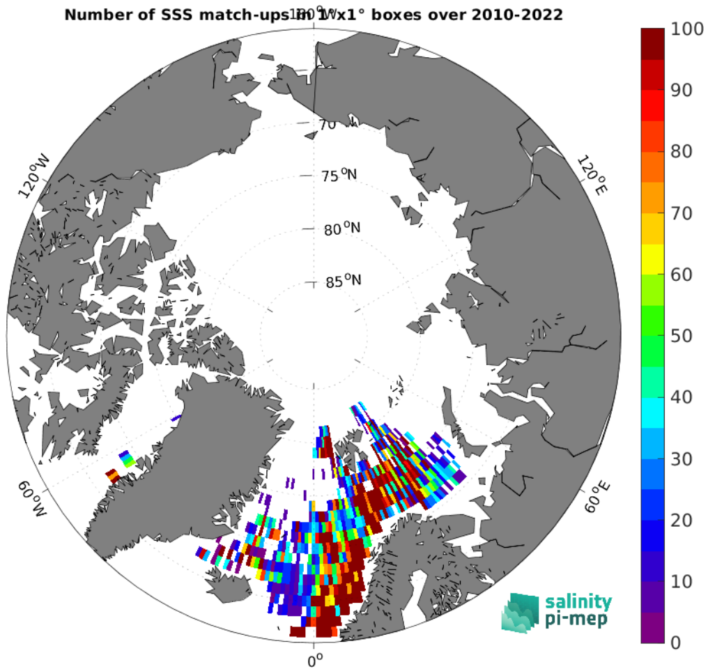
Figure 5: Number of SSS match-ups between ICES SSS and the CCI SSS L4 Merged-OI v5.5 - 30-day running (ESA) SSS product for the Arctic Ocean Pi-MEP region over 1^\circ \times 1^\circ boxes and for the full satellite product period.
