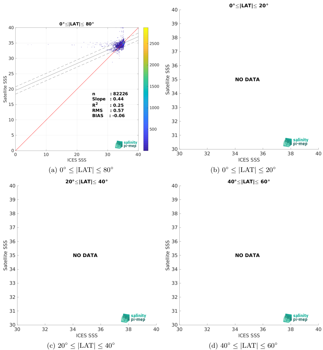
Figure 10: Contour maps of the concentration of CCI SSS L4 Merged-OI v5.5 - 30-day running (ESA) SSS (y-axis) versus ICES SSS (x-axis) at match-up pairs for different latitude bands. For each plot, the red line shows x=y . The black thin and dashed lines indicate a linear fit through the data cloud and the \pm 95\% confidence levels, respectively. The number match-up pairs n , the slope and R^2 coefficient of the linear fit, the root mean square (RMS) and the mean bias between satellite and in situ data are indicated for each latitude band in each plots.
