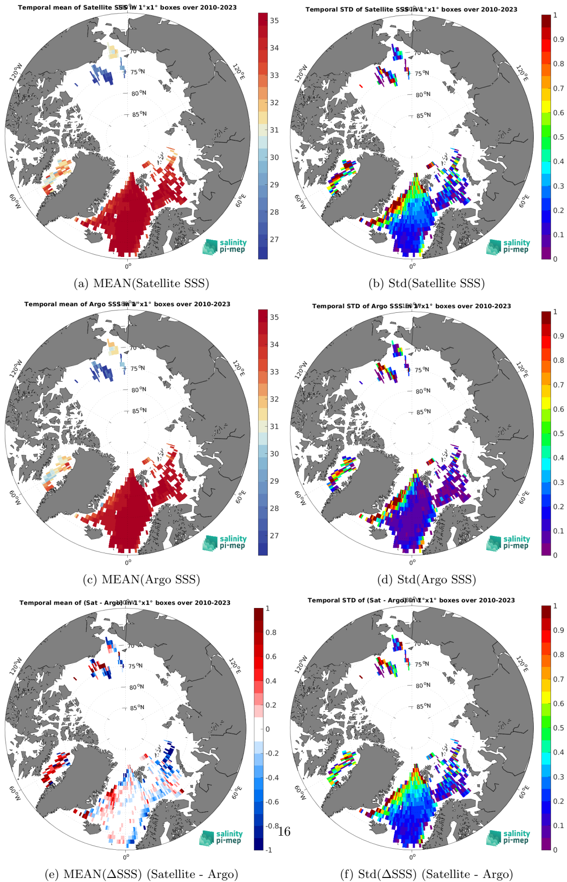
Figure 7: Temporal mean (left) and Std (right) of SSS from CCI SSS L4 Merged-OI v5.5 - 30-day running (ESA) (top), Argo (middle), and of \Delta SSS (Satellite - Argo). Only match-up pairs are used to generate these maps.
