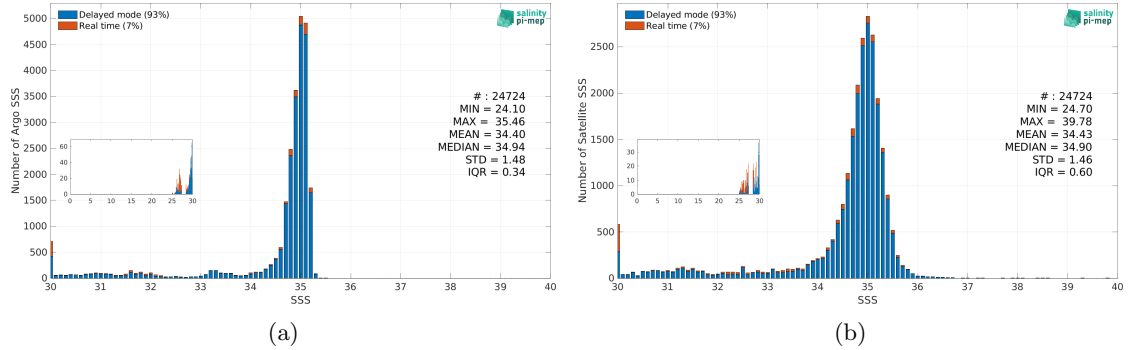
Figure 3: Histograms of SSS from Argo (a) and CCI SSS L4 Merged-OI v5.5 - 30-day running (ESA) (b) considering all match-up pairs per bins of 0.1 over the Arctic Ocean Pi-MEP region and for the full satellite product period.
