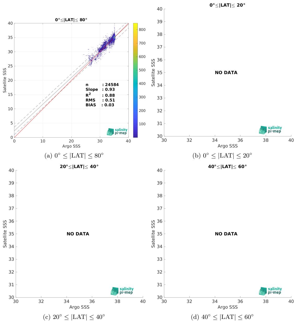
Figure 10: Contour maps of the concentration of CCI SSS L4 Merged-OI v5.5 - 30-day running (ESA) SSS (y-axis) versus Argo SSS (x-axis) at match-up pairs for different latitude bands. For each plot, the red line shows x=y . The black thin and dashed lines indicate a linear fit through the data cloud and the \pm 95\% confidence levels, respectively. The number match-up pairs n , the slope and R^2 coefficient of the linear fit, the root mean square (RMS) and the mean bias between satellite and in situ data are indicated for each latitude band in each plots.
