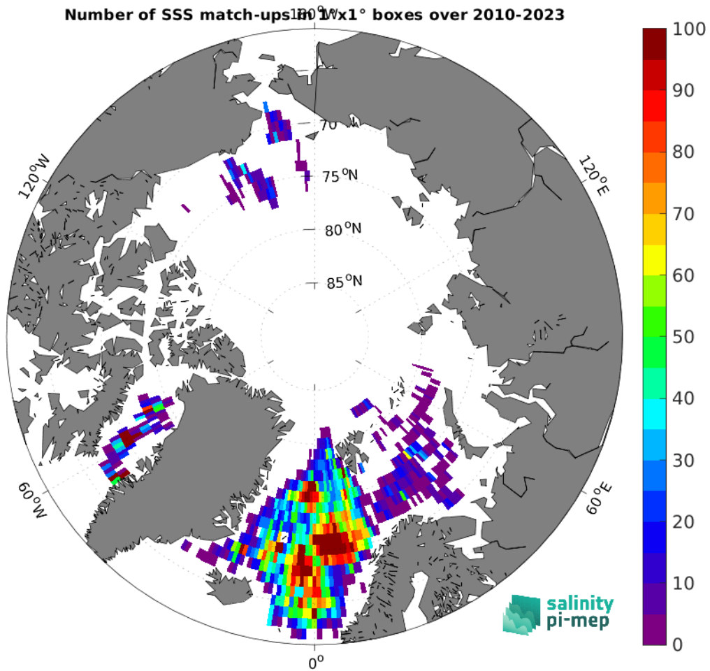
Figure 5: Number of SSS match-ups between Argo SSS and the CCI SSS L4 Merged-OI v5.5 - 30-day running (ESA) SSS product for the Arctic Ocean Pi-MEP region over 1^\circ \times 1^\circ boxes and for the full satellite product period.
