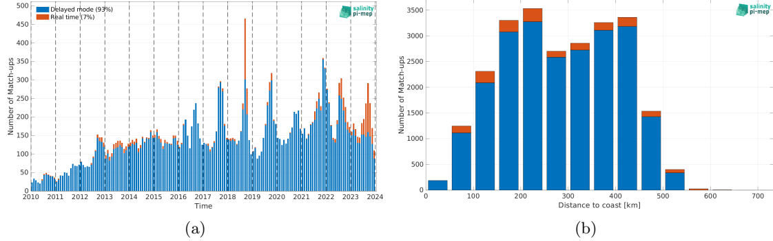
Figure 2: Number of match-ups between Argo and CCI SSS L4 Merged-OI v5.5 - 30-day running (ESA) SSS as a function of time (a) and as function of the distance to coast (b) over the Arctic Ocean Pi-MEP region and for the full satellite product period.
