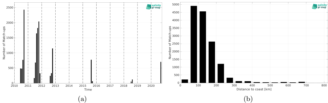
Figure 2: Number of match-ups between TSG (SAMOS) and CCI SSS L4 Merged-OI v4.41 - 7-day running (ESA) SSS as a function of time (a) and as function of the distance to coast (b) over the Arctic Ocean Pi-MEP region and for the full satellite product period.
