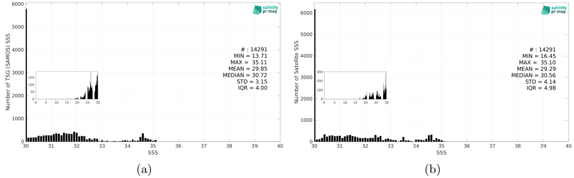
Figure 3: Histograms of SSS from TSG (SAMOS) (a) and CCI SSS L4 Merged-OI v4.41 - 7-day running (ESA) (b) considering all match-up pairs per bins of 0.1 over the Arctic Ocean Pi-MEP region and for the full satellite product period.
