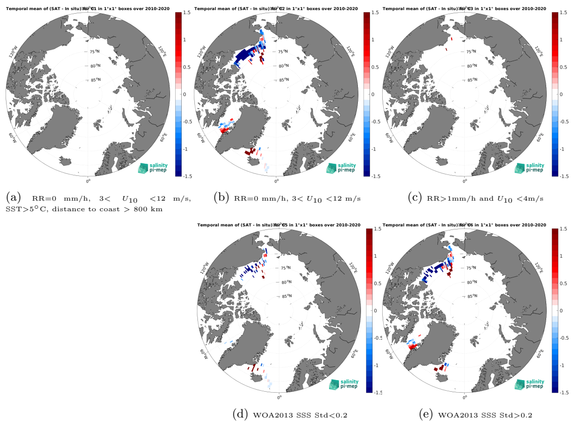
Figure 14: Temporal mean gridded over spatial boxes of size 1^\circ \times 1^\circ of \Delta\text{SSS} (CCI SSS L4 Merged-OI v4.41 - 7-day running (ESA) - TSG (SAMOS)) for 5 different subdatasets corresponding to:RR=0 mm/h, 3 < U_{10} < 12 m/s, SST>5°C, distance to coast > 800 km (a), RR=0 mm/h, 3 < U_{10} < 12 m/s (b), RR>1mm/h and U_{10} < 4 m/s (c), WOA2013 SSS Std<0.2 (d), WOA2013 SSS Std>0.2 (e).
