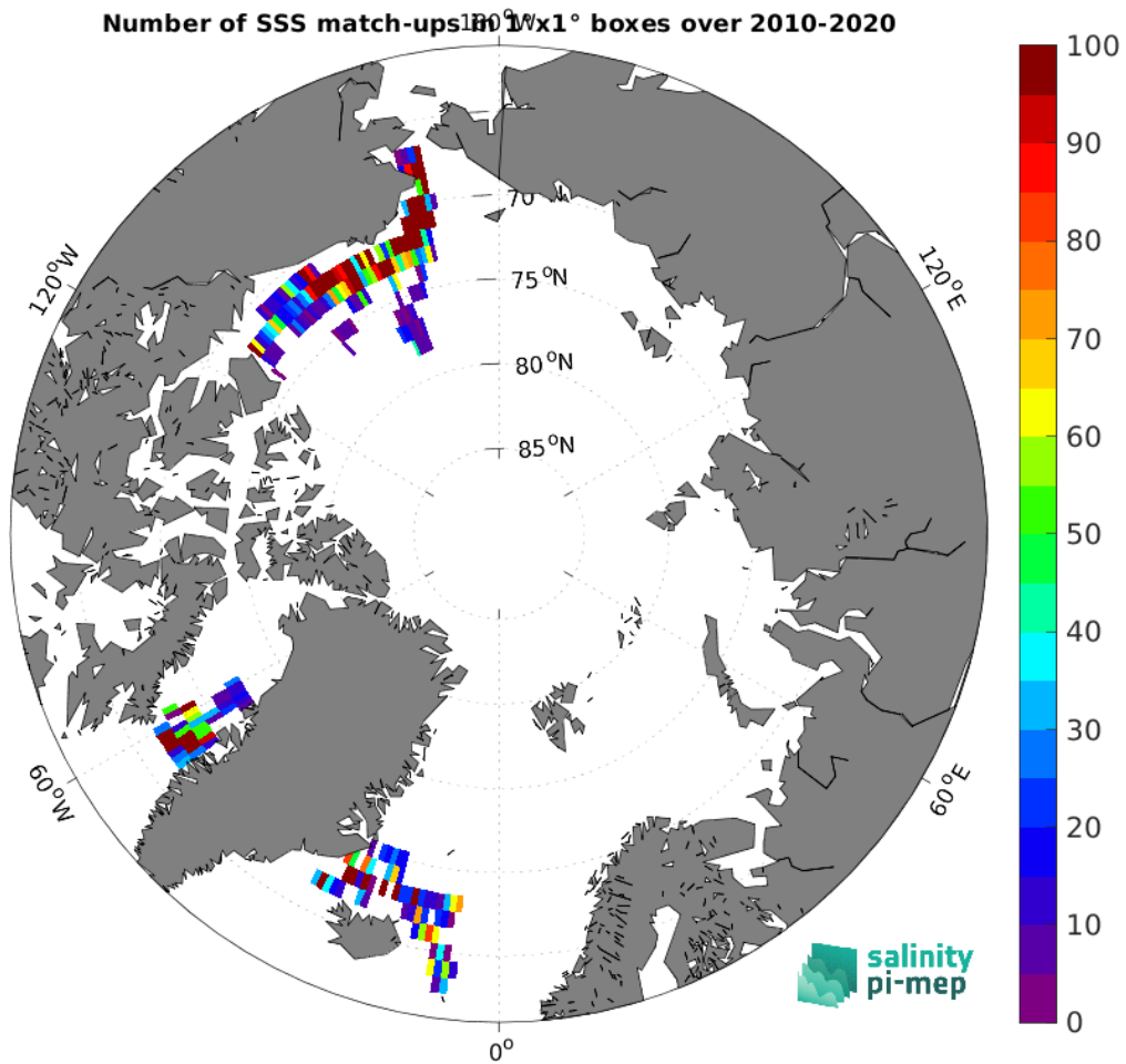
Figure 5: Number of SSS match-ups between TSG (SAMOS) SSS and the CCI SSS L4 Merged-OI v4.41 - 7-day running (ESA) SSS product for the Arctic Ocean Pi-MEP region over 1^\circ \times 1^\circ boxes and for the full satellite product period.
