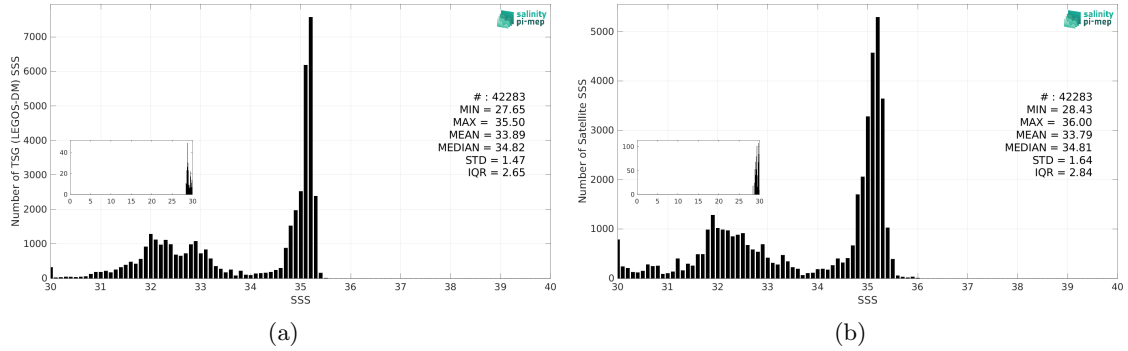
Figure 3: Histograms of SSS from TSG (LEGOS-DM) (a) and CCI SSS L4 Merged-OI v4.41 - 7-day running (ESA) (b) considering all match-up pairs per bins of 0.1 over the Arctic Ocean Pi-MEP region and for the full satellite product period.
