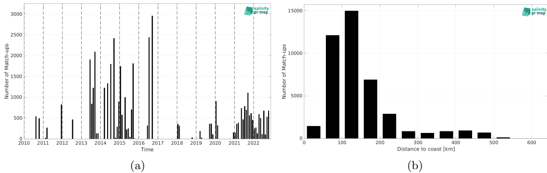
Figure 2: Number of match-ups between TSG (LEGOS-DM) and CCI SSS L4 Merged-OI v4.41 - 7-day running (ESA) SSS as a function of time (a) and as function of the distance to coast (b) over the Arctic Ocean Pi-MEP region and for the full satellite product period.
