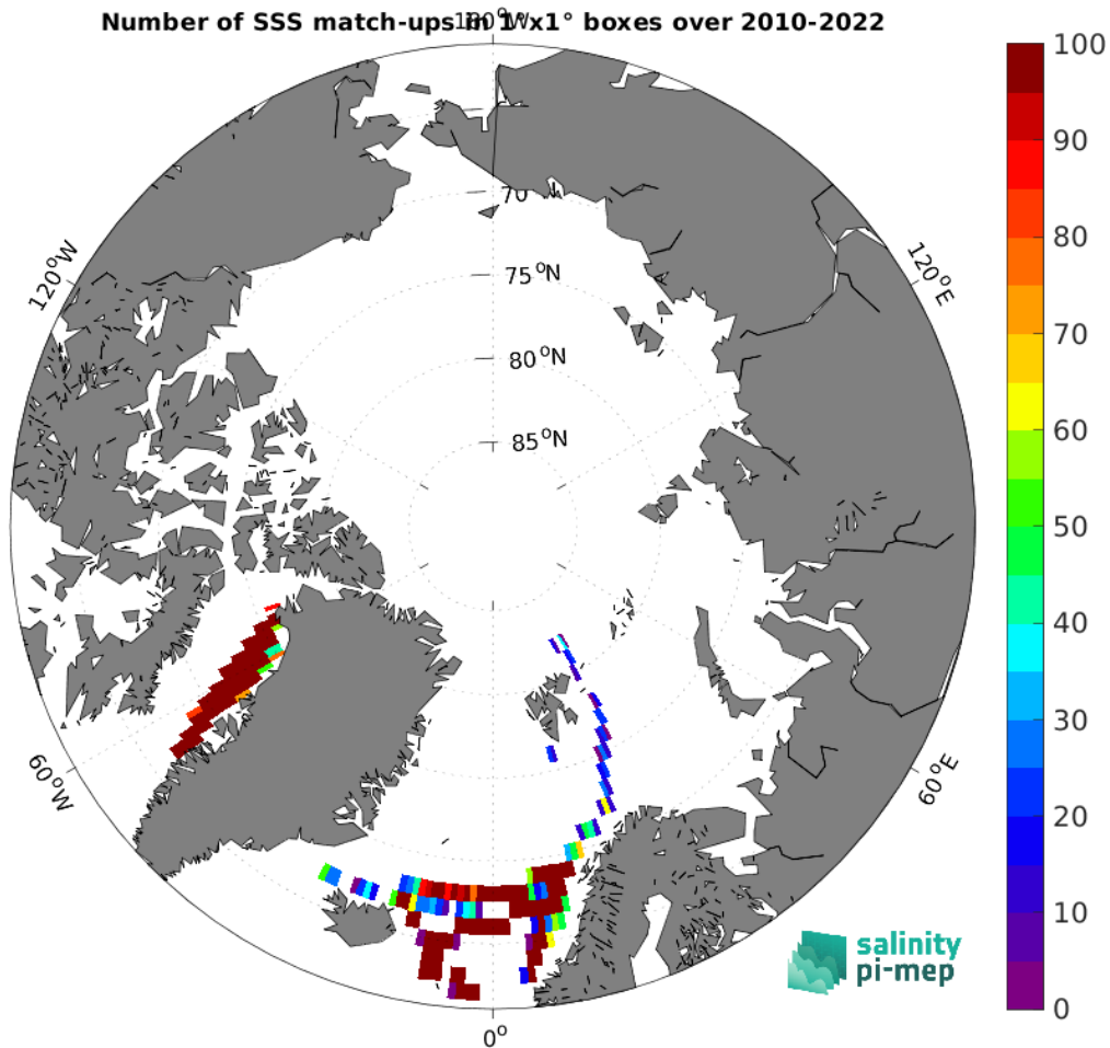
Figure 5: Number of SSS match-ups between TSG (LEGOS-DM) SSS and the CCI SSS L4 Merged-OI v4.41 - 7-day running (ESA) SSS product for the Arctic Ocean Pi-MEP region over 1^\circ \times 1^\circ boxes and for the full satellite product period.
