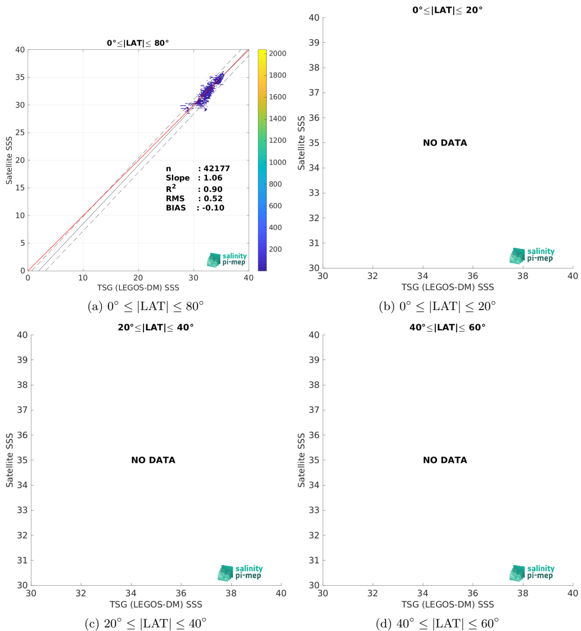
Figure 10: Contour maps of the concentration of CCI SSS L4 Merged-OI v4.41 - 7-day running (ESA) SSS (y-axis) versus TSG (LEGOS-DM) SSS (x-axis) at match-up pairs for different latitude bands. For each plot, the red line shows x=y . The black thin and dashed lines indicate a linear fit through the data cloud and the \pm 95\% confidence levels, respectively. The number match-up pairs n , the slope and R^2 coefficient of the linear fit, the root mean square (RMS) and the mean bias between satellite and in situ data are indicated for each latitude band in each plots.
