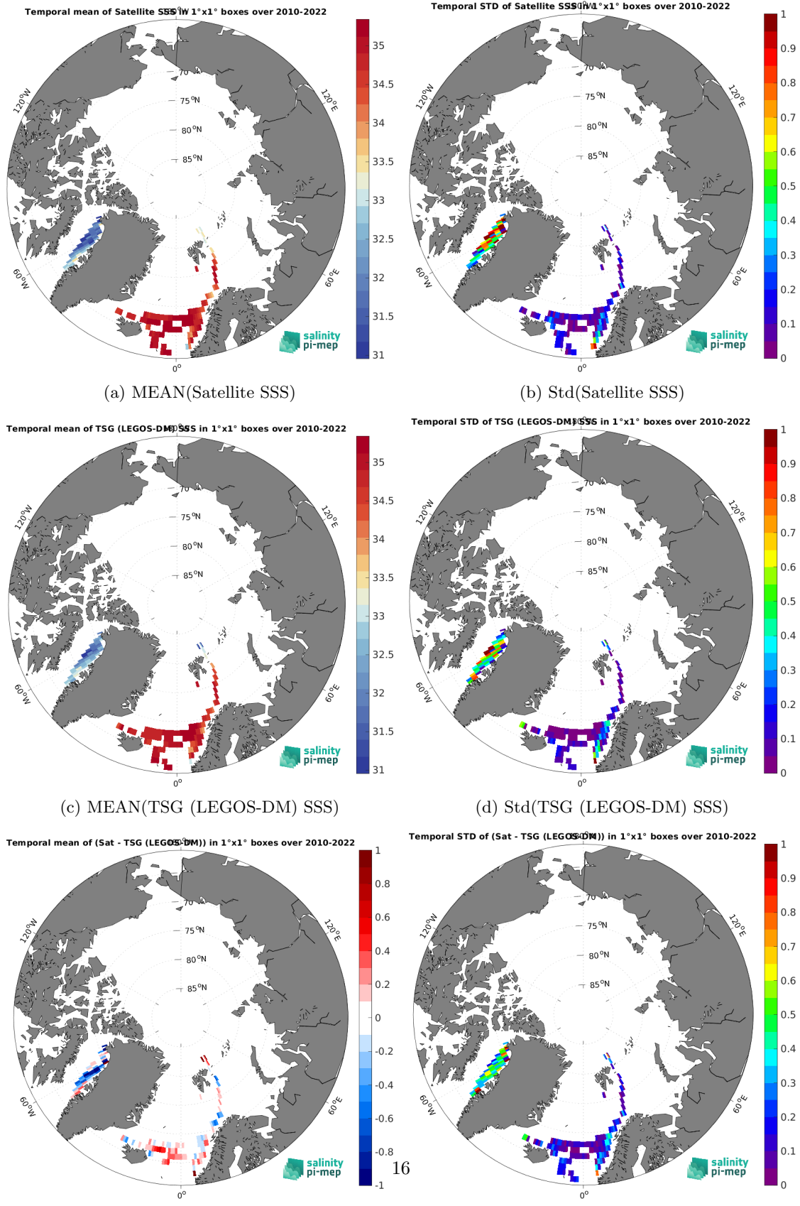
(e) MEAN( \Delta SSS) (Satellite - TSG (LEGOS-DM)) (f) Std( \Delta SSS) (Satellite - TSG (LEGOS-DM)) Figure 7: Temporal mean (left) and Std (right) of SSS from CCI SSS L4 Merged-OI v4.41 - 7-day running (ESA) (top), TSG (LEGOS-DM) (middle), and of \Delta SSS (Satellite - TSG (LEGOS-DM)). Only match-up pairs are used to generate these maps.
