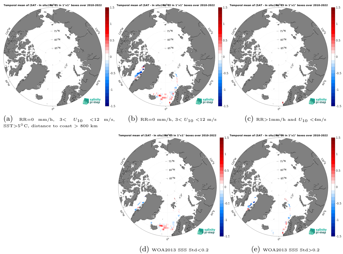
Figure 14: Temporal mean gridded over spatial boxes of size 1^\circ \times 1^\circ of \Delta SSS (CCI SSS L4 Merged-OI v4.41 - 7-day running (ESA) - TSG (LEGOS-DM)) for 5 different subdatasets corresponding to: RR=0 mm/h, 3 < U_{10} < 12 m/s, SST > 5^\circ\text{C} , distance to coast > 800 km (a), RR=0 mm/h, 3 < U_{10} < 12 m/s (b), RR > 1 mm/h and U_{10} < 4 m/s (c), WOA2013 SSS Std < 0.2 (d), WOA2013 SSS Std > 0.2 (e).
