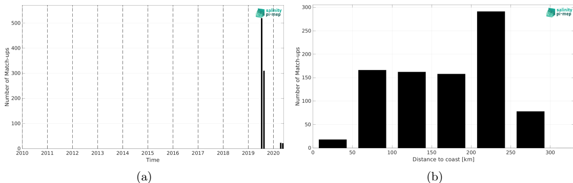
Figure 2: Number of match-ups between TSG (Lauge-Koch) and CCI SSS L4 Merged-OI v4.41 - 7-day running (ESA) SSS as a function of time (a) and as function of the distance to coast (b) over the Arctic Ocean Pi-MEP region and for the full satellite product period.
