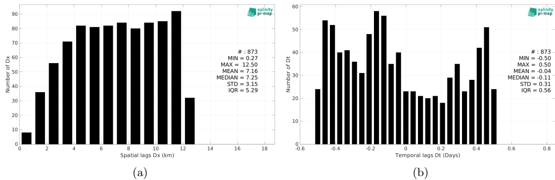
Figure 6: Histograms of the spatial (a) and temporal (b) lags between the location/time of the TSG (Lauge-Koch) measurement and the date of the corresponding CCI SSS L4 Merged-OI v4.41 - 7-day running (ESA) SSS pixel.
