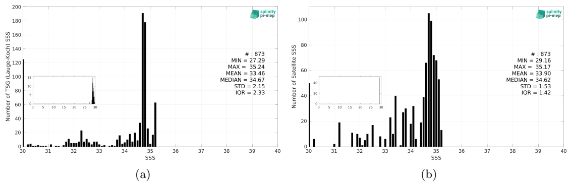
Figure 3: Histograms of SSS from TSG (Lauge-Koch) (a) and CCI SSS L4 Merged-OI v4.41 - 7-day running (ESA) (b) considering all match-up pairs per bins of 0.1 over the Arctic Ocean Pi-MEP region and for the full satellite product period.
