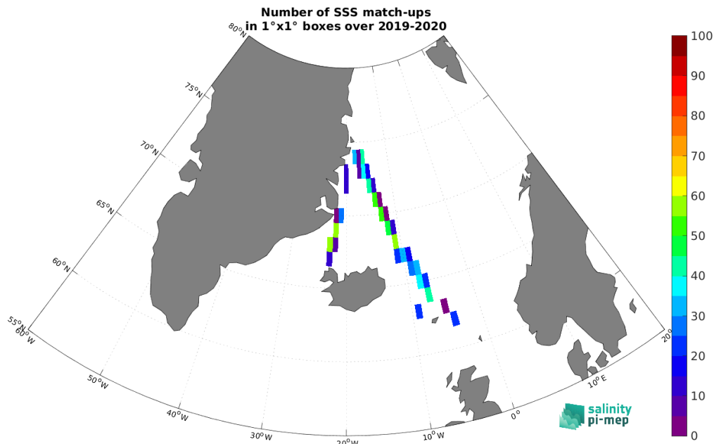
Figure 5: Number of SSS match-ups between TSG (Lauge-Koch) SSS and the CCI SSS L4 Merged-OI v4.41 - 7-day running (ESA) SSS product for the Arctic Ocean Pi-MEP region over 1^\circ \times 1^\circ boxes and for the full satellite product period.
