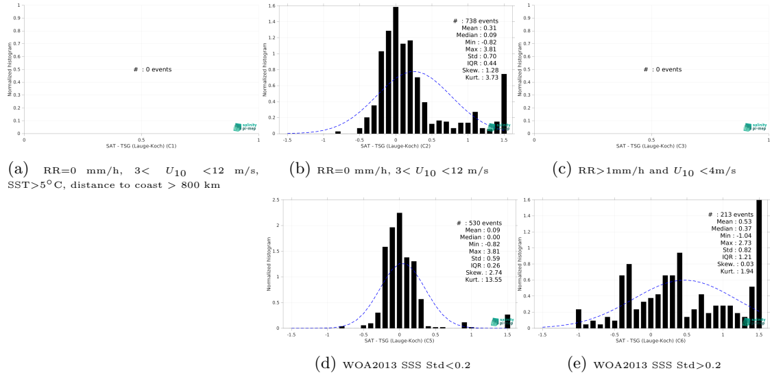
Figure 15: Normalized histogram of \Delta SSS (CCI SSS L4 Merged-OI v4.41 - 7-day running (ESA) - TSG (Lauge-Koch)) for 5 different subdatasets corresponding to: RR=0 mm/h, 3 < U_{10} < 12 m/s, SST>5°C, distance to coast > 800 km (a), RR=0 mm/h, 3 < U_{10} < 12 m/s (b), RR>1mm/h and U_{10} < 4 m/s (c), WOA2013 SSS Std<0.2 (d), WOA2013 SSS Std>0.2 (e).
